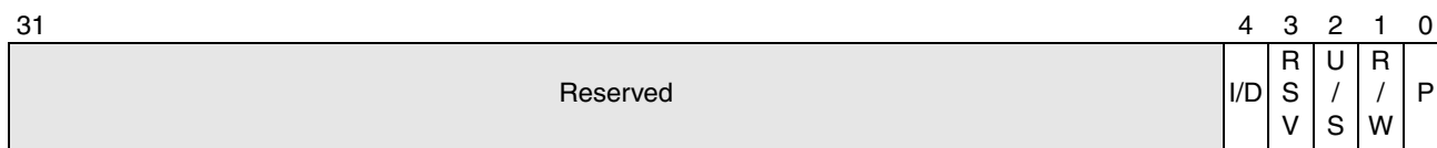
Figure 8-3. Page-Fault Error Code
