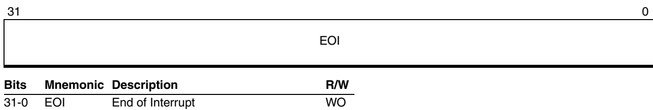
Figure 16-26. End of Interrupt - EOI (APIC Offset B0h)
