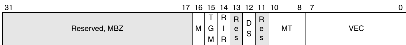
Figure 16-10. Local Interrupt 0/1 (LINT0/1) Local Vector Table Register (APIC Offset 350h/360h)
