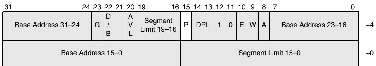
Figure 4-21. Data-Segment Descriptor—Long Mode
