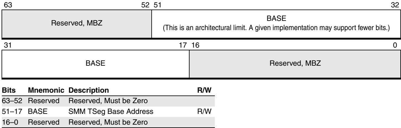
Figure 10-4. SSM_ADDR Register Format
