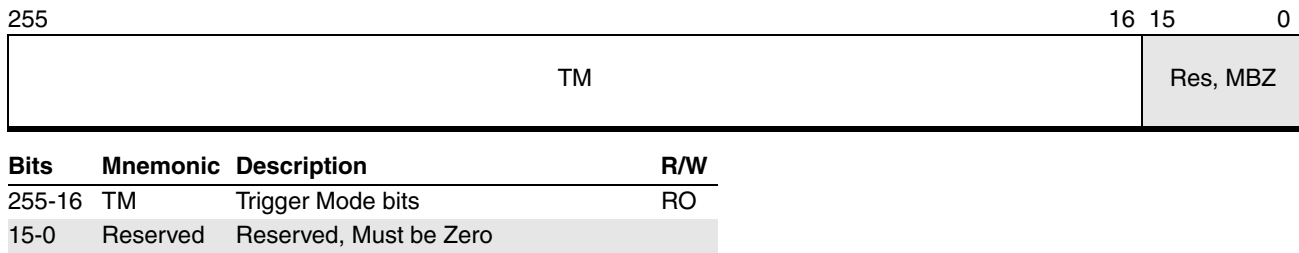
Figure 16-23. Trigger Mode Register - TMR (APIC Offset 1F0:180h)
