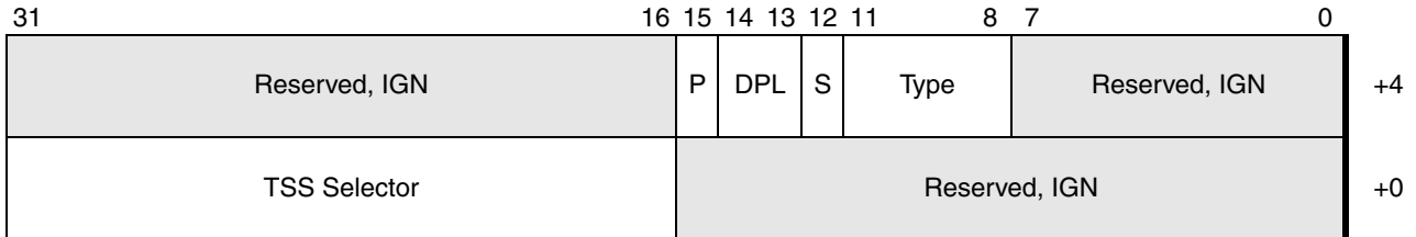
Figure 12-9. Task-Gate Descriptor, Legacy Mode Only
