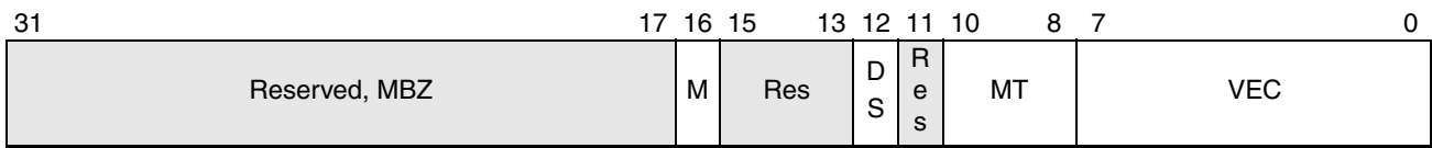
Figure 16-12. Thermal Sensor Local Vector Table Register (APIC Offset 330h)
