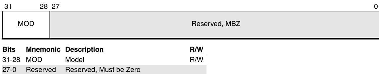
Figure 16-19. Destination Format Register (APIC Offset E0h)
