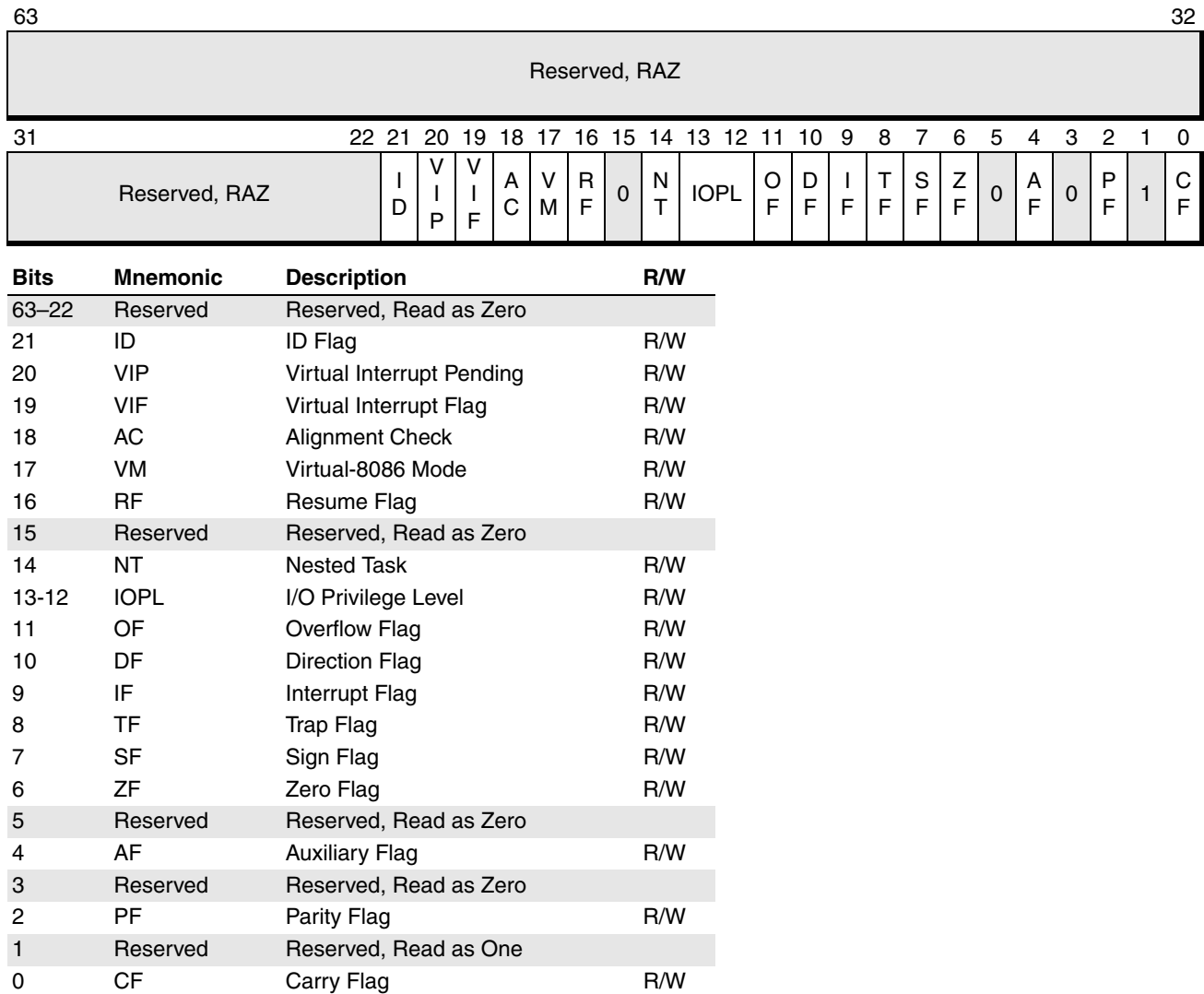
Figure 3-8. RFLAGS Register
