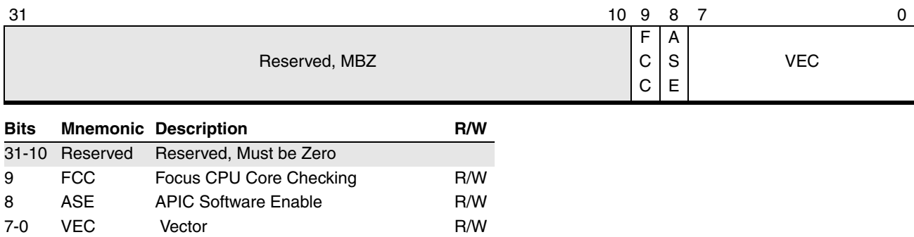
Figure 16-15. Spurious Interrupt Register (APIC Offset F0h)
