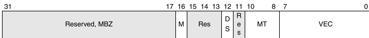
Figure 16-13. APIC Error Local Vector Table Register (APIC Offset 370h)
