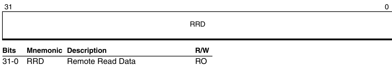
Figure 16-17. Remote Read Register (APIC Offset C0h)
