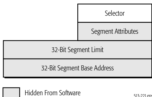
Figure 4-4. Segment-Register Format
