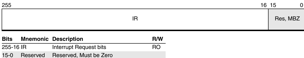
Figure 16-21. Interrupt Request Register - IRR (APIC Offset 270:200h)
