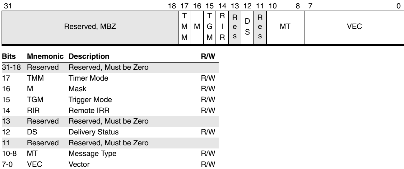
Figure 16-5. General Local Vector Table Register Format
