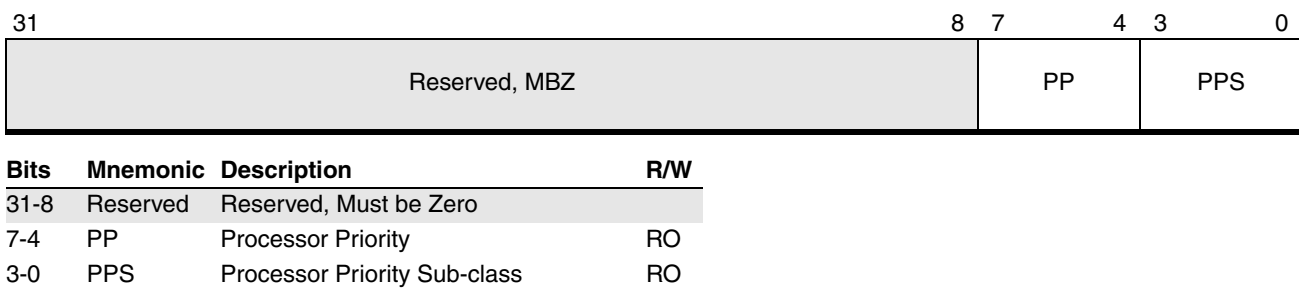
Figure 16-25. Processor Priority Register - PPR (APIC Offset A0h)
