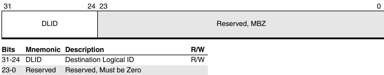
Figure 16-18. Logical Destination Register - LDR (APIC Offset D0h)
