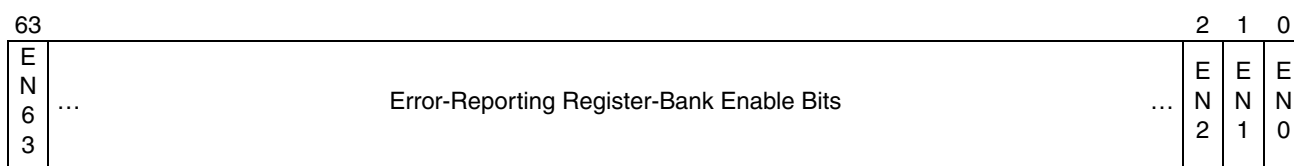
Figure 9-3. MCG_CTL Register
