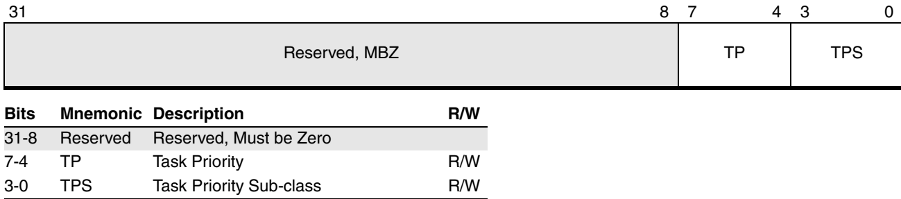
Figure 16-24. APIC 80 - Task Priority Register - TPR (APIC Offset 80h)
