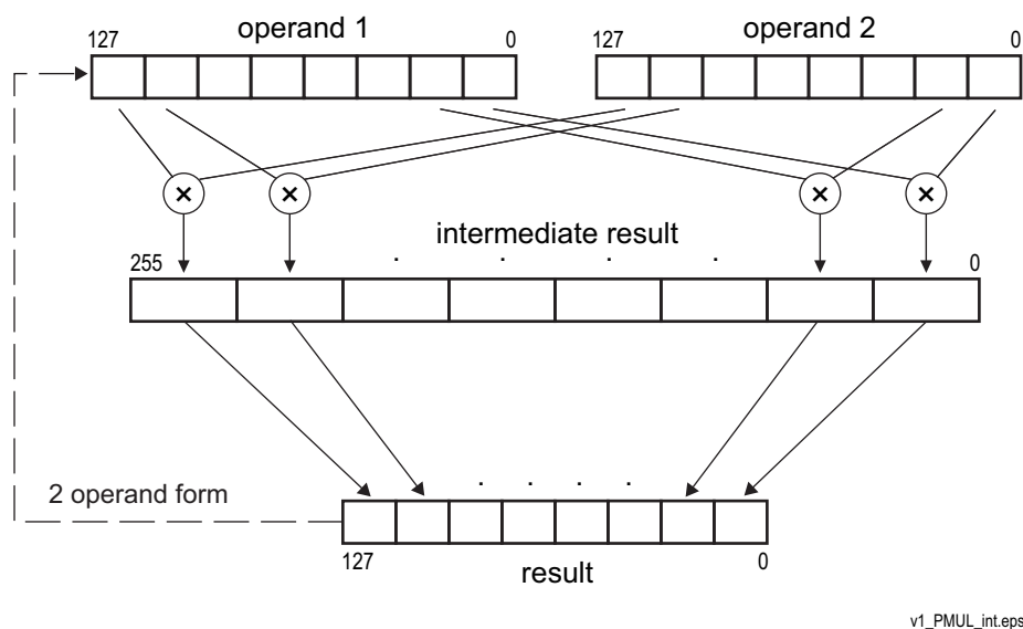
Figure 4-32. PMULxW Multiply Operation
