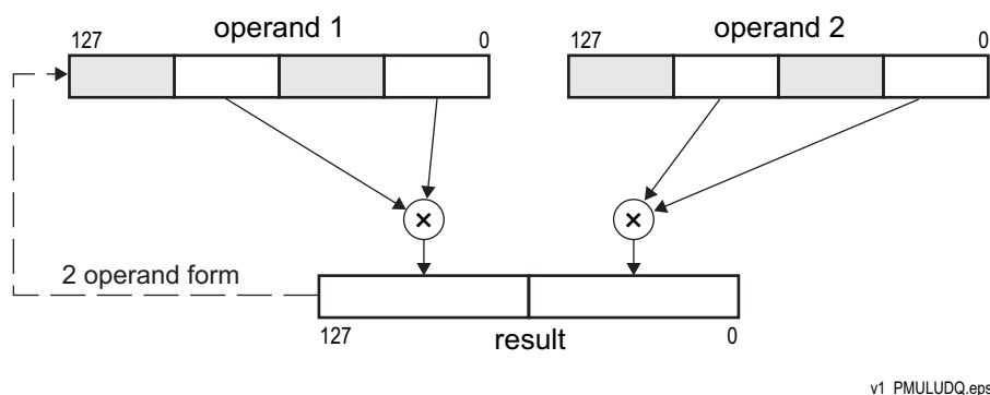
Figure 4-33. PMULUDQ Multiply Operation
