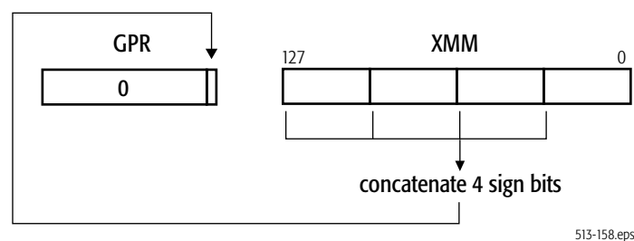
Figure 4-40. MOVMSKPS Move Mask Operation
