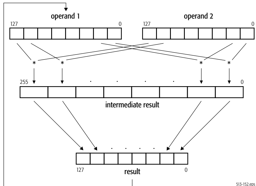
Figure 4-28. PMULxW Multiply Operation
