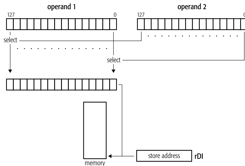
Figure 4-20. MASKMOVDQU Move Mask Operation
