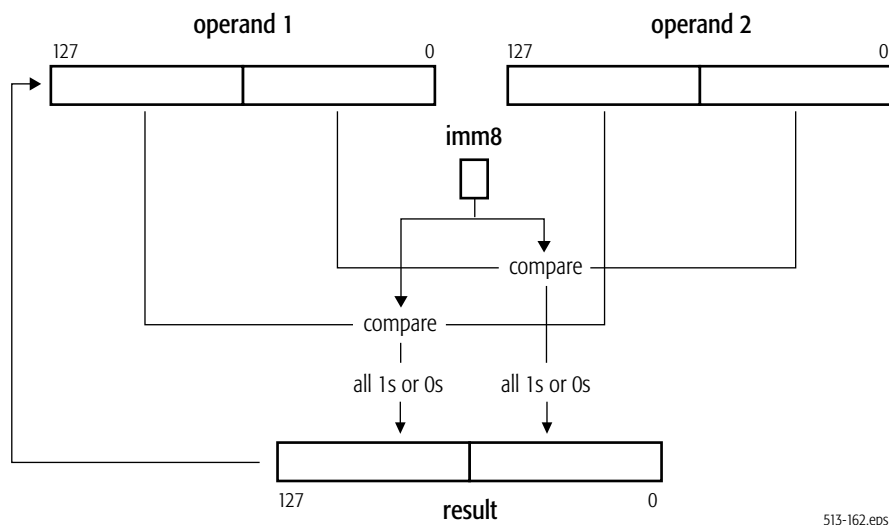
Figure 4-41. CMPPD Compare Operation
