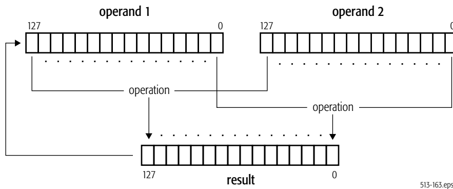
Figure 4-27. Arithmetic Operation on Vectors of Bytes
