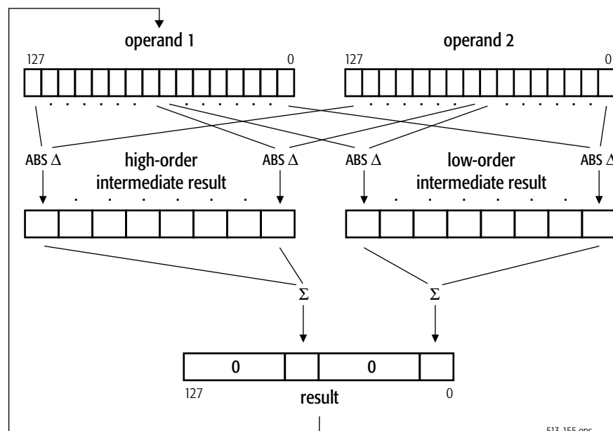
Figure 4-33. PSADBW Sum-of-Absolute-Differences Operation
