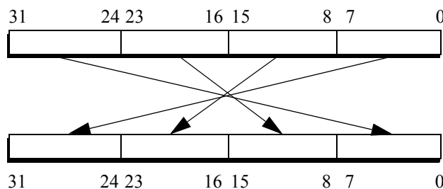
Figure 3-8. BSWAP Doubleword Exchange
