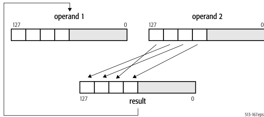
Figure 4-26. PSHUFW Shuffle Operation
