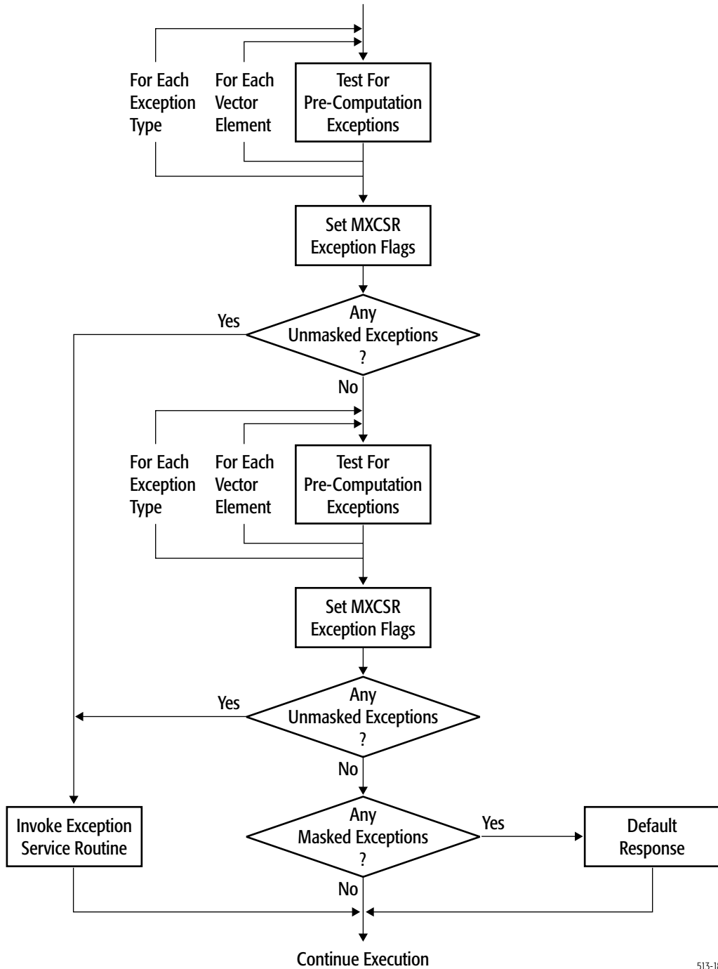
Figure 4-43. SIMD Floating-Point Detection Process
