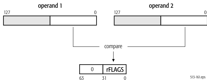
Figure 4-42. COMISD Compare Operation
