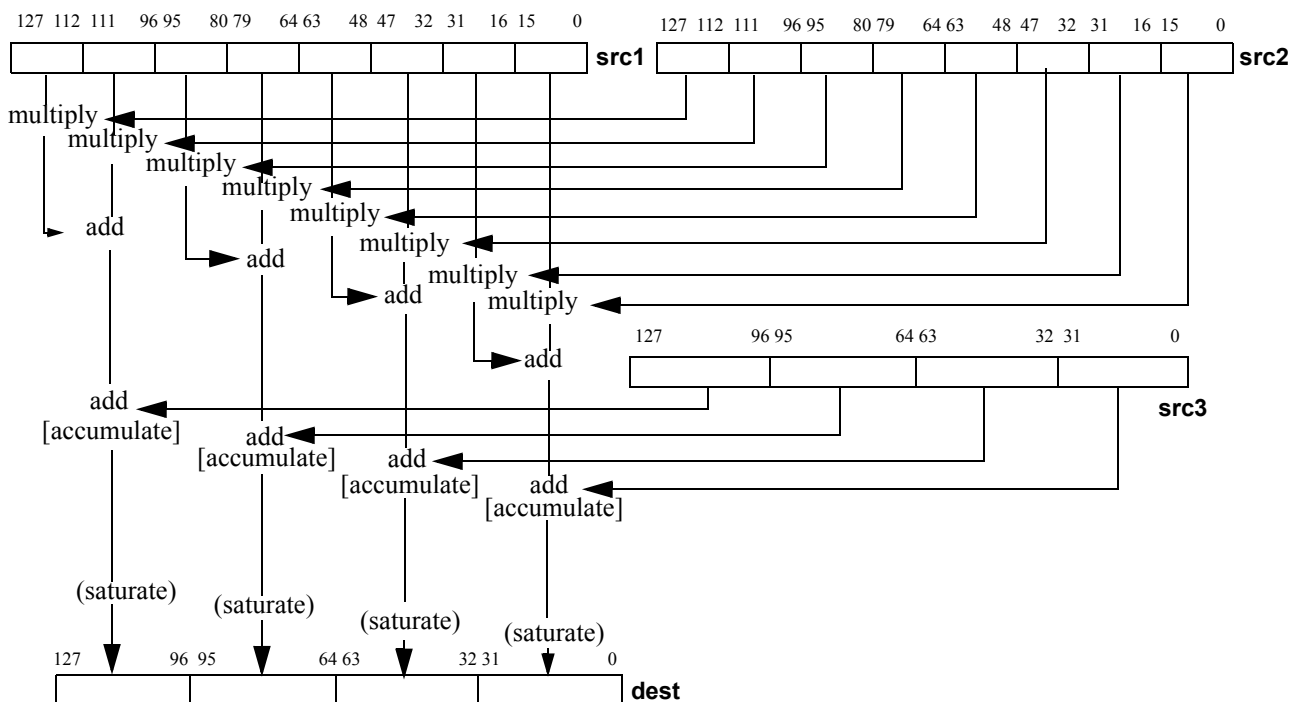
Figure 4-32. Operation of Multiply, Add and Accumulate Instructions
