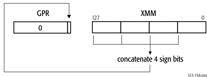
Figure 4-36. MOVMSKPS Move Mask Operation
