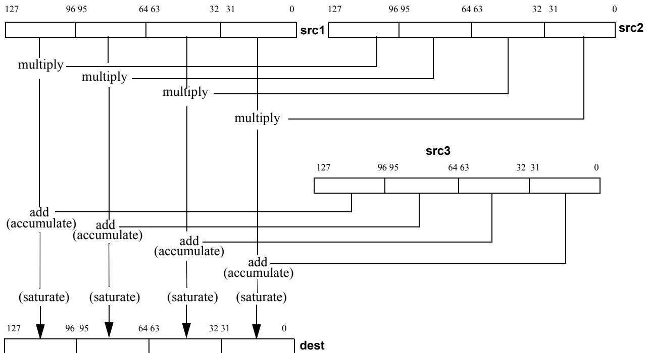
Figure 4-31. Operation of Multiply and Accumulate Instructions
