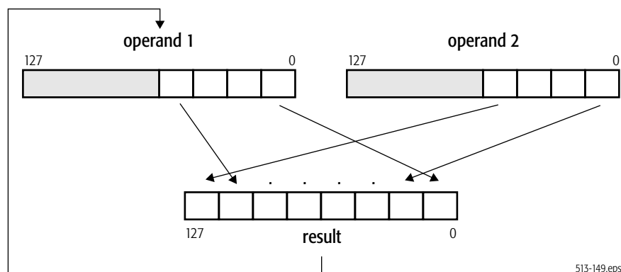
Figure 4-23. PUNPCKLWD Unpack and Interleave Operation
