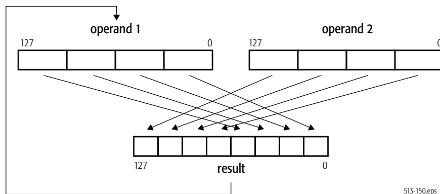
Figure 4-22. PACKSSDW Pack Operation
