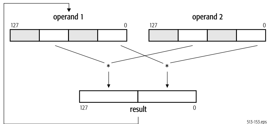
Figure 4-29. PMULUDQ Multiply Operation
