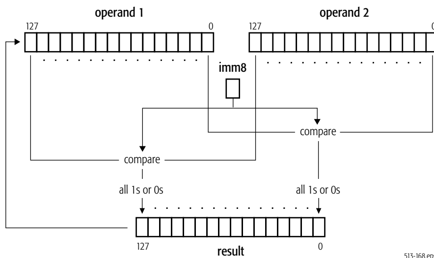
Figure 4-34. PCMPEQB Compare Operation
