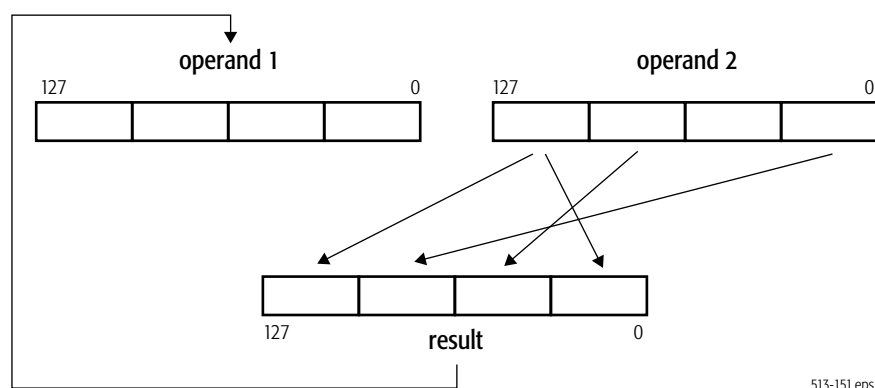
Figure 4-25. PSHUFD Shuffle Operation
