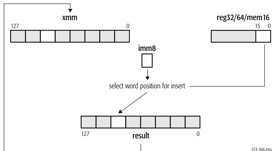
Figure 4-24. PINSRW Operation
