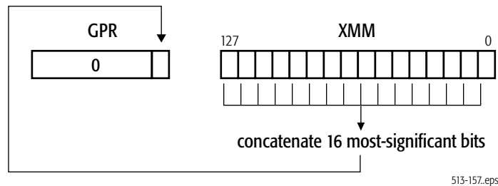
Figure 4-21. PMOVMSKB Move Mask Operation
