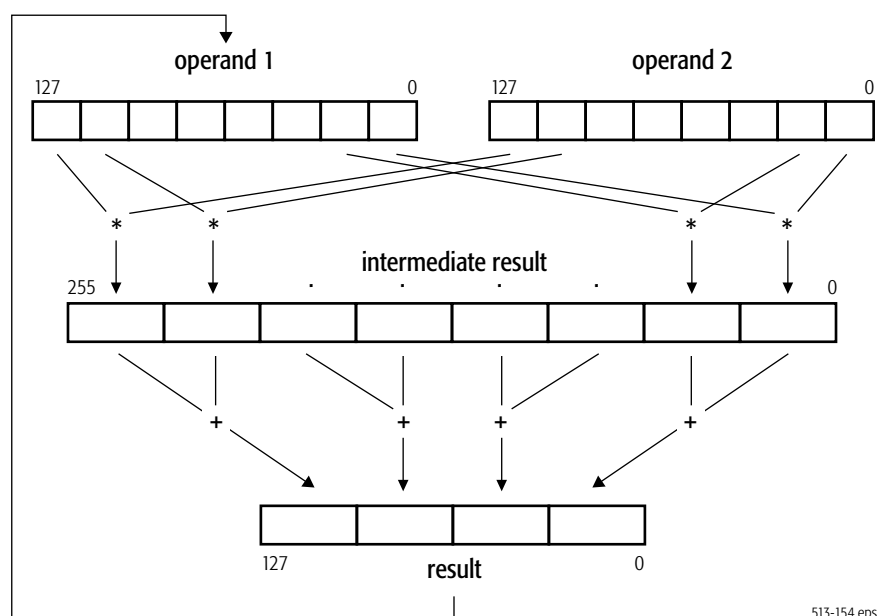
Figure 4-30. PMADDWD Multiply-Add Operation
