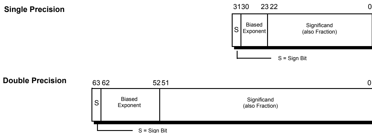
Figure 4-17. SSE Floating-Point Data Types
