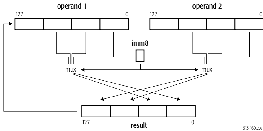
Figure 4-39. SHUFPS Shuffle Operation
