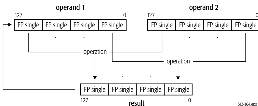
Figure 4-40. ADDPS Arithmetic Operation
