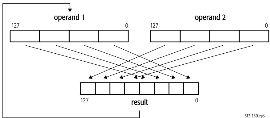
Figure 4-4. Pack Operation
