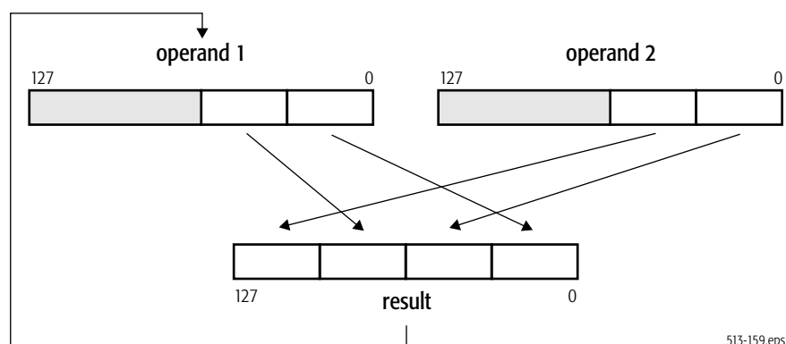
Figure 4-38. UNPCKLPS Unpack and Interleave Operation
