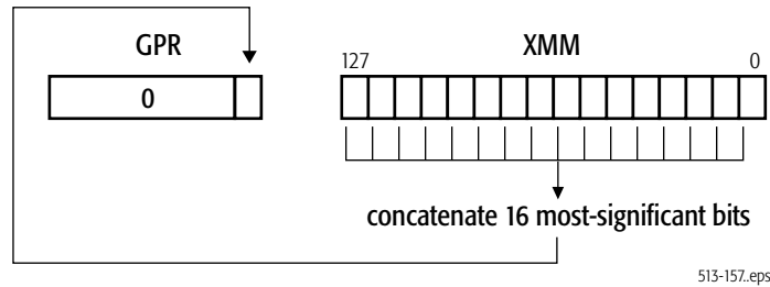
Figure 4-11. Move Mask Operation
