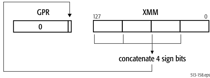
Figure 4-32. MOVMSKPS Move Mask Operation
