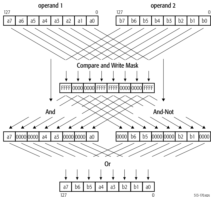
Figure 4-10. Branch-Removal Sequence
