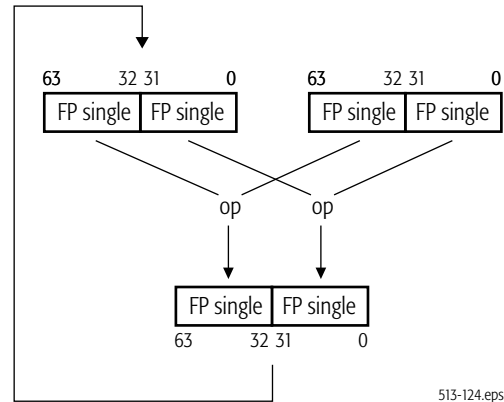
Figure 5-6. Floating-Point (3DNow!™) Operations
