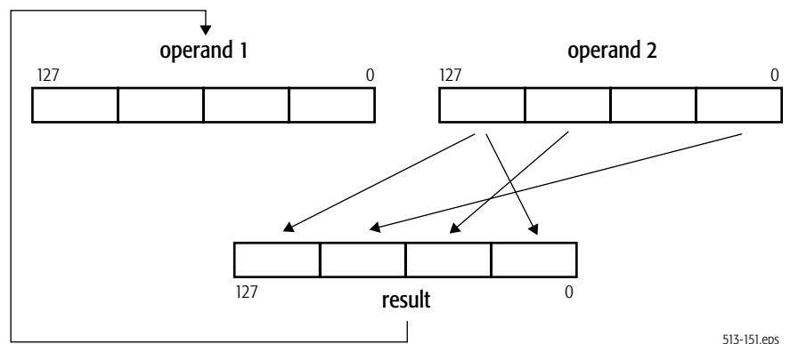
Figure 4-5. Shuffle Operation
