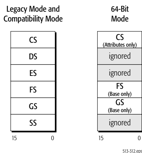
Figure 2-2. Segment Registers
