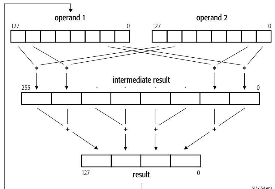
Figure 4-8. Multiply-Add Operation
