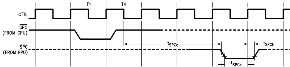
FIGURE 4-13. SPC Timing
