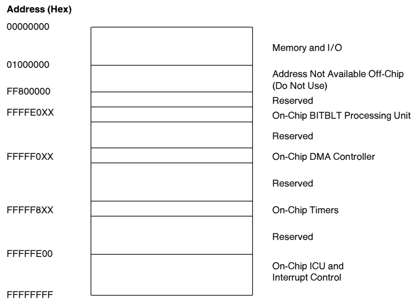
FIGURE 2-20. NS32CG160 Address Mapping
