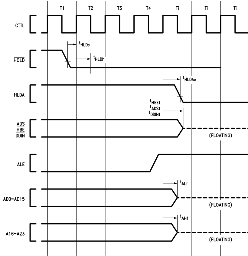
FIGURE 4-8. \overline{\text{HOLD}} Acknowledge Timing (Bus Initially Not Idle)
