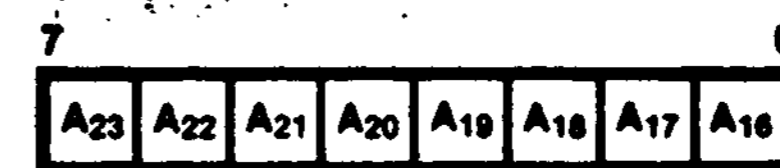
Figure 3-8. I/O Page Register
