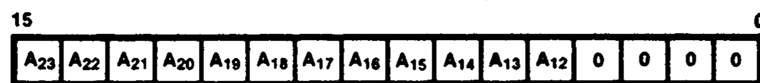
Figure 3-7. Interrupt/Trap Vector Table Pointer
