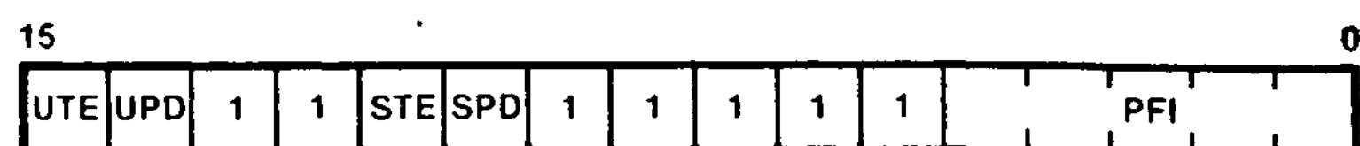
Figure 7-4. MMU Master Control Register
