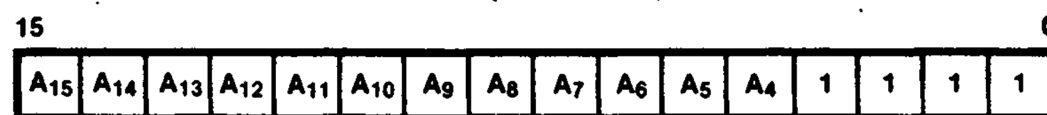
Figure 3-10. System Stack Limit Register
