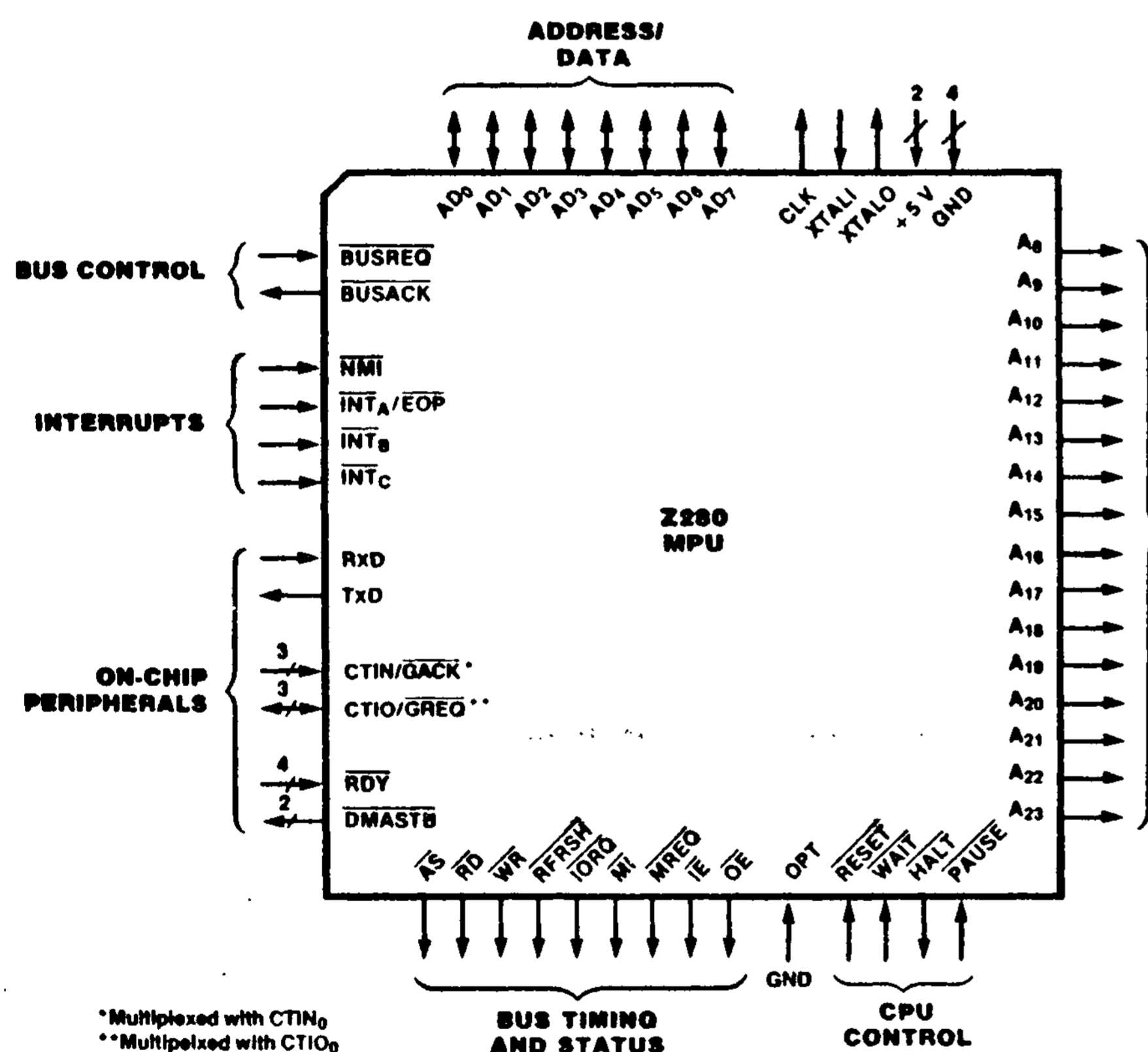
Figure 12-1a. Pin Functions
