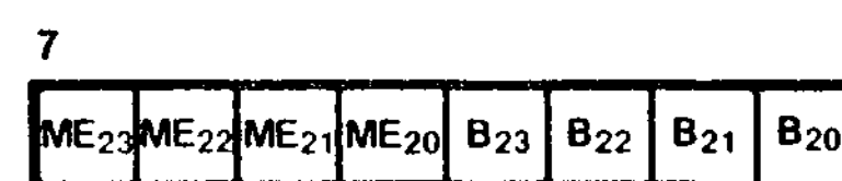
Figure 10-2. Local Address Register
