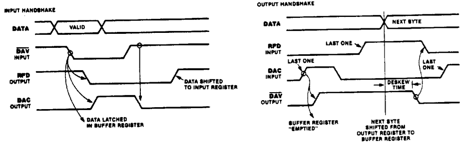
Figure 8. 3-Wire Handshake
