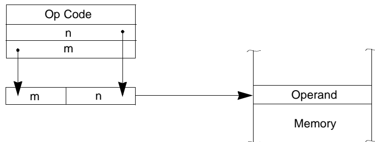
Figure 78. Extended Addressing
