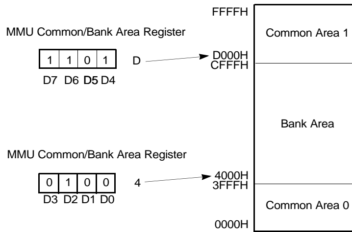
Figure 28. Logical Space Configuration (Example)
