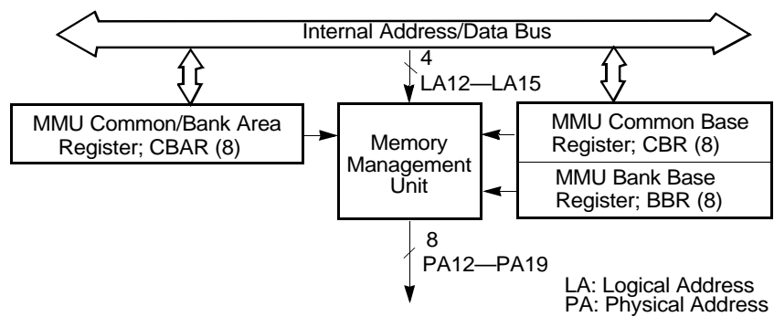
Figure 25. MMU Block Diagram
