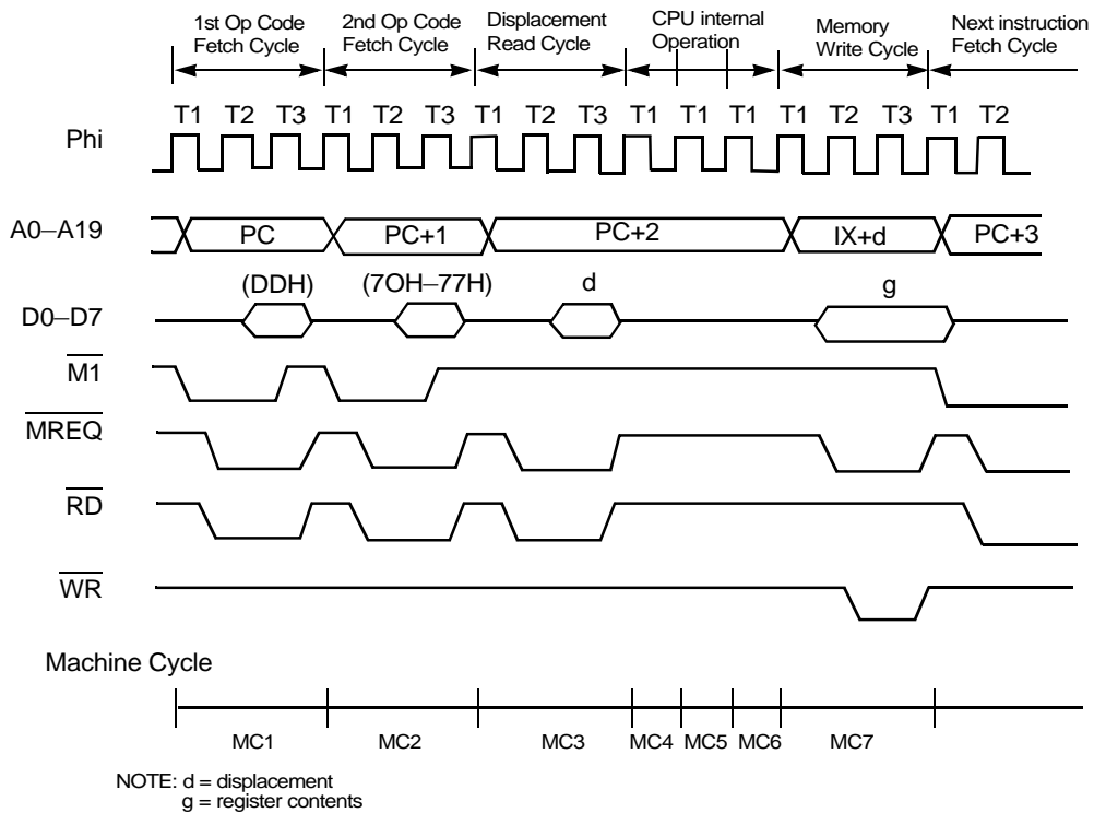
Figure 14. Instruction Timing Diagram
