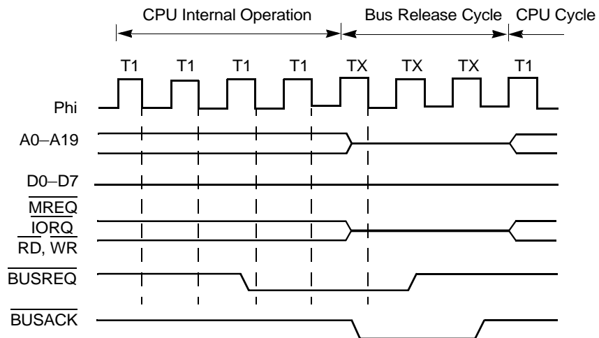
Figure 17. Bus Exchange Timing During CPU Internal Operation
