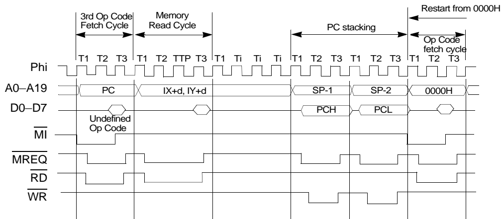
Figure 33. TRAP Timing - 3rd Op Code Undefined
