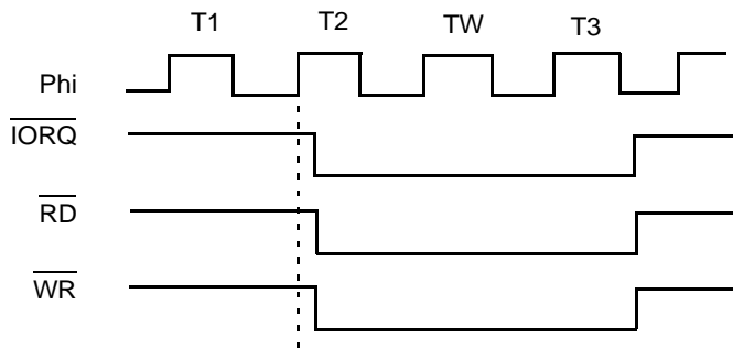
Figure 8. I/O Read and Write cycles with IOE = 0 Timing Diagram
