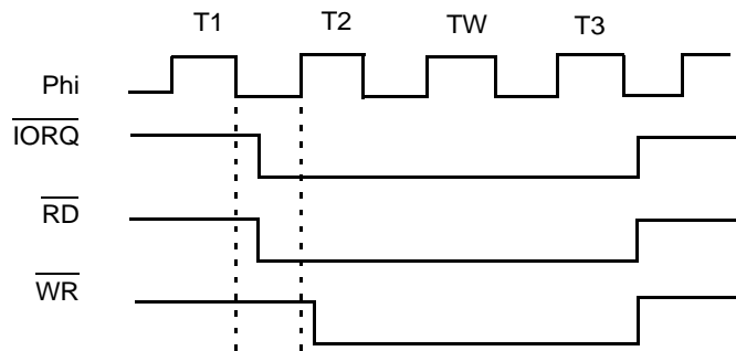
Figure 7. I/O Read and Write Cycles with \overline{IOE} = 1 Timing Diagram
