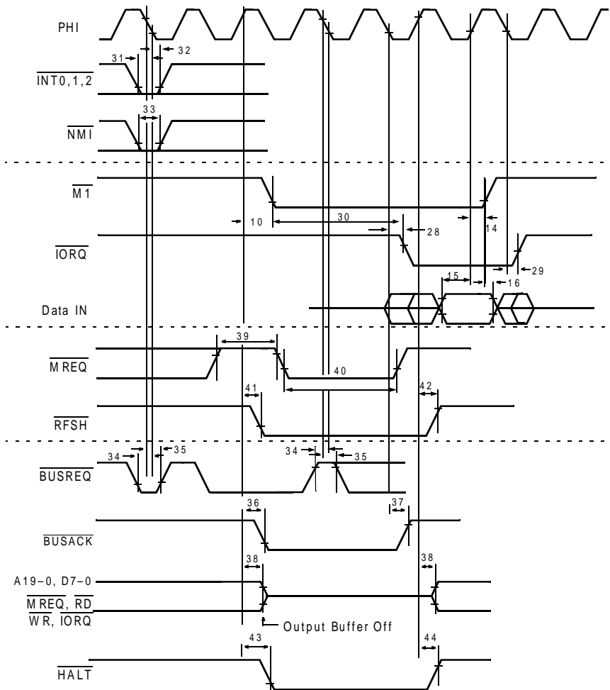
Figure 82. AC Timing Diagram 2
