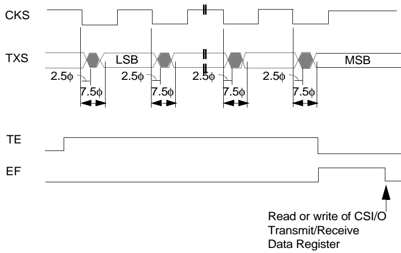
Figure 60. Transmit Timing—External Clock
