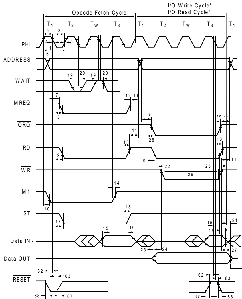
Figure 81. AC Timing Diagram 1
