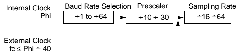
Figure 56. ASCI Clock
