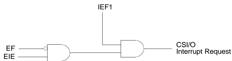
Figure 58. CSI/O Interrupt Request Generation
