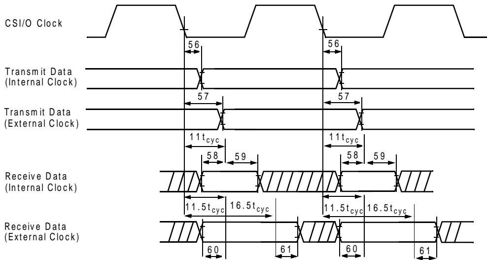
Figure 90. CSI/O Receive/Transmit Timing Diagram
