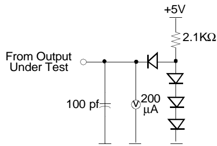
Figure 93. Test Setup
