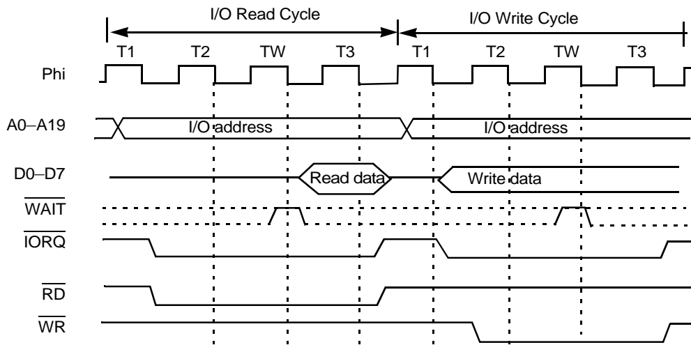
Figure 13. I/O Read/Write Timing Diagram
