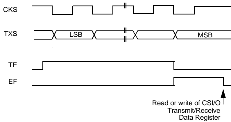
Figure 59. Transmit Timing Diagram-Internal Clock
