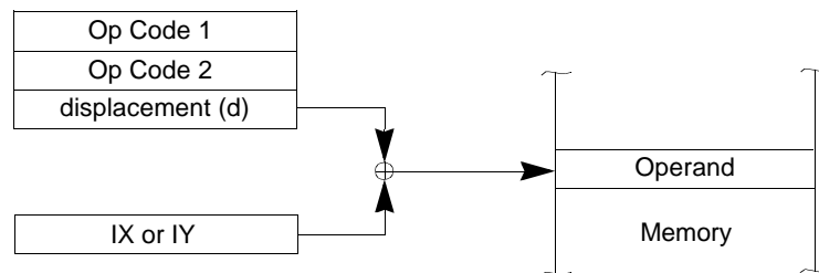
Figure 77. Indexed Addressing
