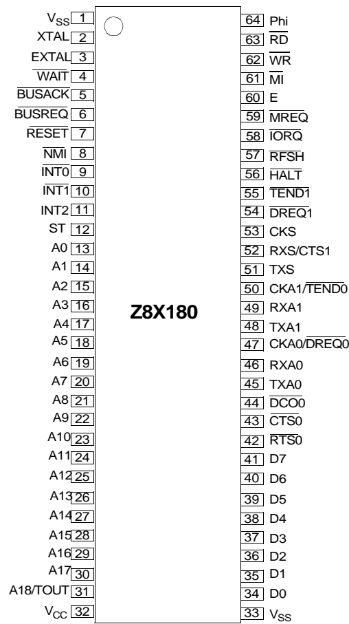
Figure 1. 64-Pin DIP
