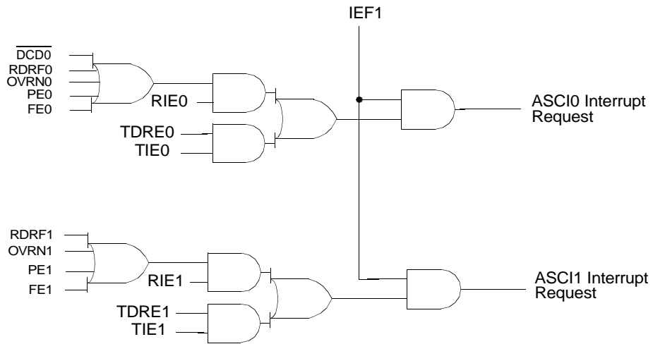
Figure 55. ASCI Interrupt Request Circuit Diagram
