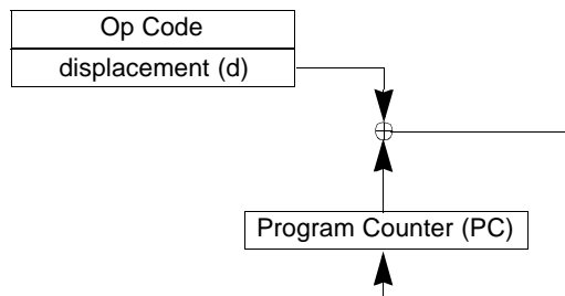
Figure 80. Relative Addressing
