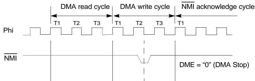
Figure 51. \overline{\text{NMI}} and DMA Operation Timing Diagram
