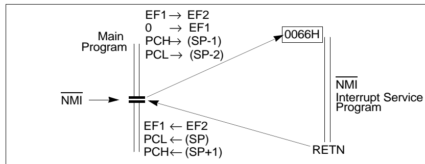
Figure 34. \overline{\text{NMI}} Use
