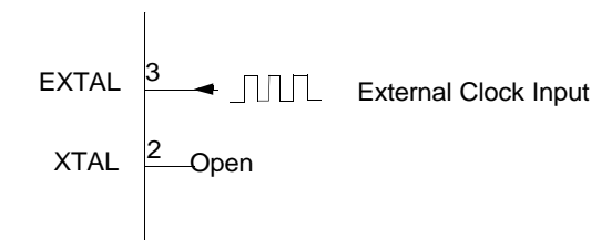
Figure 70. External Clock Interface
