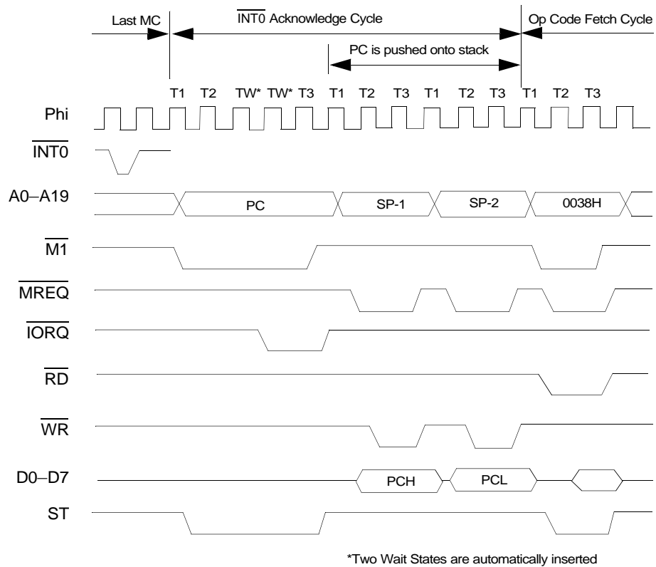
Figure 38. \overline{\text{INT0}} Mode 1 Timing
