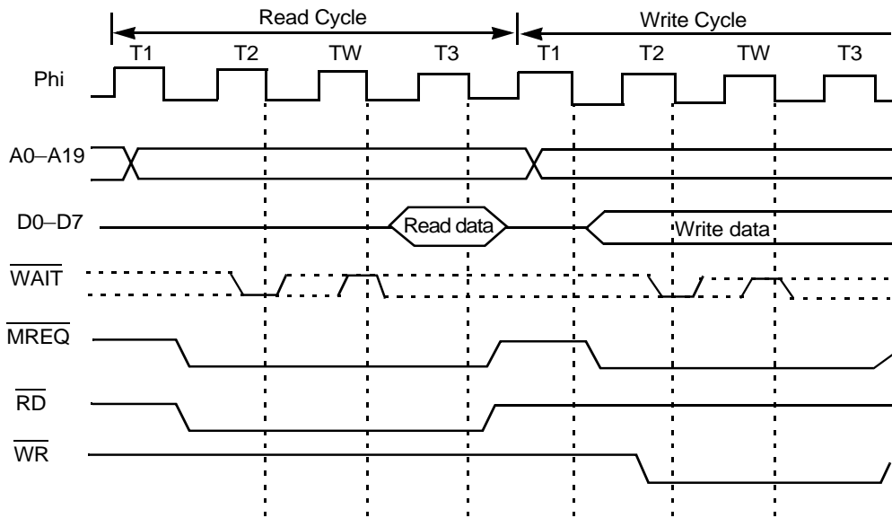
Figure 12. Memory Read/Write (with Wait State) Timing Diagram
