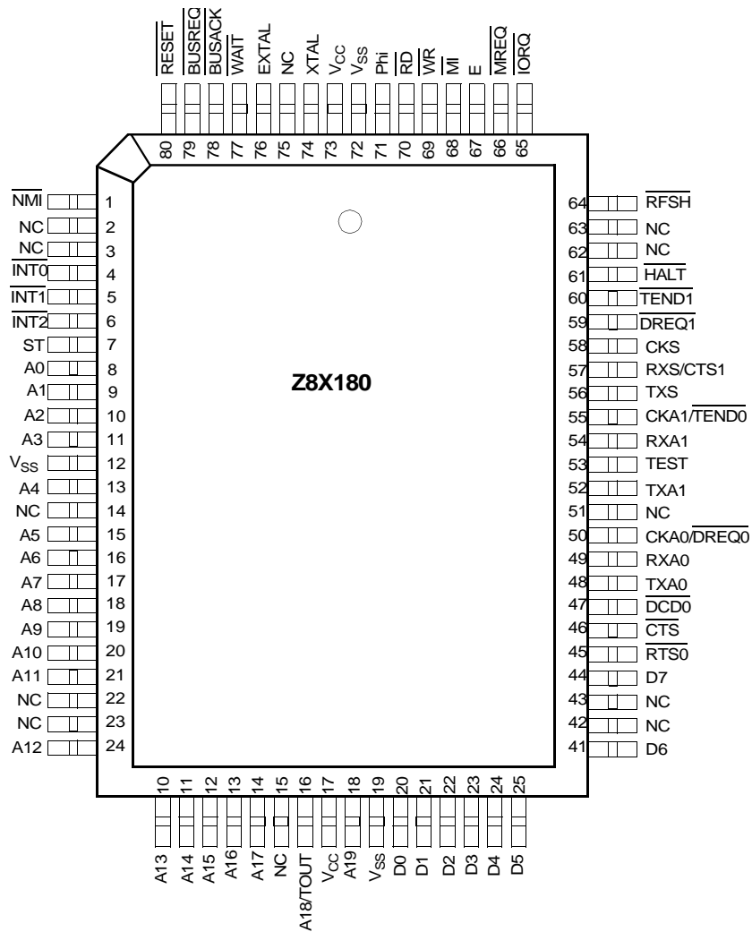
Figure 3. 80-Pin QFP
