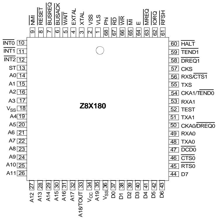
Figure 2. 68-Pin PLCC
