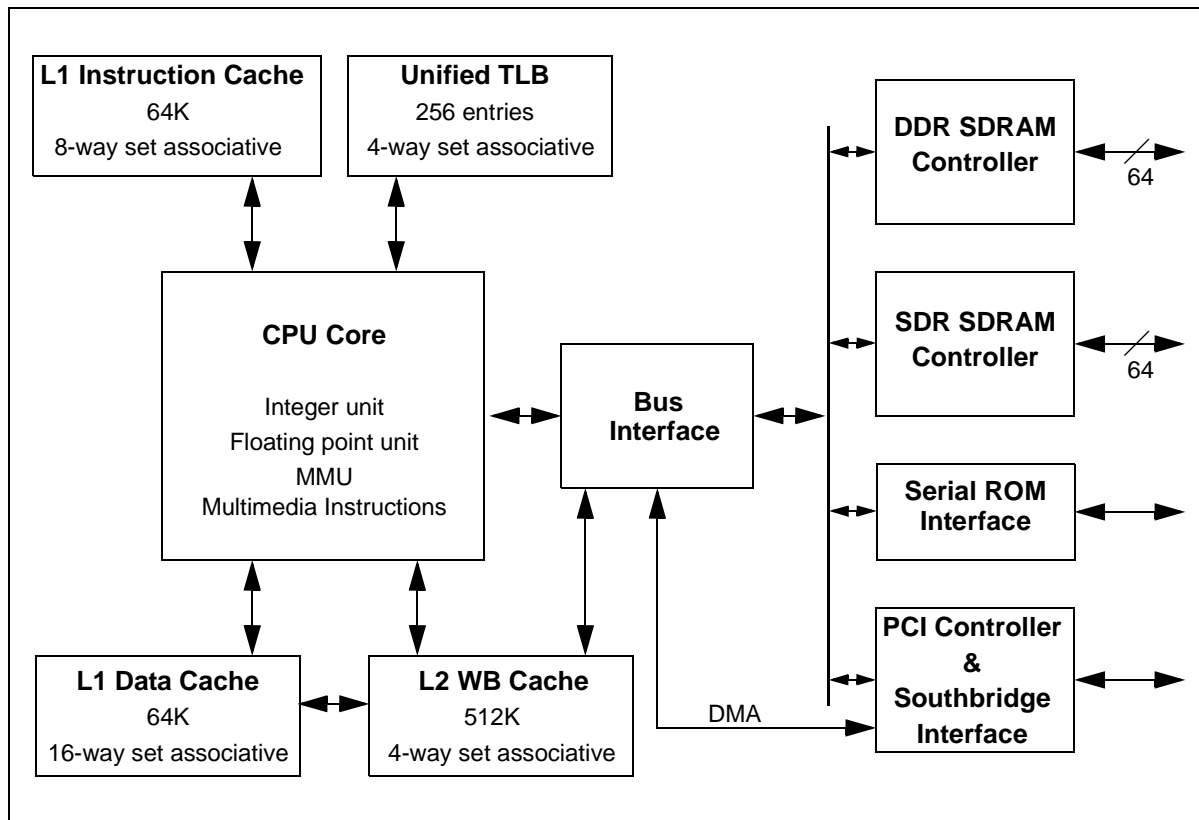
FIGURE 1. Crusoe Processor Block Diagram - Model TM5600
