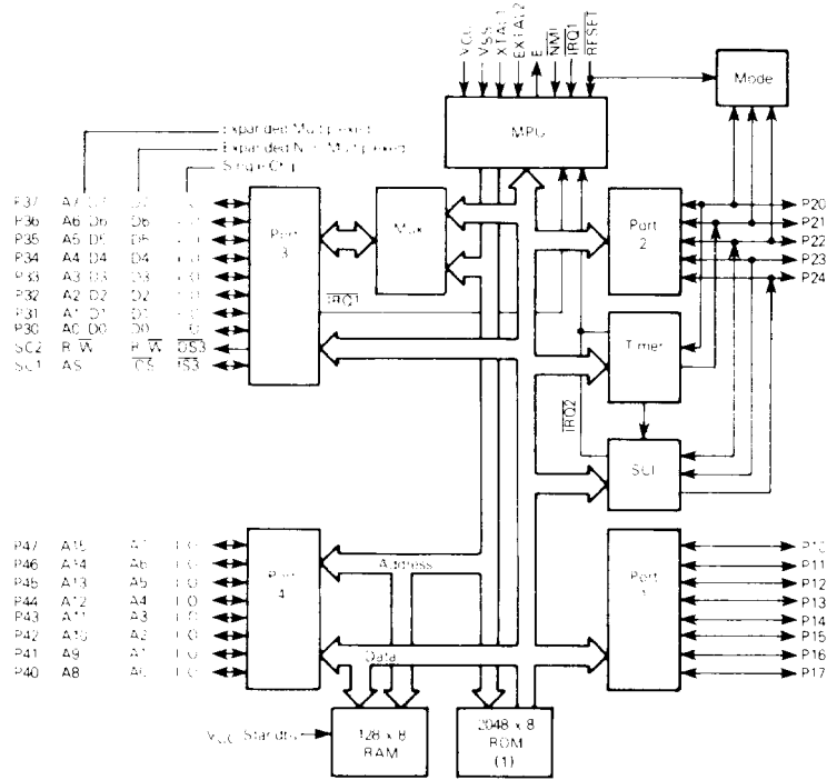
FIGURE 1 – 6801/6803 BLOCK DIAGRAM
