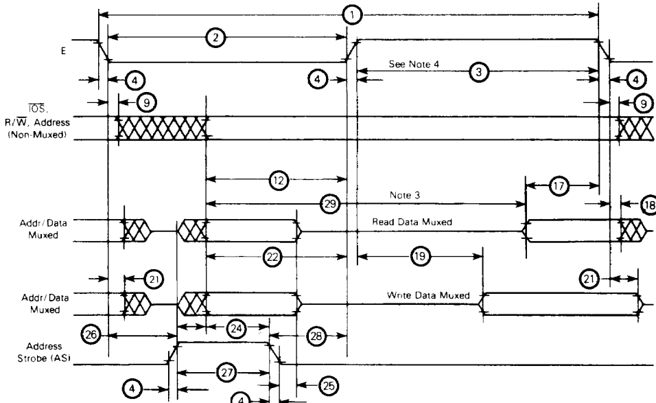
FIGURE 6 – BUS TIMING
