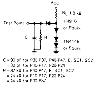
FIGURE 8 – TIMING TEST LOAD PORTS 1, 2, 3, 4
