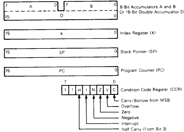
FIGURE 9 – PROGRAMMING MODEL
