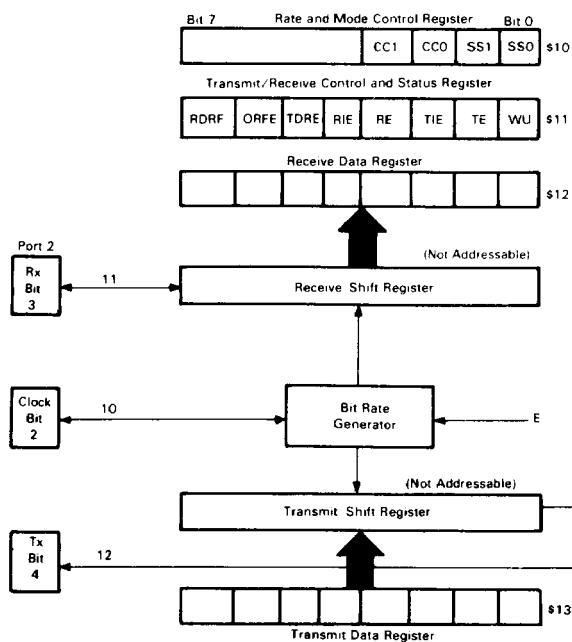
FIGURE 23 – SCI REGISTERS
