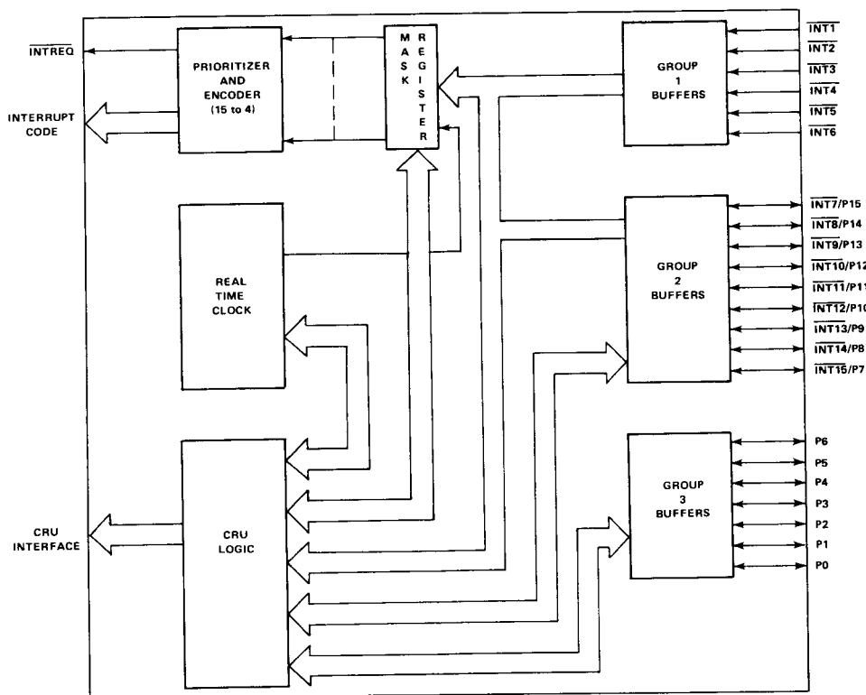
FIGURE 2 - TMS 9901 BLOCK DIAGRAM
