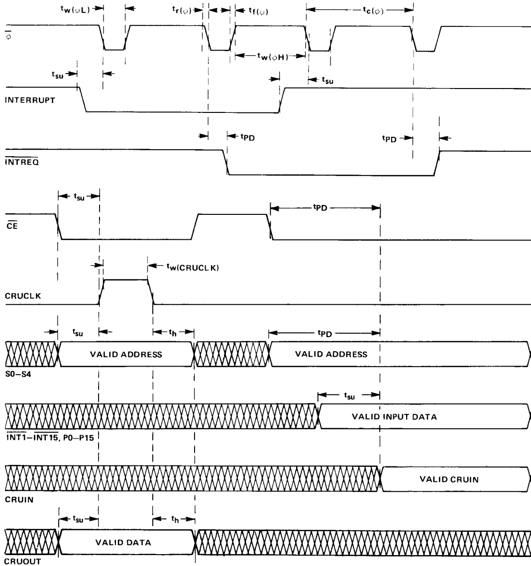
FIGURE 8 – SWITCHING CHARACTERISTICS
