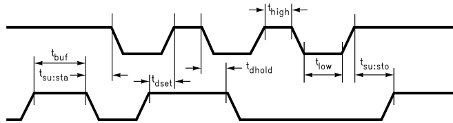
FIGURE 13. Access.bus Timing Diagram
