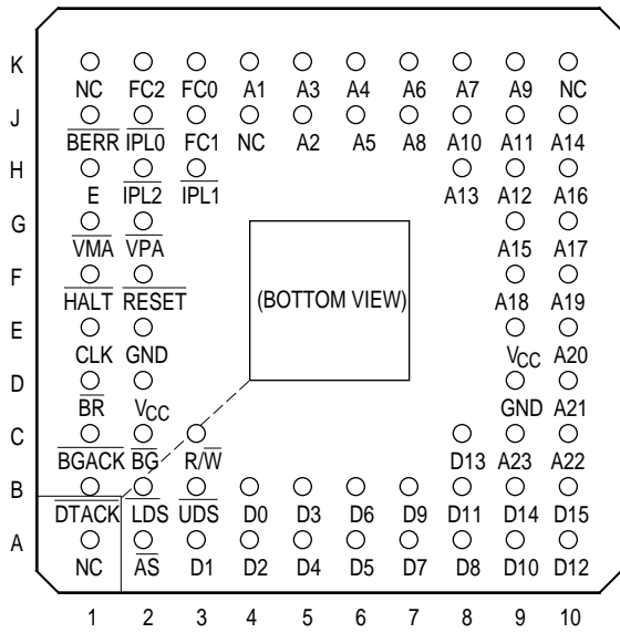
MC68000/MC68010/MC68HC000
