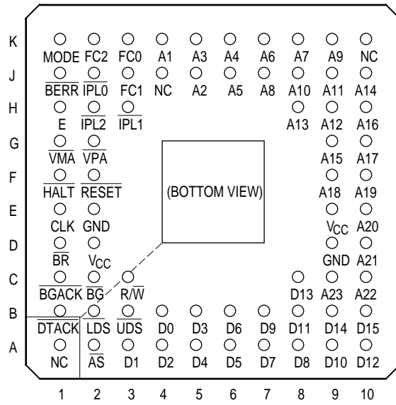
MC68HC001
