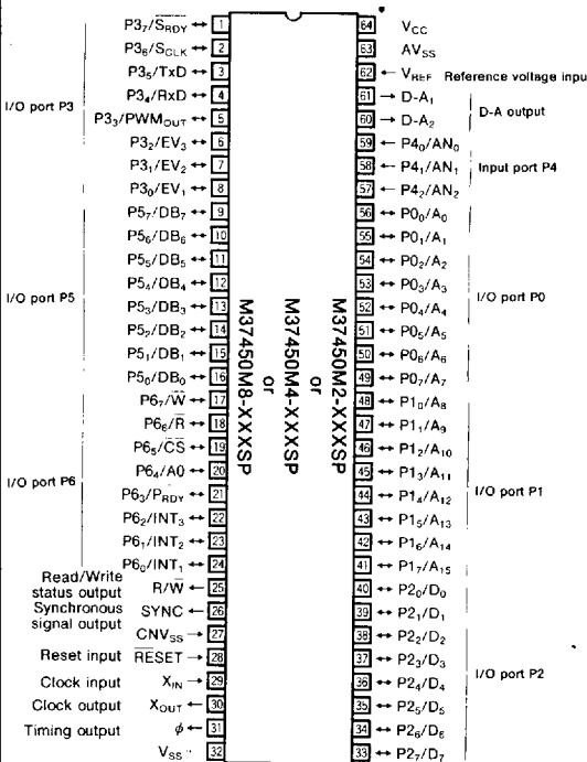
Outline 64P4B
