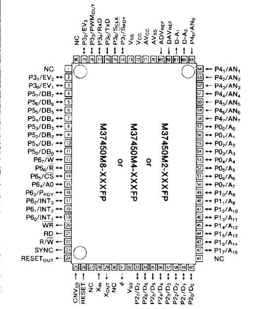
Outline 80P6
