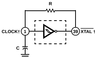
FIGURE 9. RC NETWORK FOR OSCILLATOR
