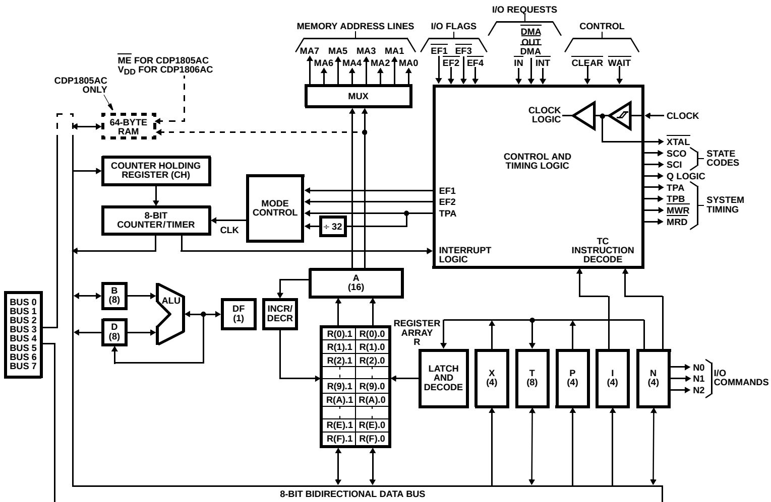
FIGURE 2. BLOCK DIAGRAM FOR CDP1805AC AND CDP1806AC
