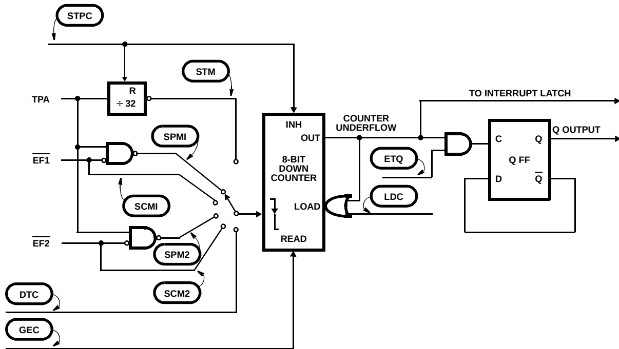
FIGURE 7. TIMER/COUNTER DIAGRAM
