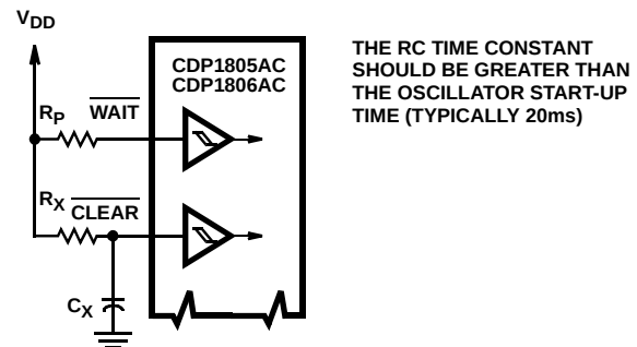
FIGURE 11. RESET/RUN DIAGRAM
