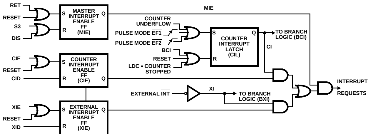
FIGURE 6. INTERRUPT LOGIC CONTROL DIAGRAM
