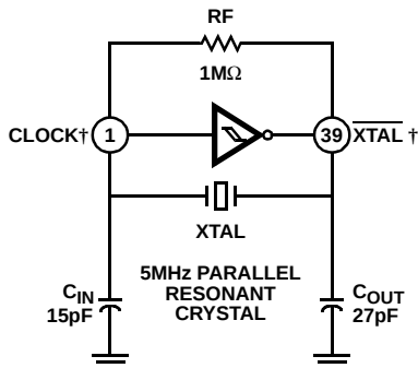
FIGURE 8. TYPICAL 5MHz CRYSTAL OSCILLATOR
