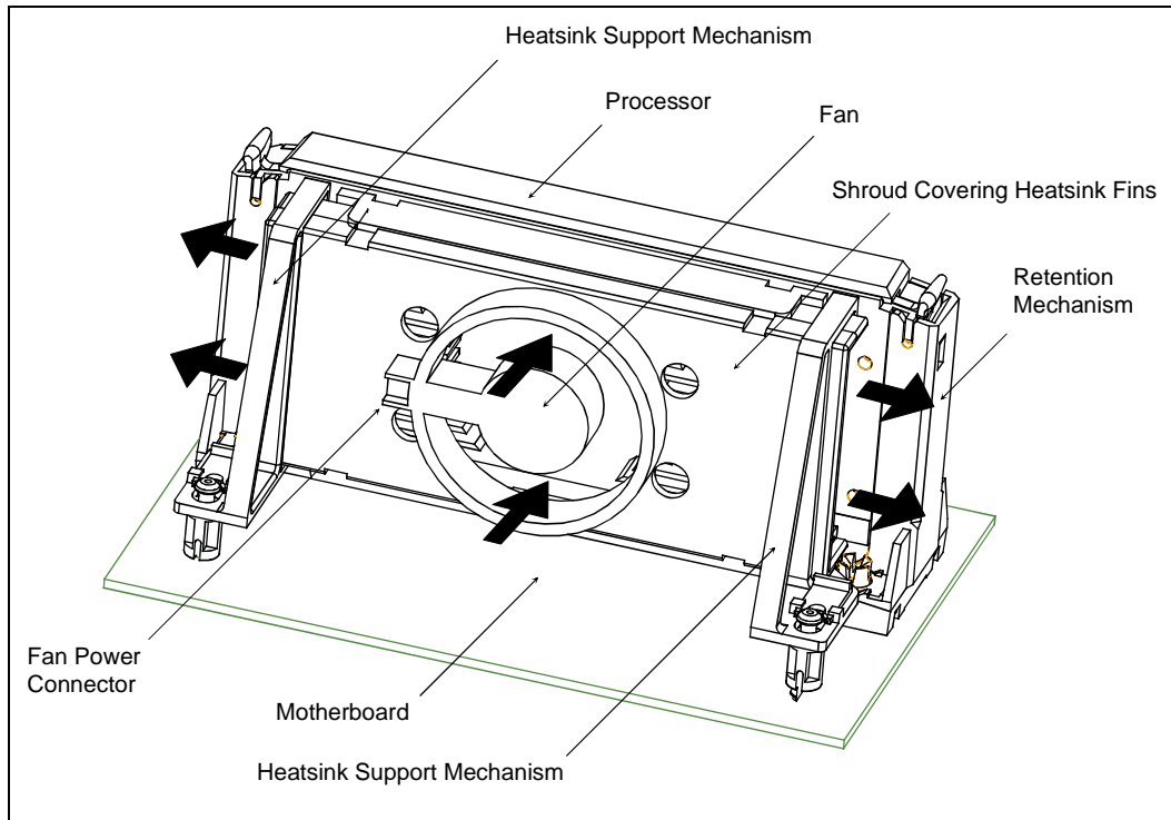
Figure 38. Boxed Pentium® II Processor in Retention Mechanism (Fan Power Cable Not Shown)
