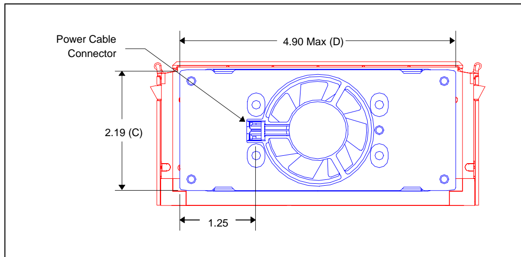
Figure 40. Front View Space Requirements for the Boxed Processor
