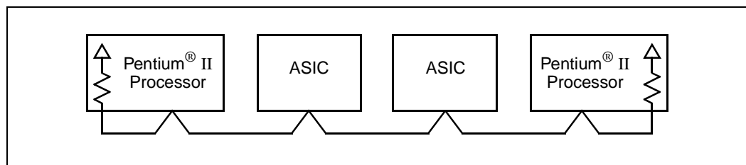
Figure 2. GTL+ Bus Topology
