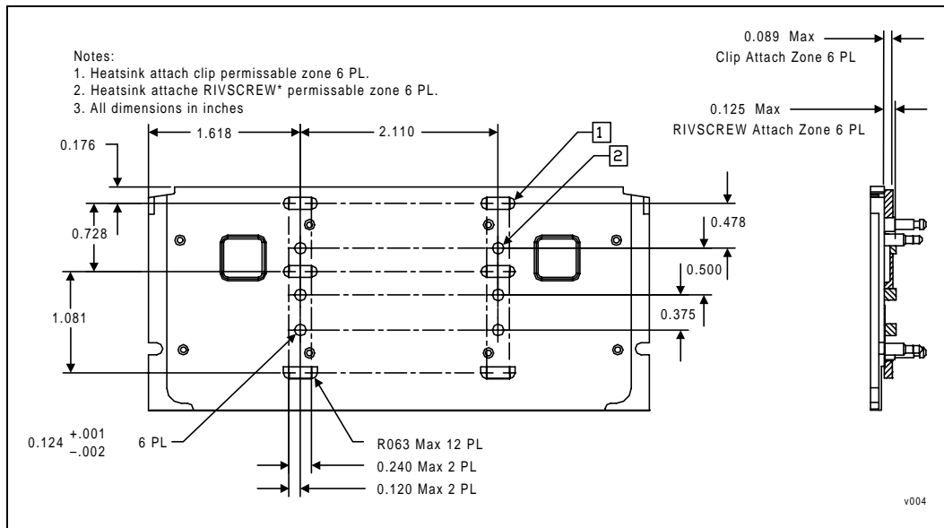
Figure 22. Heatsink Attachment Mechanism Design Space
