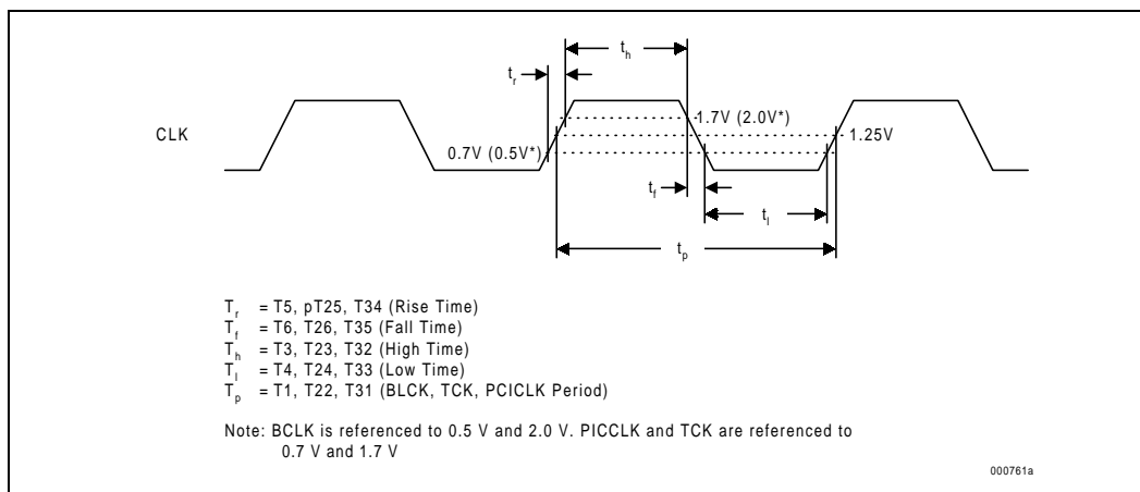
Figure 6. BCLK, PICCLK, and TCK Generic Clock Waveform
