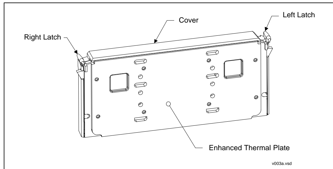
Figure 17. Pentium® II 100 MHz Processor S.E.C. Cartridge, Enhanced Thermal Plate (ETP) Side View
