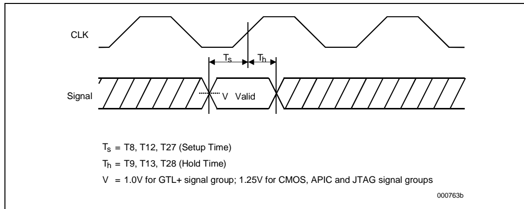
Figure 8. Pentium® II Processor System Bus Setup and Hold Timings
