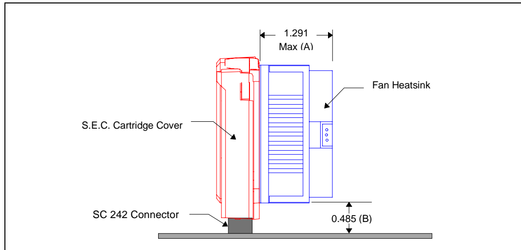
Figure 39. Side View Space Requirements for the Boxed Processor (Fan Heatsink Supports Not Shown)
