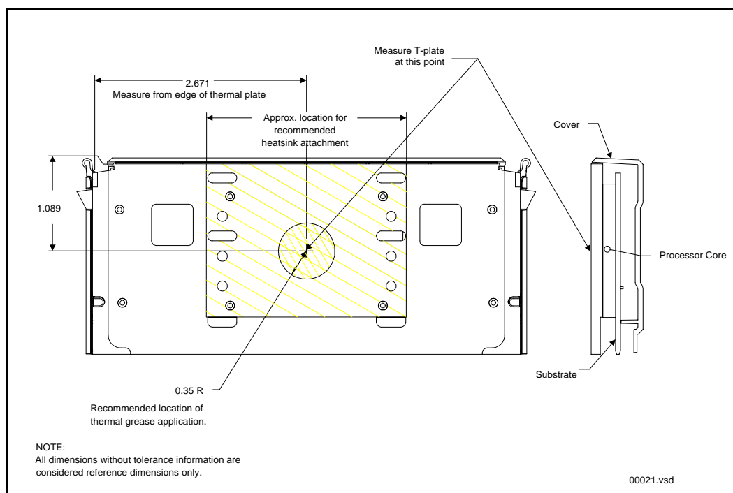
Figure 18. Processor Thermal Plate Temperature Measurement Location
