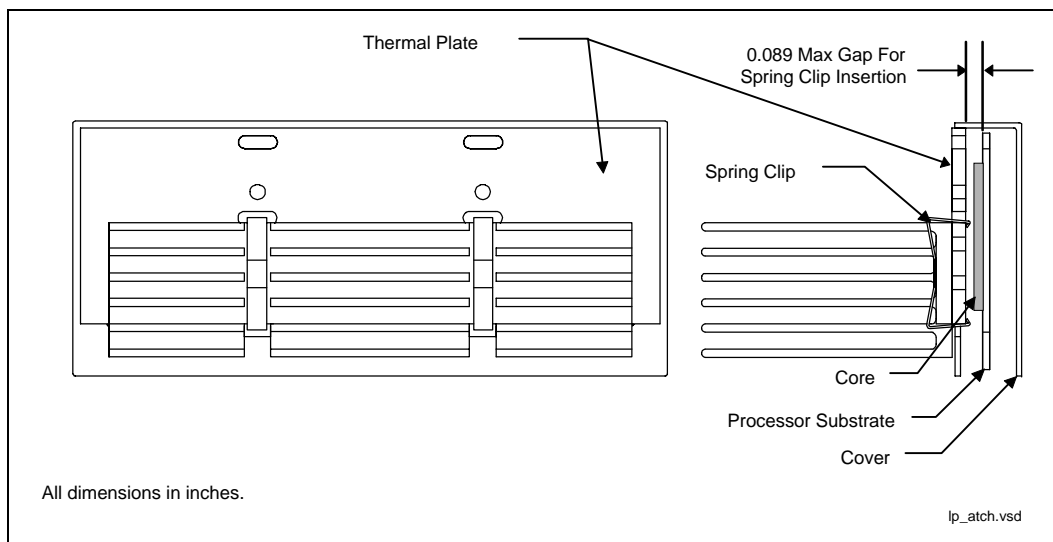
Figure 23. Processor With Low Profile Heatsink Attached Using Spring Clips
