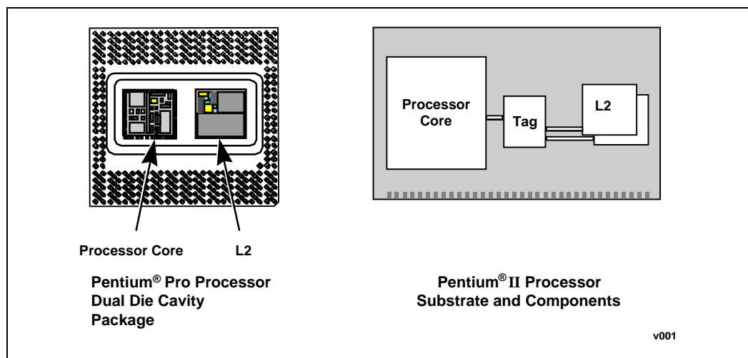
Figure 1. Second Level (L2) Cache Implementations
