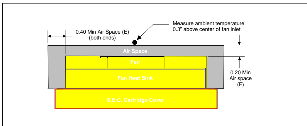
Figure 41. Top View Space Requirements for the Boxed Processor
