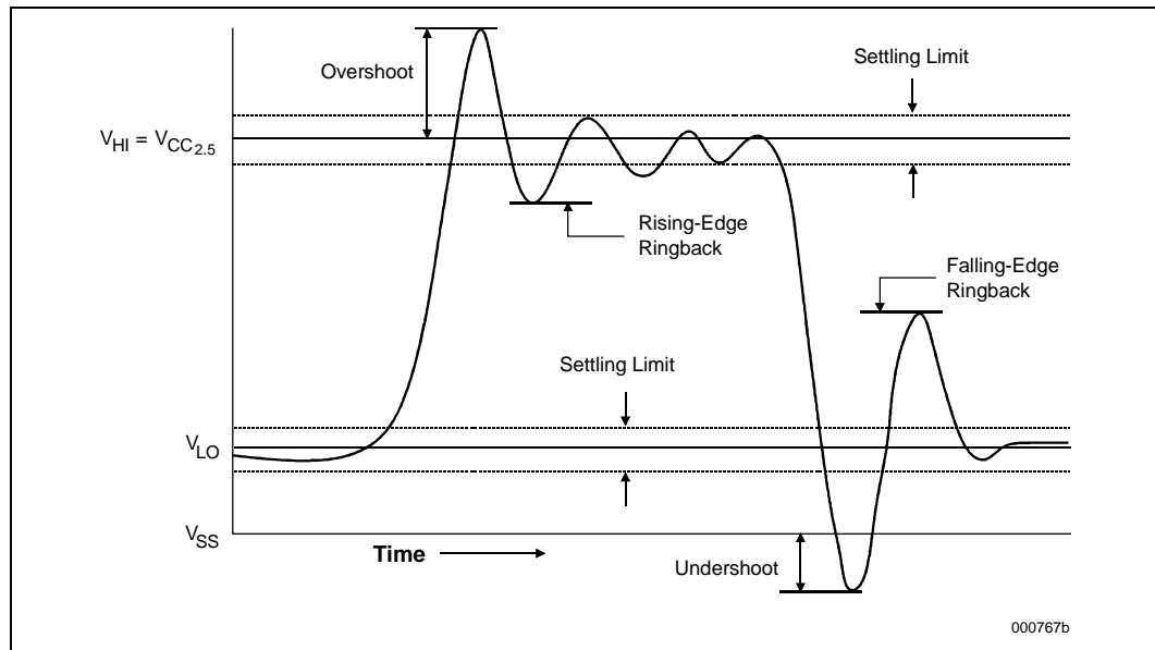
Figure 16. Non-GTL+ Overshoot/Undershoot, Settling Limit, and Ringback
