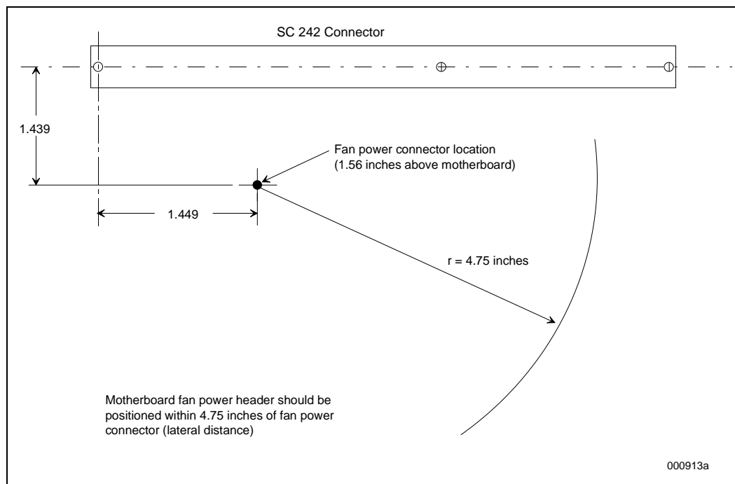
Figure 46. Recommended Motherboard Power Header Placement Relative to Fan Power Connector and Pentium® II Processor
