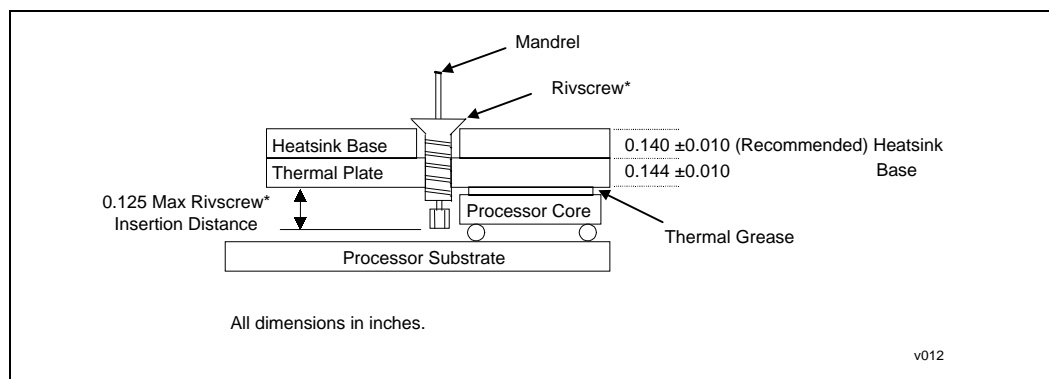
Figure 27. General Rivscrew* Heatsink Mechanical Recommendations
