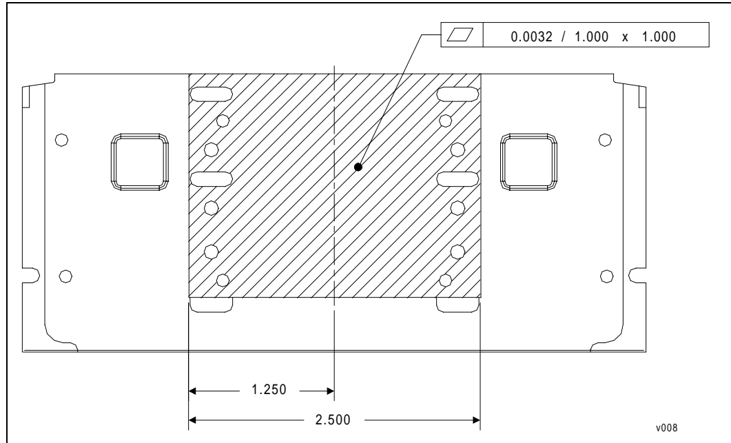
Figure 34. Pentium® II Processor S.E.C. Cartridge Thermal Plate Attachment Detail Dimensions, Continued
