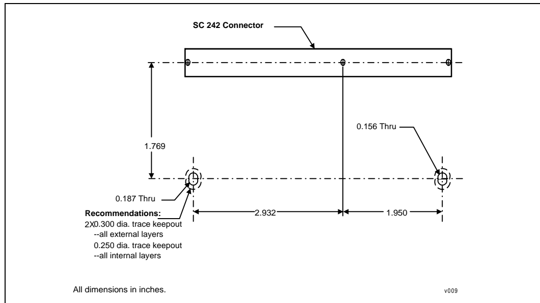
Figure 42. Heatsink Support Hole Locations and Size
