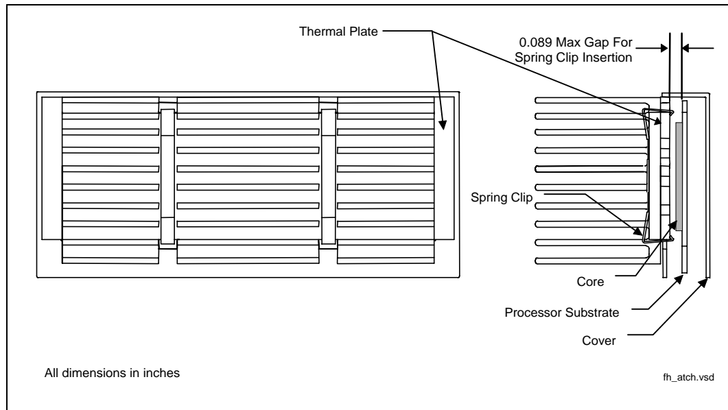
Figure 24. Processor With Full Height Heatsink Attached Using Spring Clips
