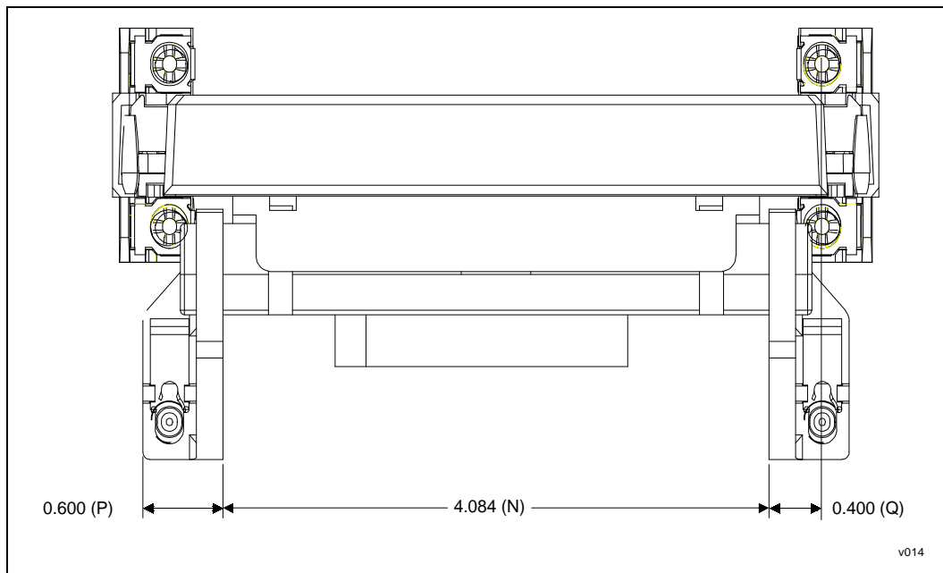
Figure 44. Top View Space Requirements for Boxed Processor Fan Heatsink Supports
