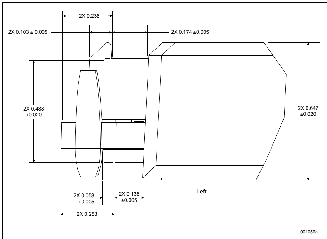
Figure 31. Pentium® II Processor S.E.C. Cartridge Latch Arm, Thermal Plate Lug, and Cover Lug Dimensions
