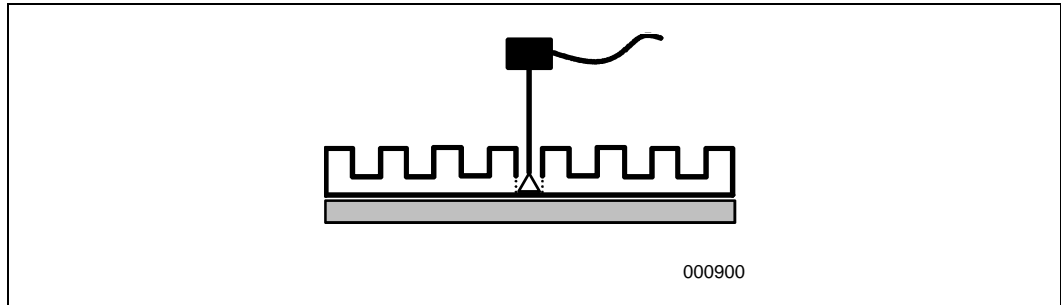
Figure 20. Technique for Measuring T_{PLATE} with 90° Angle Attachment
