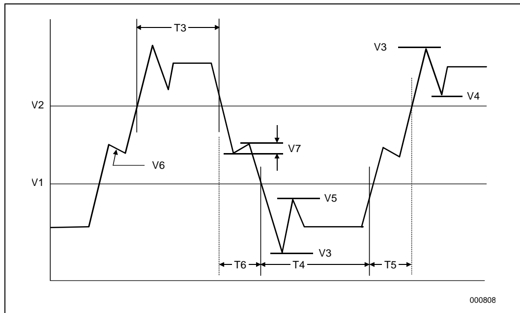
Figure 14. BCLK, TCK, PICCLK Generic Clock Waveform at the Processor Edge Fingers
