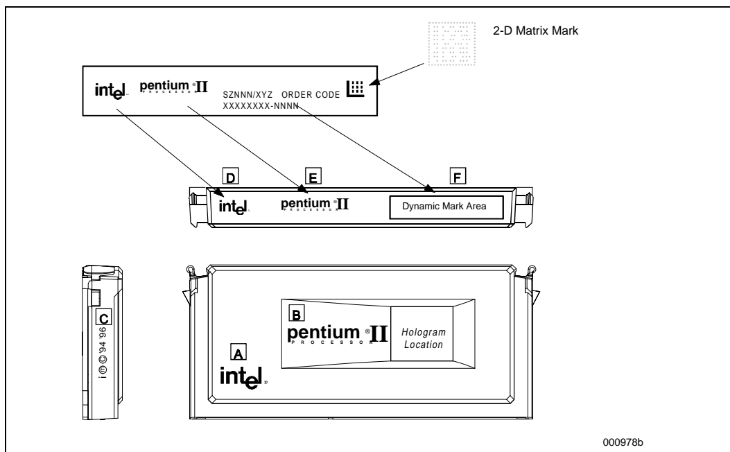
Figure 37. Pentium® II Processor S.E.C. Cartridge Markings
