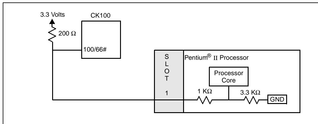
Figure 4. 100/66# Pin Example
