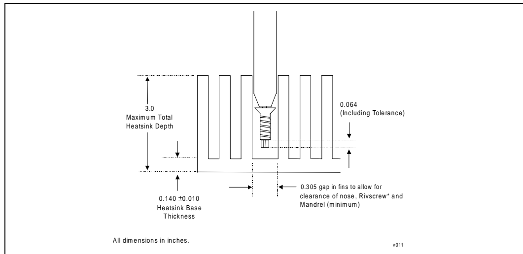
Figure 25. Heatsink Recommendations and Guidelines for Use With Rivscrews*
