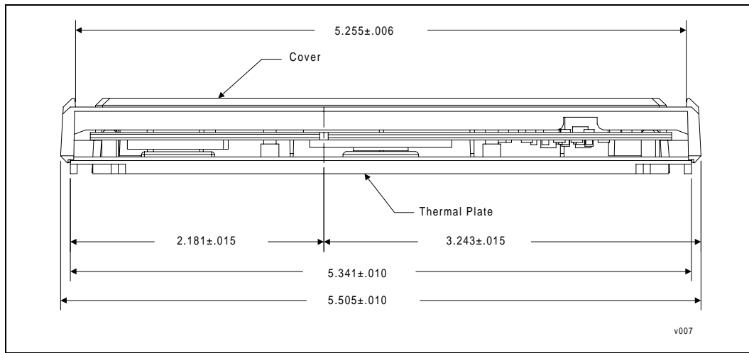
Figure 31. Pentium® II Processor S.E.C. Cartridge Latch Arm, Thermal Plate Lug, and Cover Lug Dimensions
