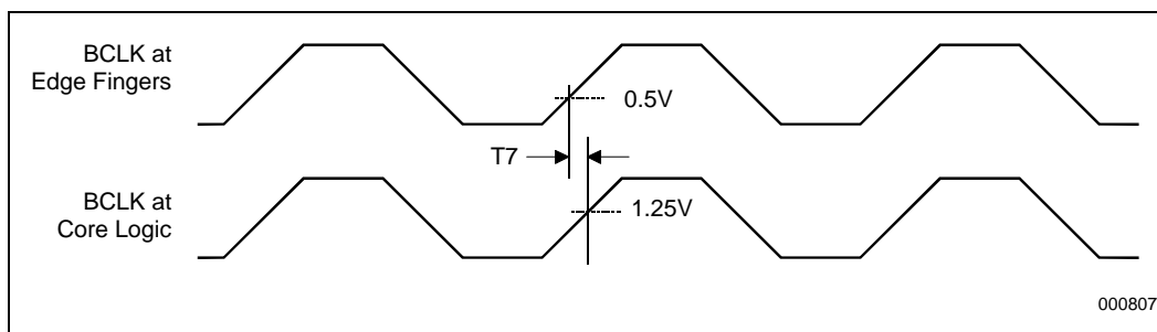
Figure 6. BCLK, PICCLK, and TCK Generic Clock Waveform
