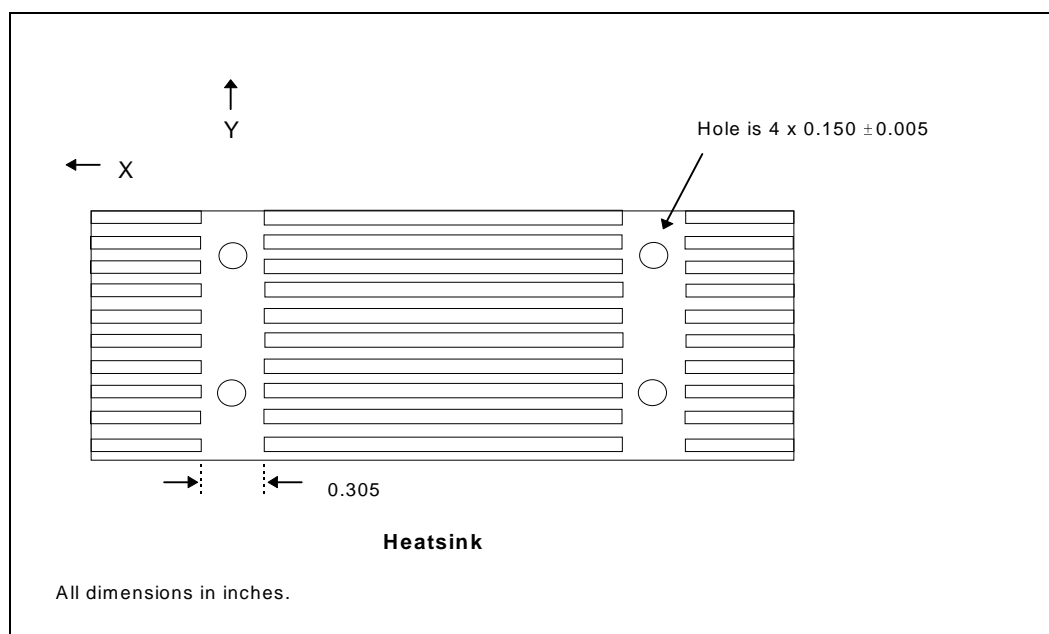
Figure 27. General Rivscrew* Heatsink Mechanical Recommendations
