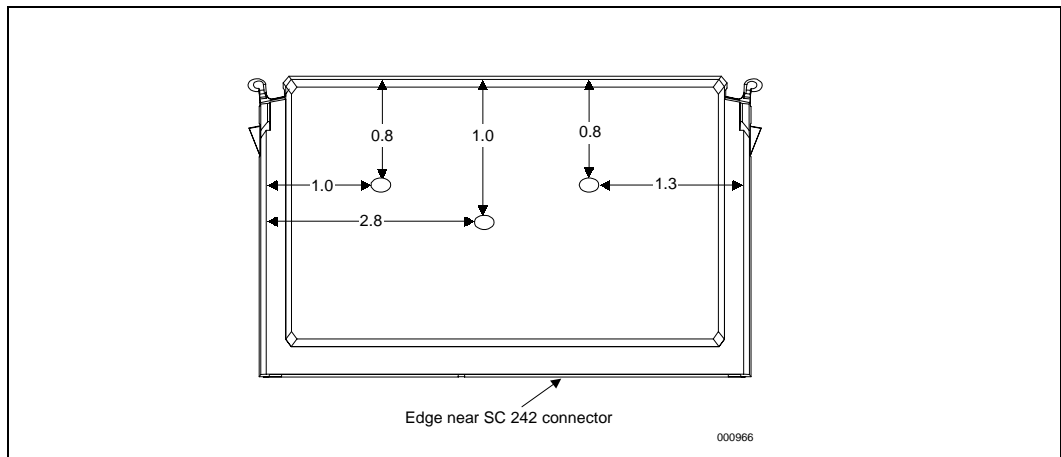
Figure 21. Guideline Locations for Cover Temperature ( T_{COVER} ) Thermocouple Placement
