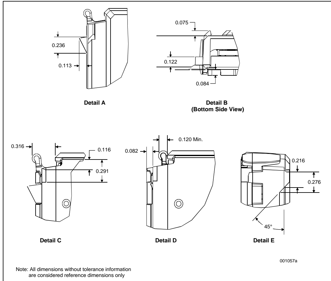
Figure 32. Pentium® II Processor S.E.C. Cartridge Latch Arm, Thermal Plate, and Cover Detail Dimensions (Reference Dimensions Only)
