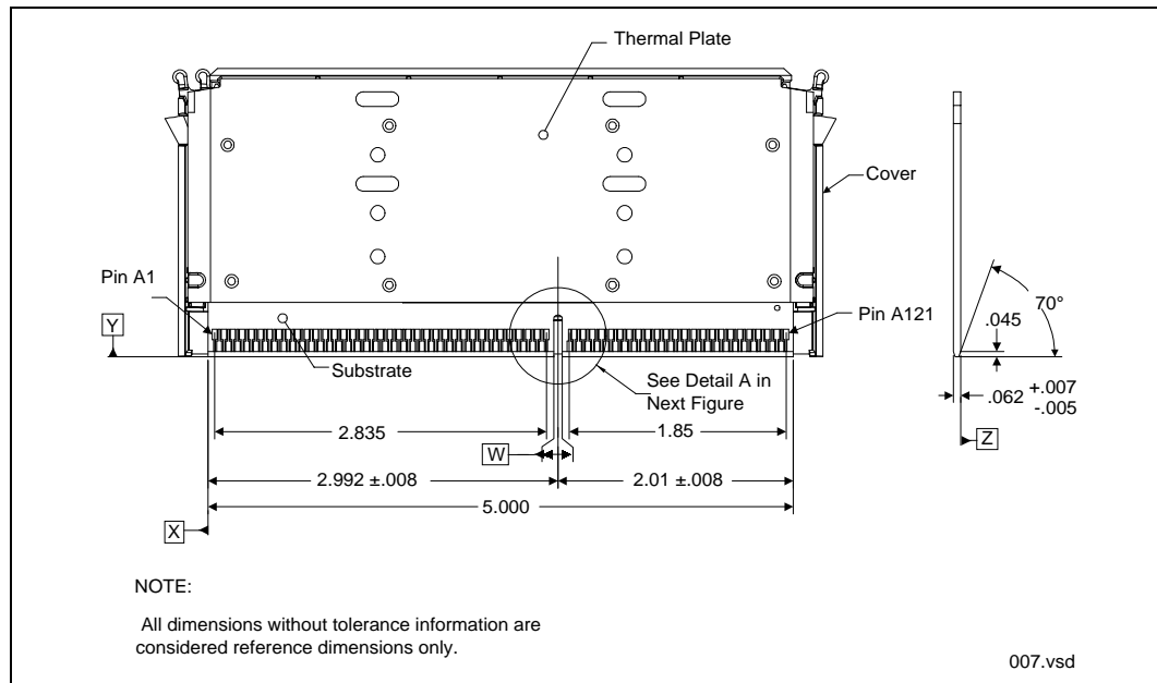
Figure 35. Pentium® II Processor Substrate—Edge Finger Contact Dimensions
