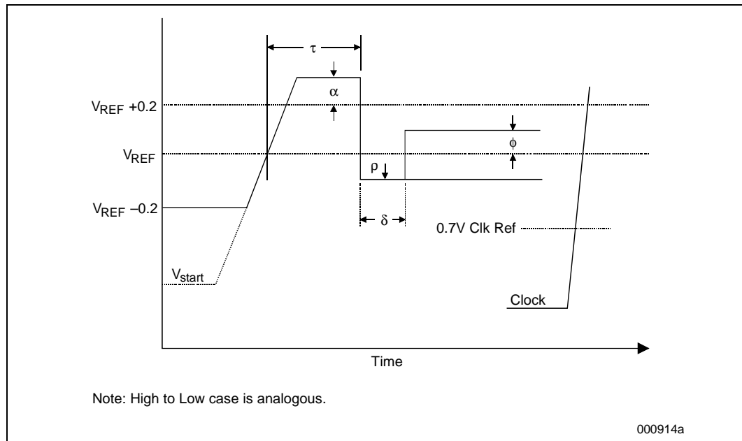
Figure 15. Low to High GTL+ Receiver Ringback Tolerance
