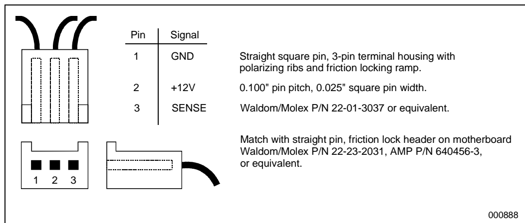
Figure 45. Boxed Processor Fan Heatsink Power Cable Connector Description
