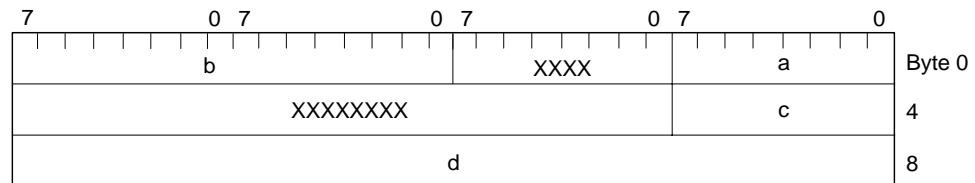
Figure 7-1 Natural Alignment
