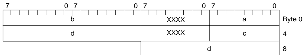
Figure 7-2 User-constrained Alignment
