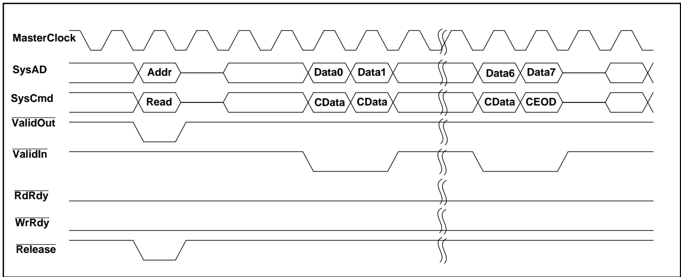
Figure 5: R4640 Block Read Request
