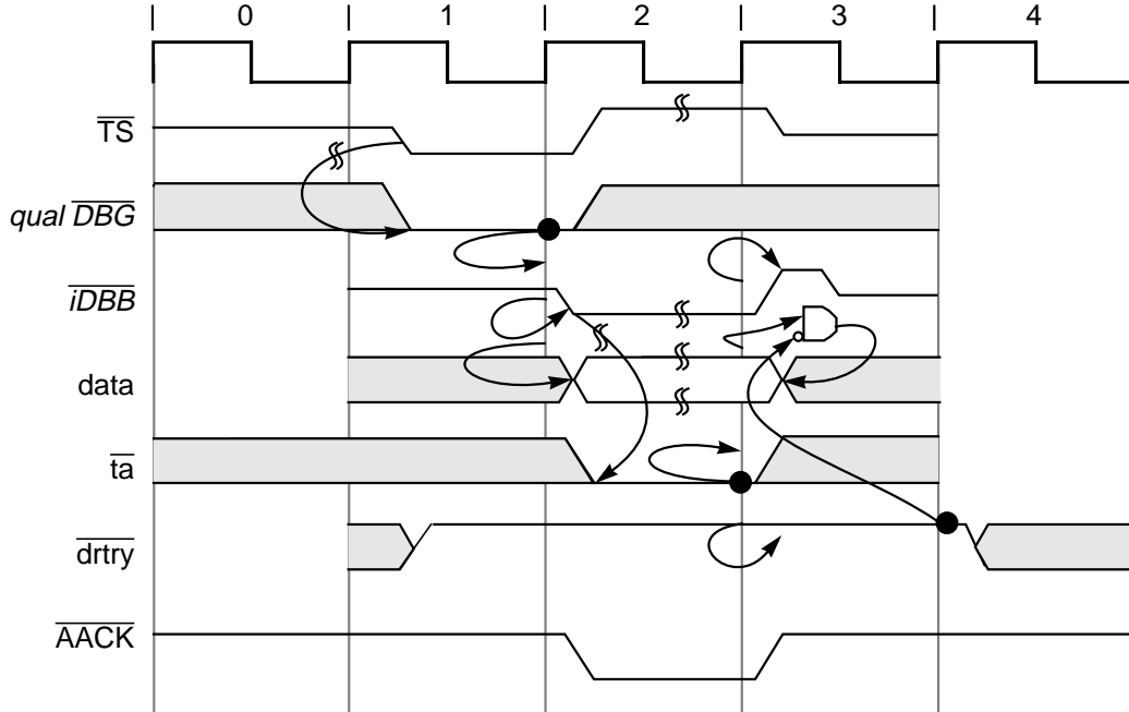
Figure 8-10. Normal Single-Beat Read Termination
