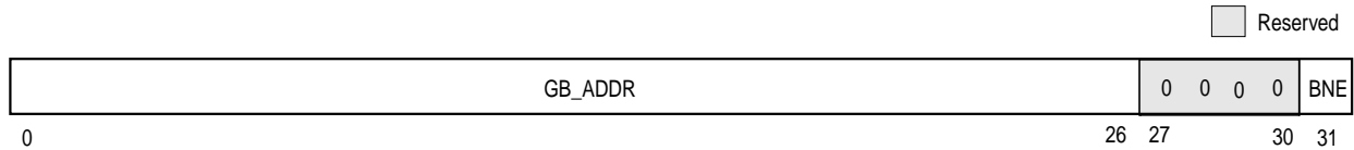
Figure 2-16. Write Pipe Address Register (WPAR)
