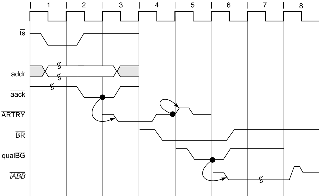
Figure 8-8. Snooped Address Cycle with \overline{\text{ARTRY}}
