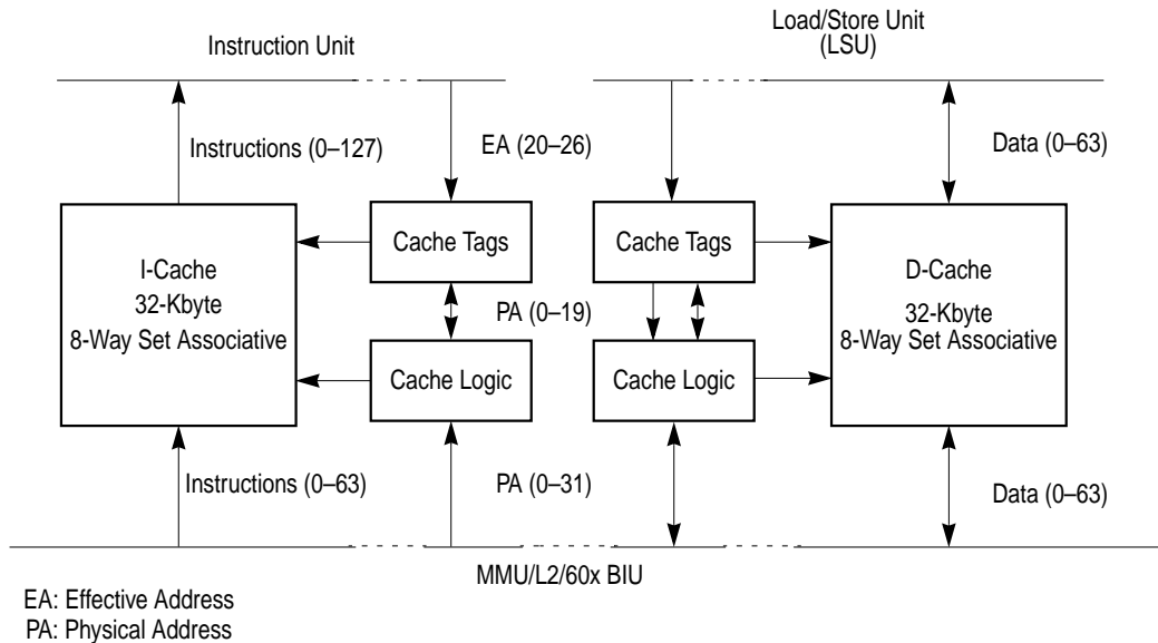
Figure 3-1. Cache Integration
