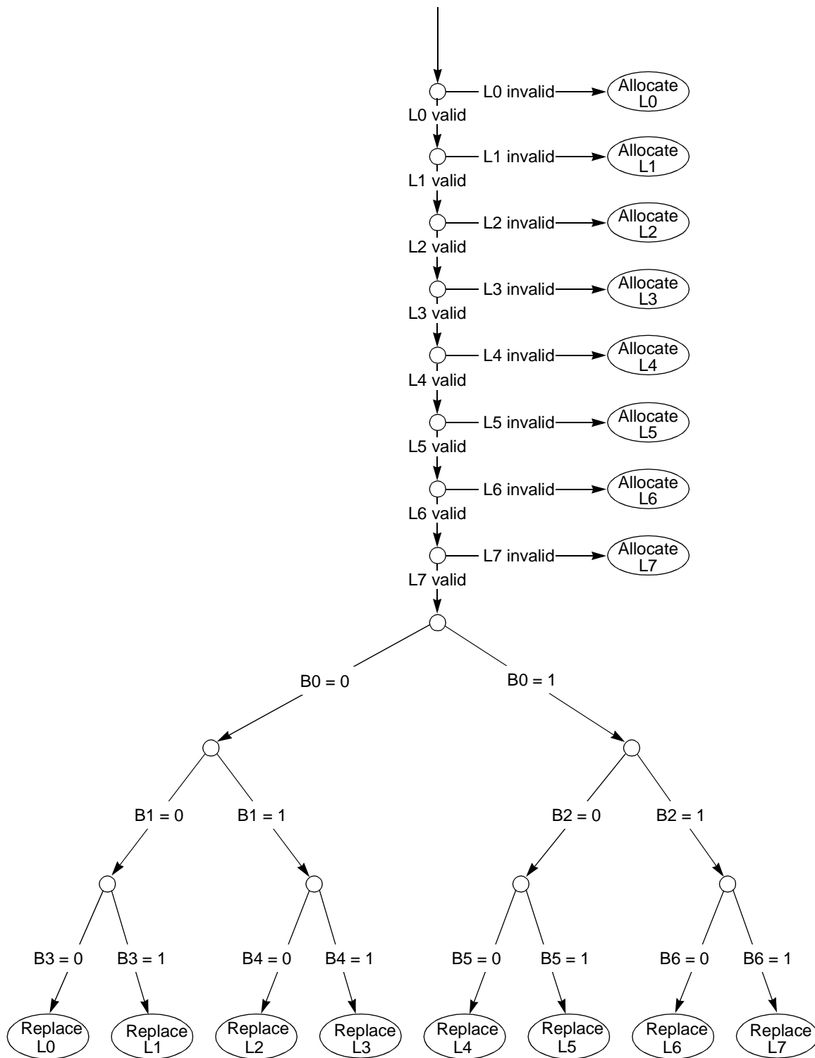
Figure 3-5. PLRU Replacement Algorithm
