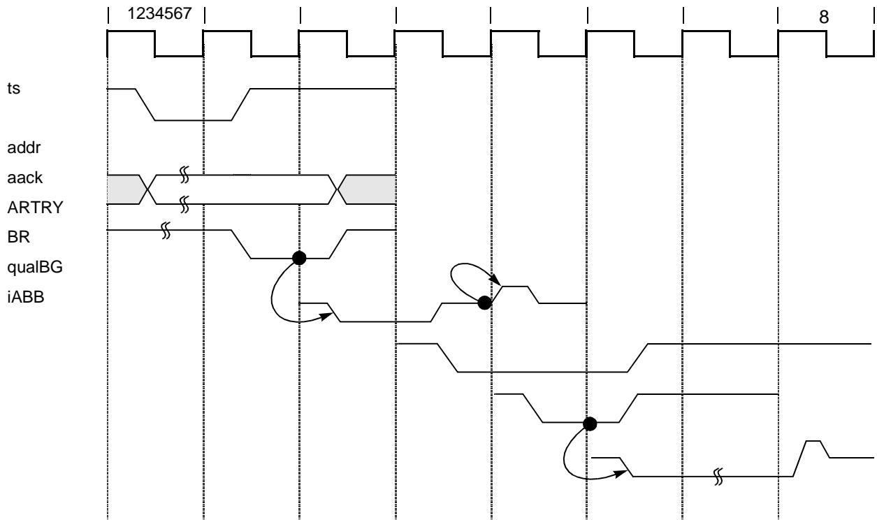
Figure 8-8. Snoop Address Cycle with \overline{\text{ARTRY}}
