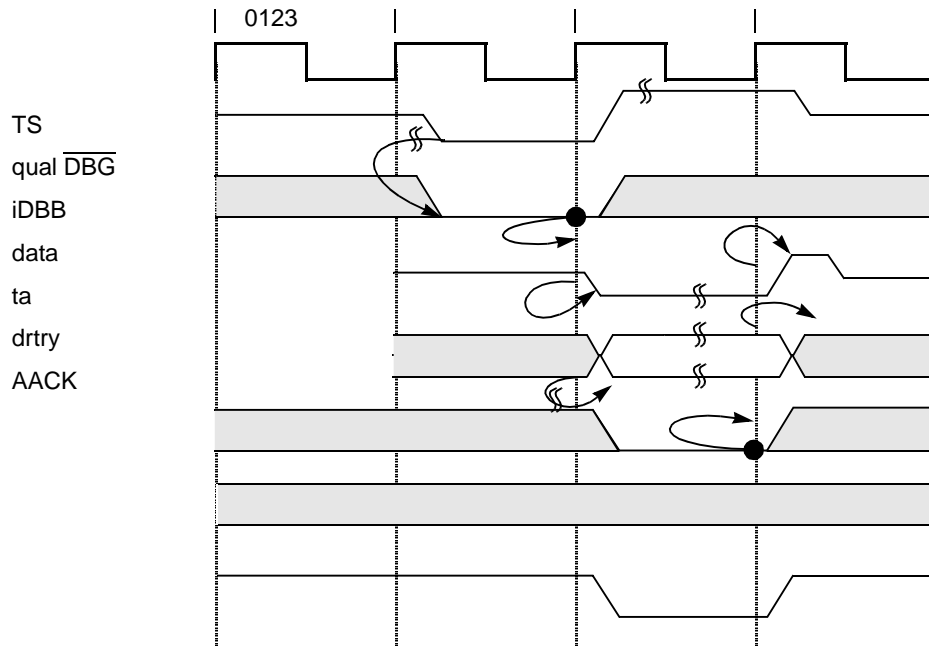
Figure 8-11. Normal Single-Beat Write Termination
