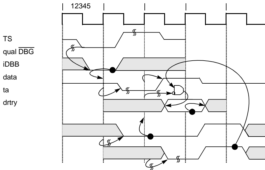
Figure 8-13. Termination with \overline{\text{DRTRY}}
