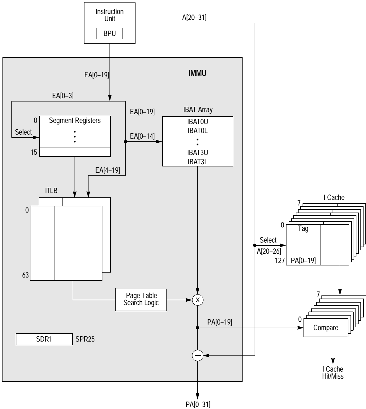
Figure 5-2. PowerPC 750CX/CXe/CXr Microprocessor IMMU Block Diagram
