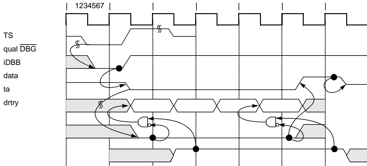
Figure 8-12. Normal Burst Transaction
