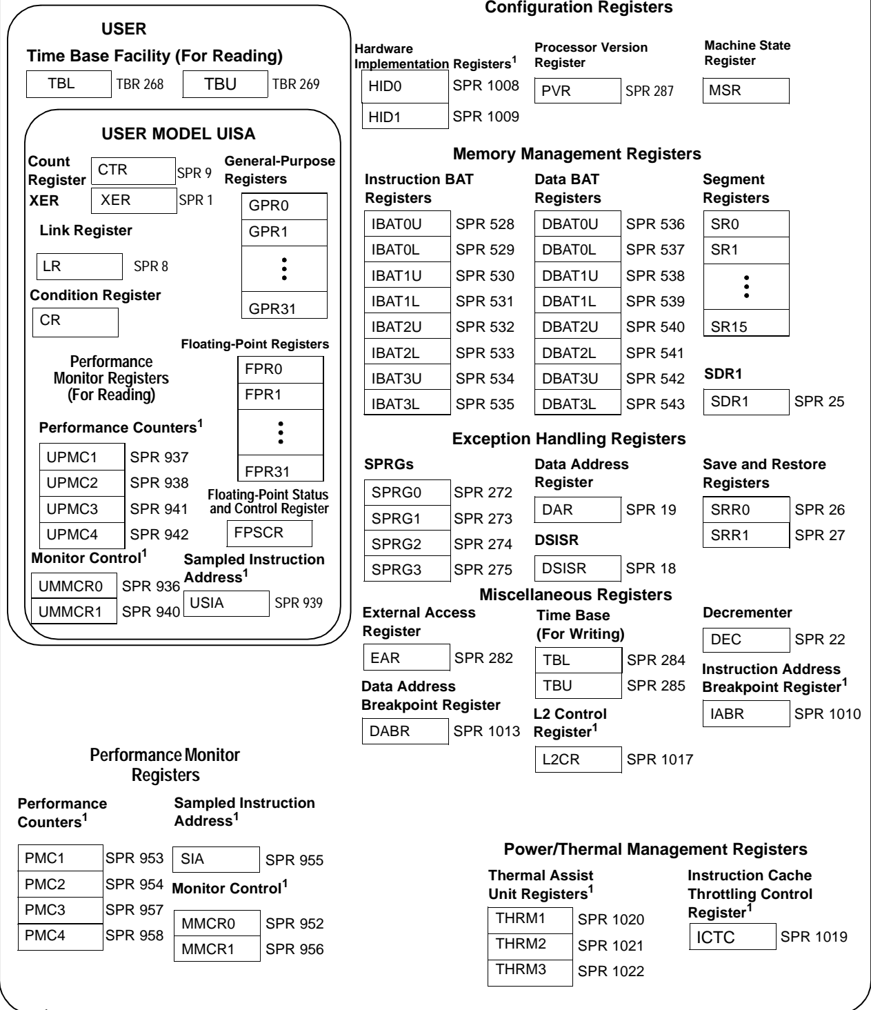
Figure 1-5. 750CX/CXe/CXr Microprocessor Programming Model—Registers
