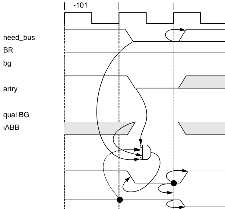
Figure 8-6. Address Bus Arbitration Showing Bus Parking
