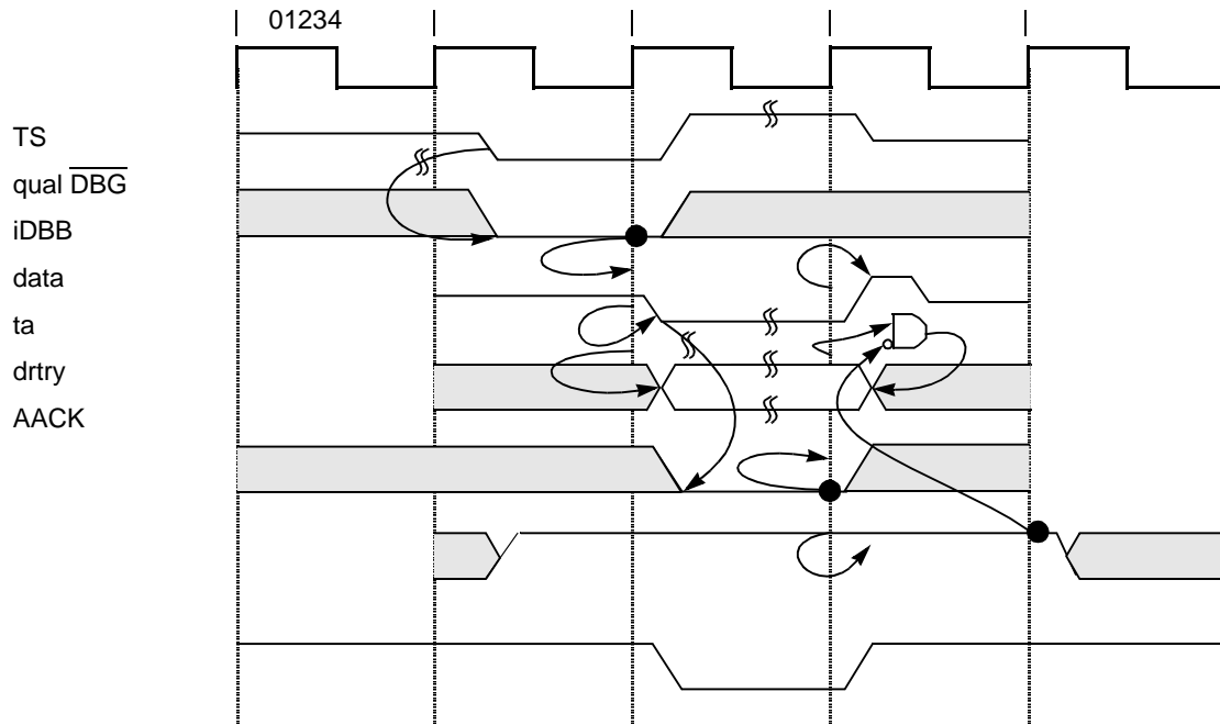
Figure 8-10. Normal Single-Beat Read Termination
