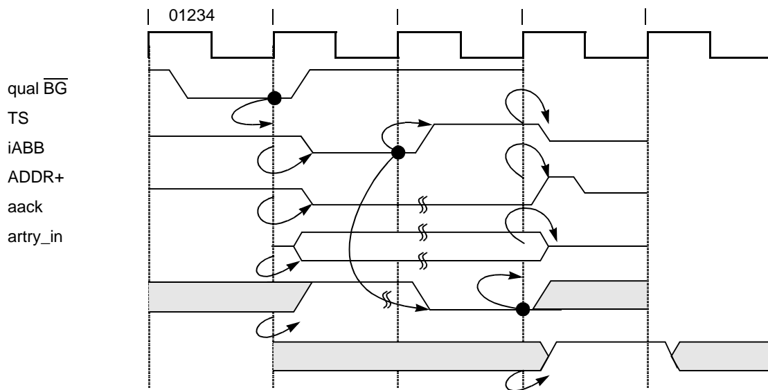
Figure 8-7. Address Bus Transfer
