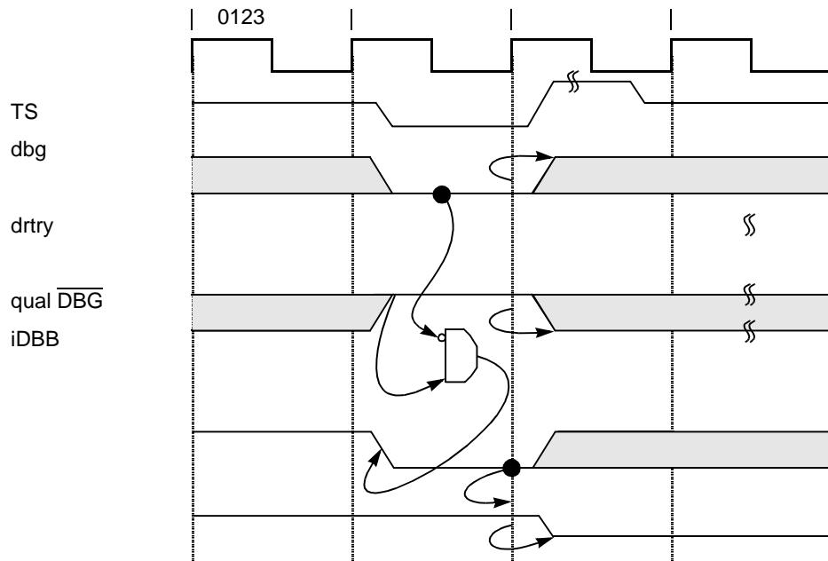
Figure 8-9. Data Bus Arbitration
