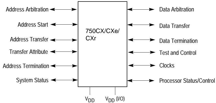
Figure 1-3. System Interface
