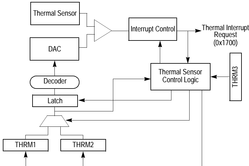
Figure 10-1. Thermal Assist Unit Block Diagram
