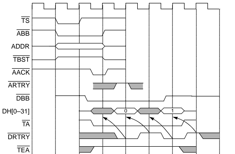
Figure 8-23. 32-Bit Data Bus Transfer (Two-Beat Burst with DRTRY)
