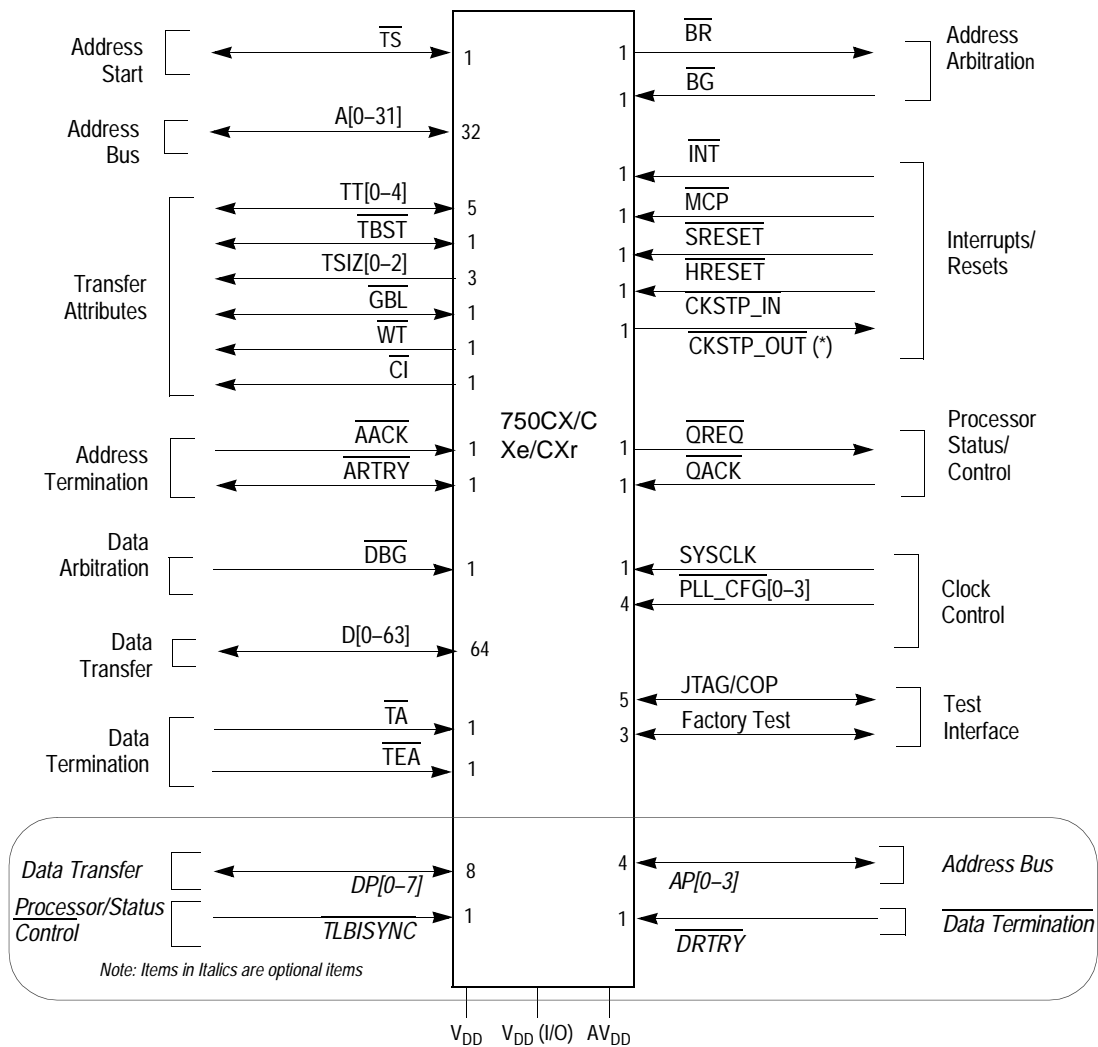
Figure 7-1. PowerPC 750CX/CXe/CXr Signal Groups
