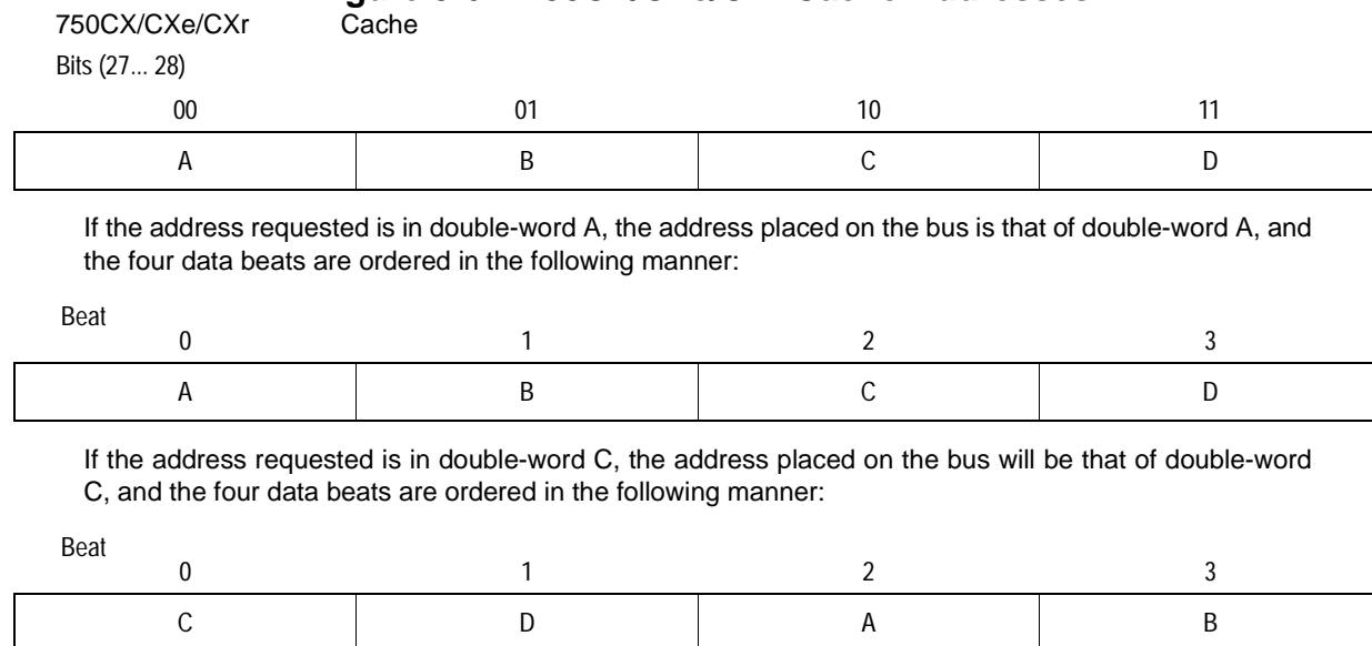
Figure 3-6. 750CX/CXe/CXr Cache Addresses
