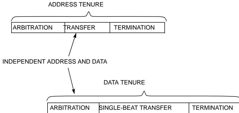
Figure 8-4. Overlapping Tenures on the 750CX/CXe/CXr Bus for a Single-Beat Transfer
