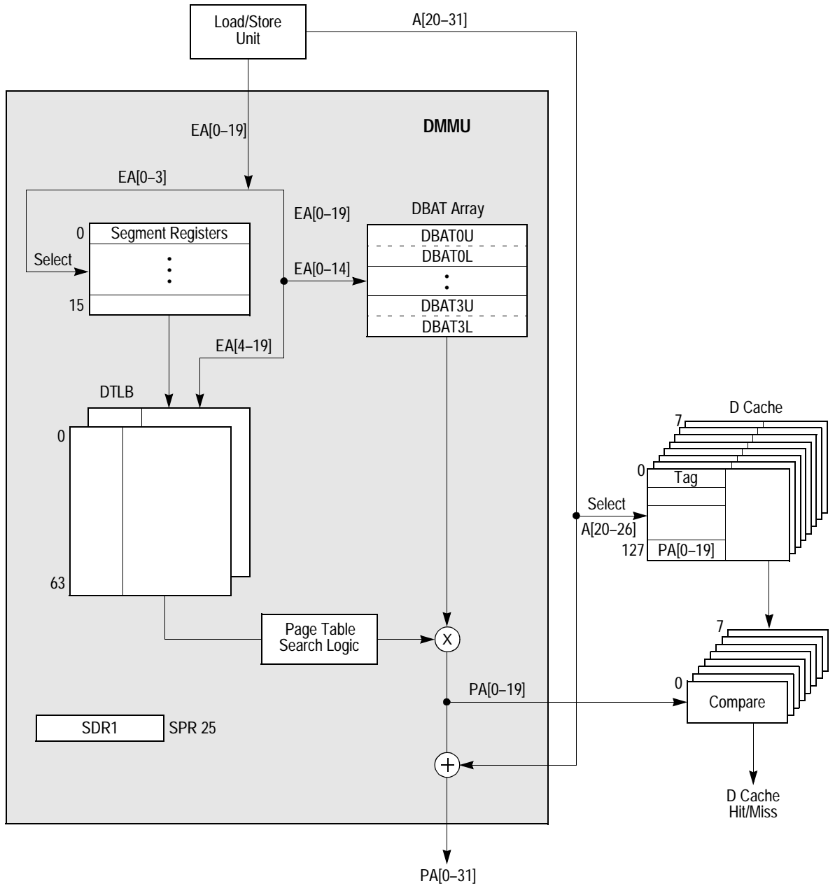
Figure 5-3. The 750CX/CXe/CXr Microprocessor DMMU Block Diagram
