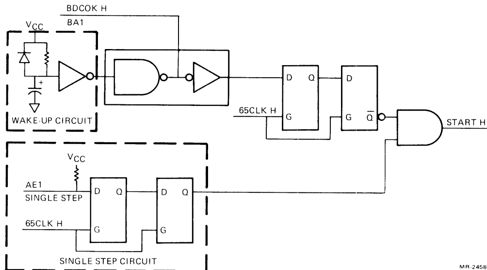
Figure 5-7 Clock Generator Initialization Circuitry
