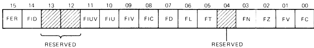
Figure 9-4 Floating Point Status Register
