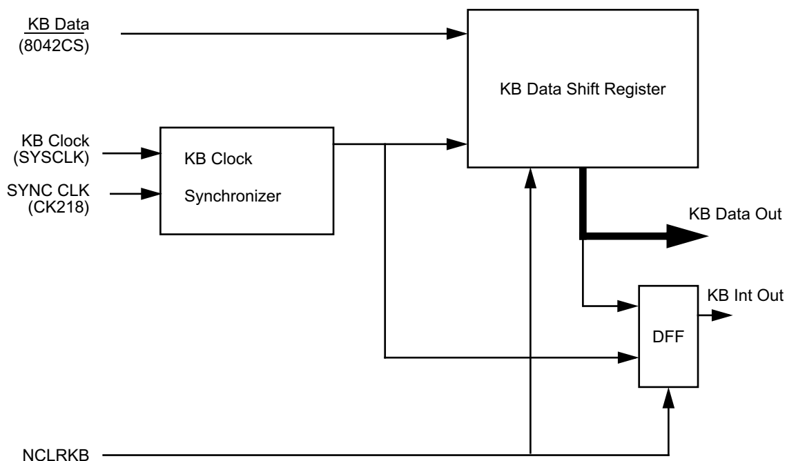
Figure B-1 XT Keyboard Block Diagram
