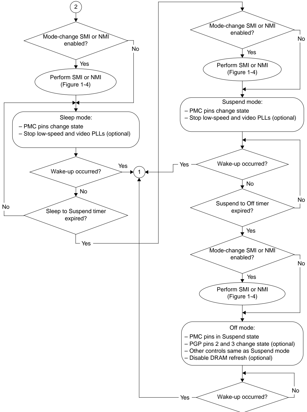
Figure 1-3 State Transition Flowchart (continued)
