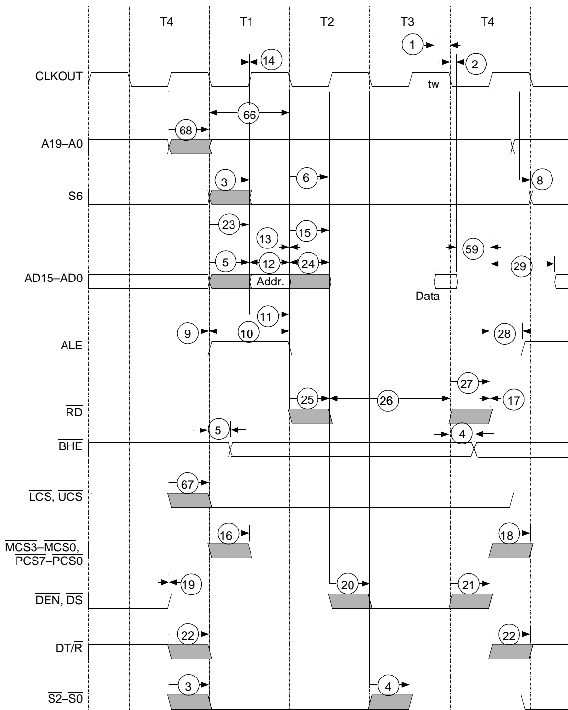
Figure 14. Read Cycle Waveforms
