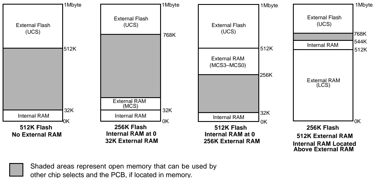
Figure 11. Example Memory Maps
