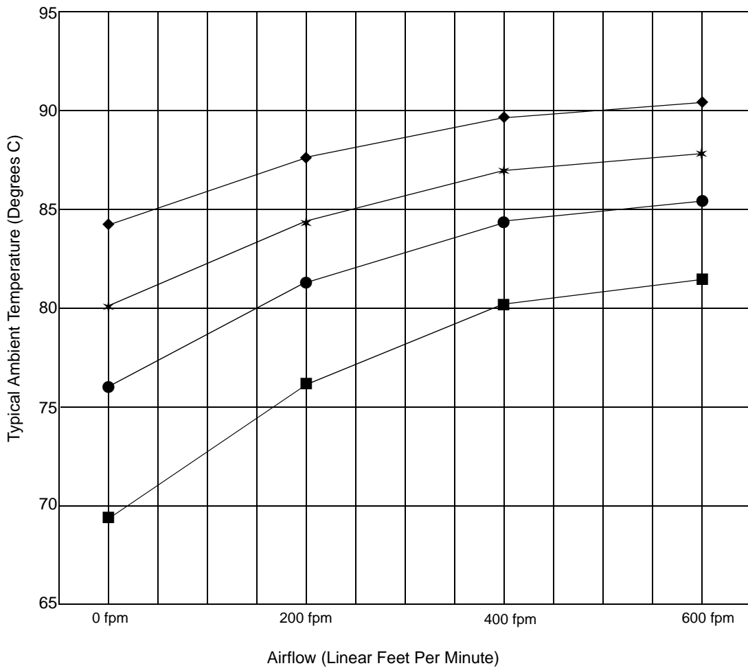
Figure 18. Typical Ambient Temperatures for TQFP with 2-Layer Board
