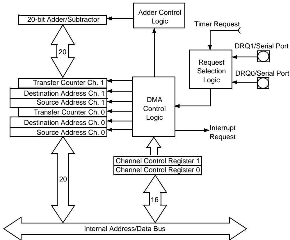
Figure 12. DMA Unit Block Diagram
