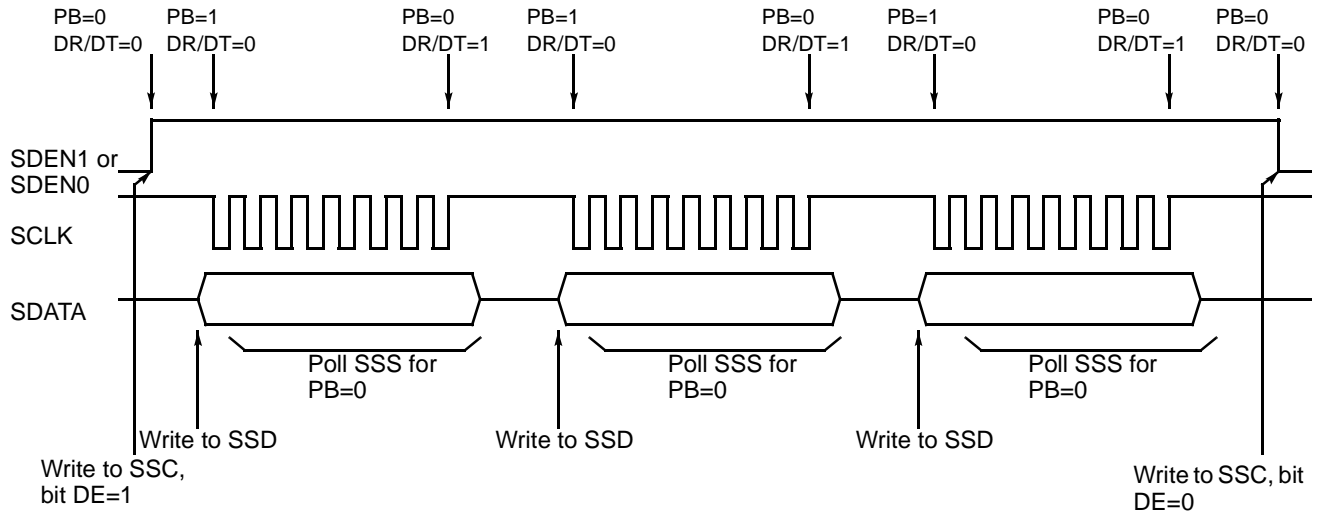
Figure 13. Synchronous Serial Interface Multiple Write
