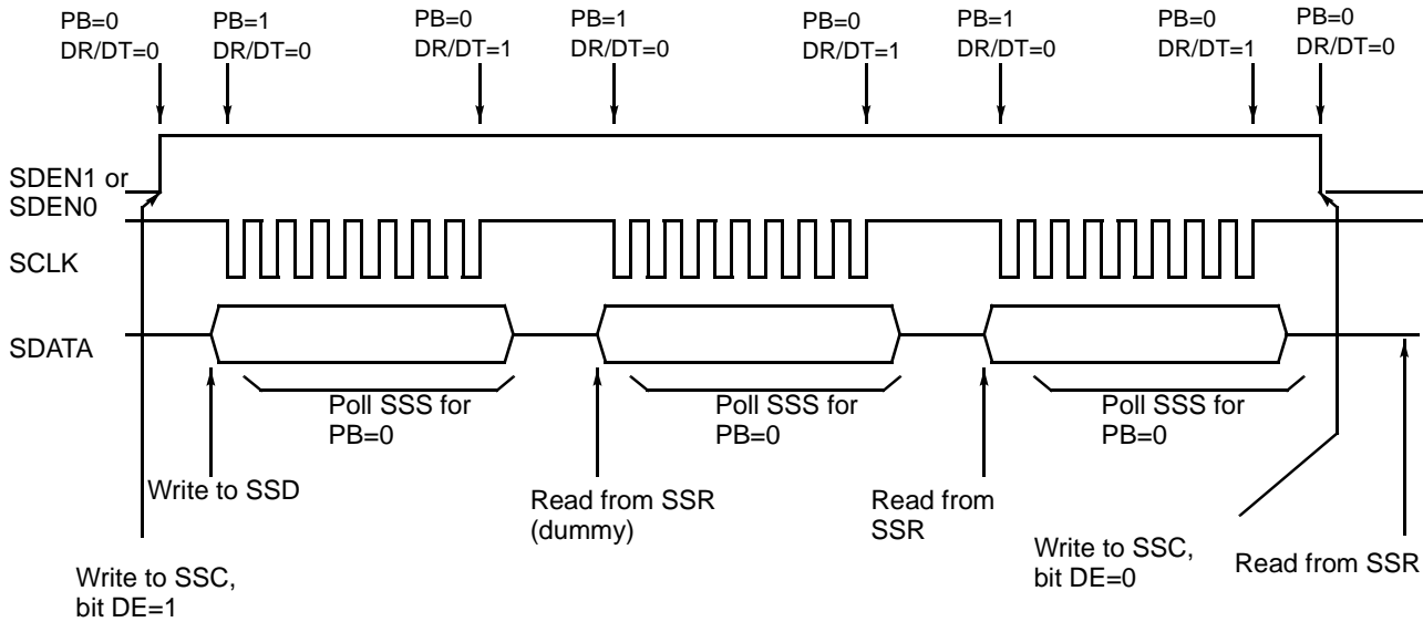
Figure 14. Synchronous Serial Interface Multiple Read
