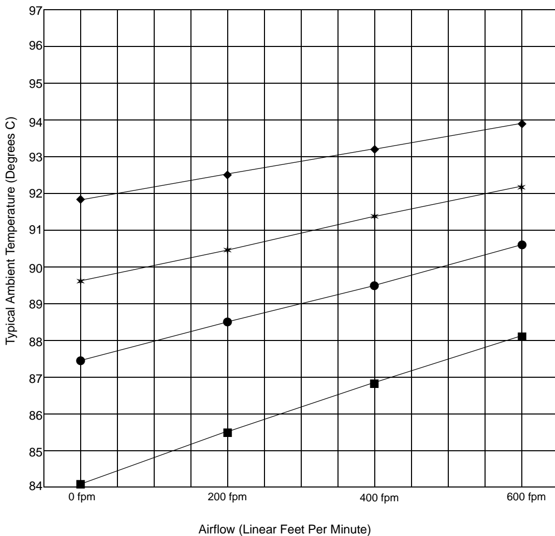
Figure 20. Typical Ambient Temperatures for TQFP with 4-Layer to 6-Layer Board
