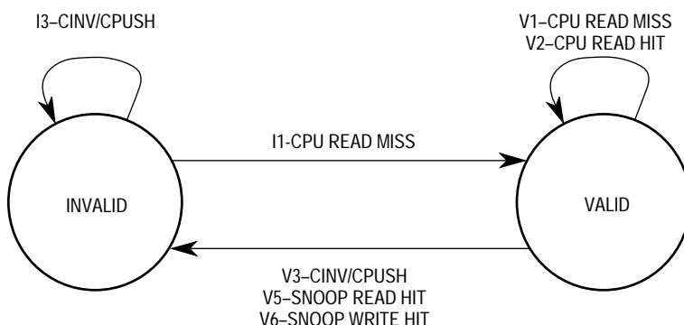
Figure 4-4. Instruction-Cache Line State Diagram
