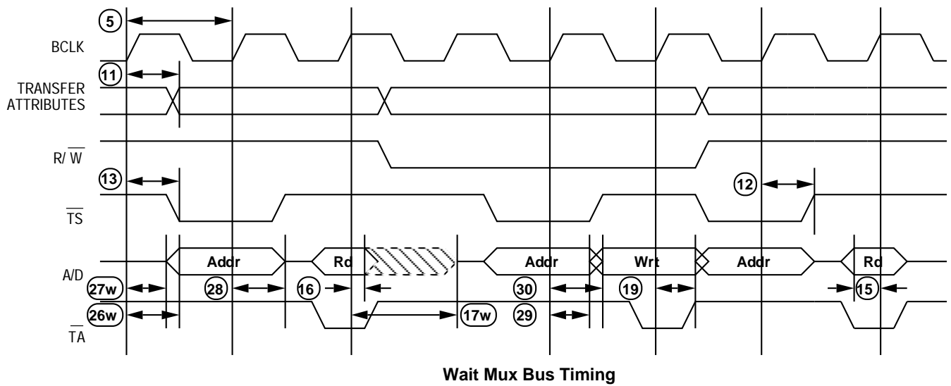
Figure 10-3. Read/Write Timing
