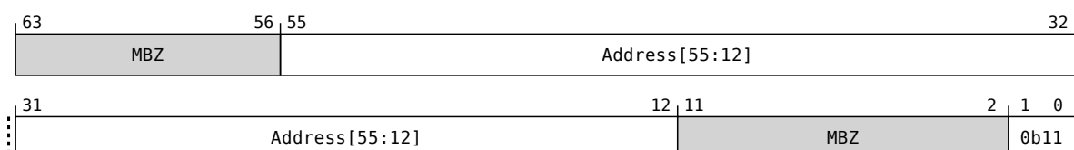
Figure 3.16: Level 0 Table entry
