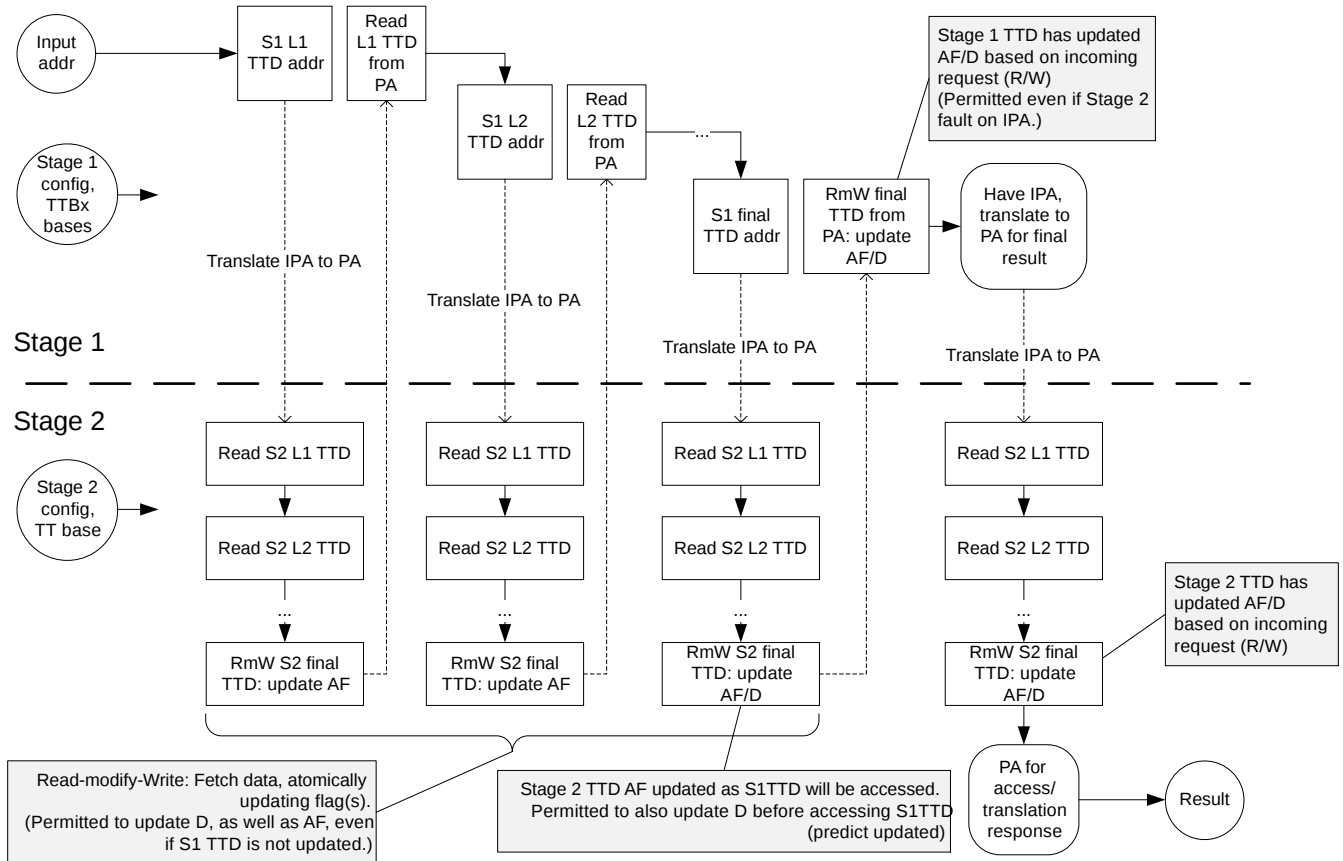
Figure 3.11: Example Hardware flag update with nested translation
