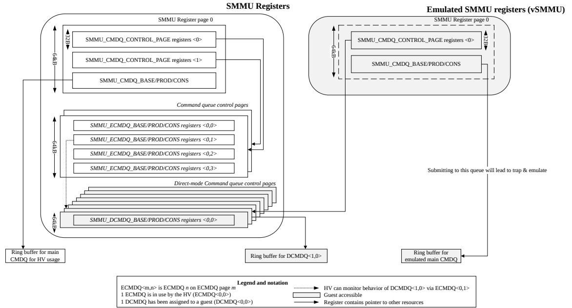
Figure 3.9: Example DCMDQ configuration
