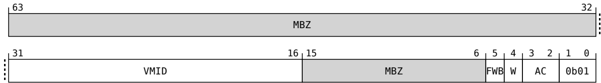
Figure 3.15: Level 0 Block entry
