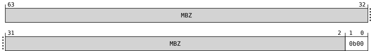
Figure 3.14: Level 0 No Access entry
