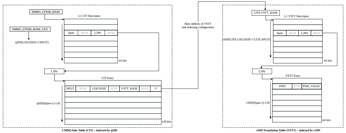
Figure 3.10: Table walks during SID translation
