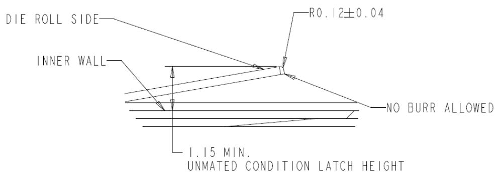
Figure 4-24: Latch flap, cross-sectional view from top
