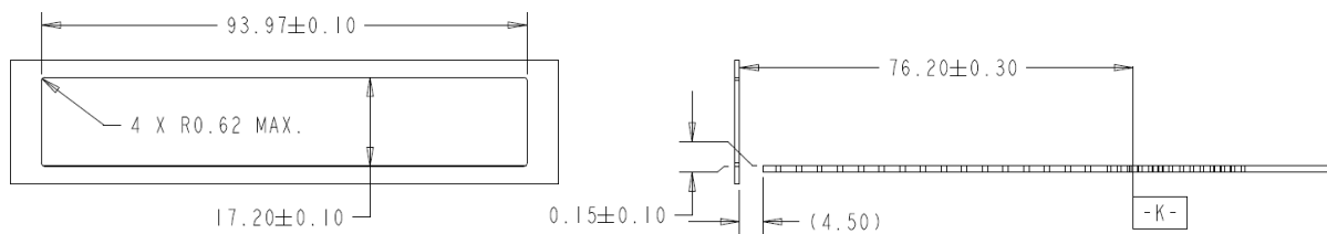
Figure 4-27: Bezel design for 1x4 cage
