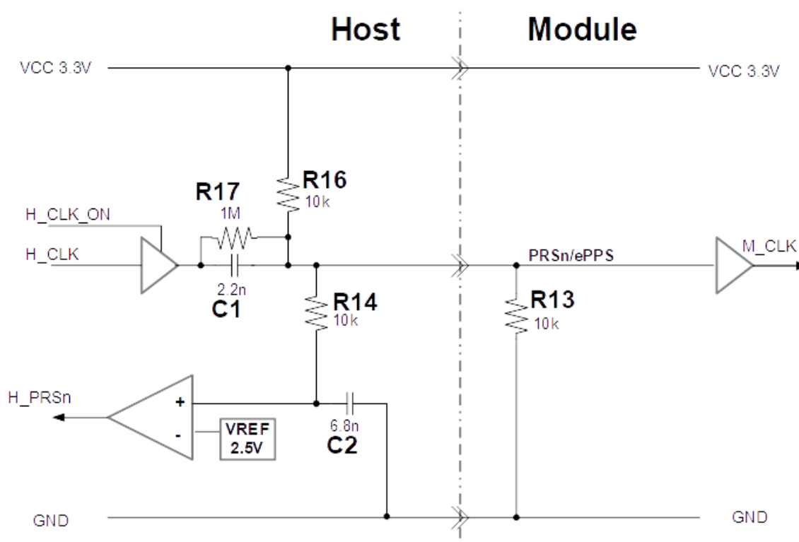
Figure 10-7: PRSn/ePPS circuit
