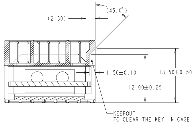
SECTION KEYING-KEYING
