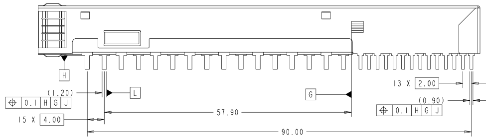
Figure 8-16: Cage positioning pins and forward stop
