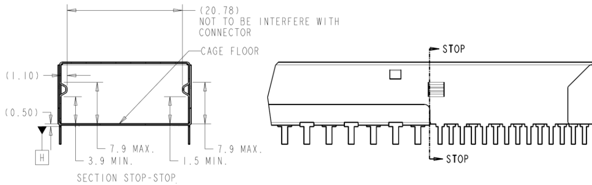
Figure 8-18: Stop feature in OSFP-XD-RHS cage
