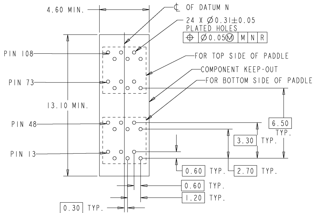
DETAIL CHF-A
