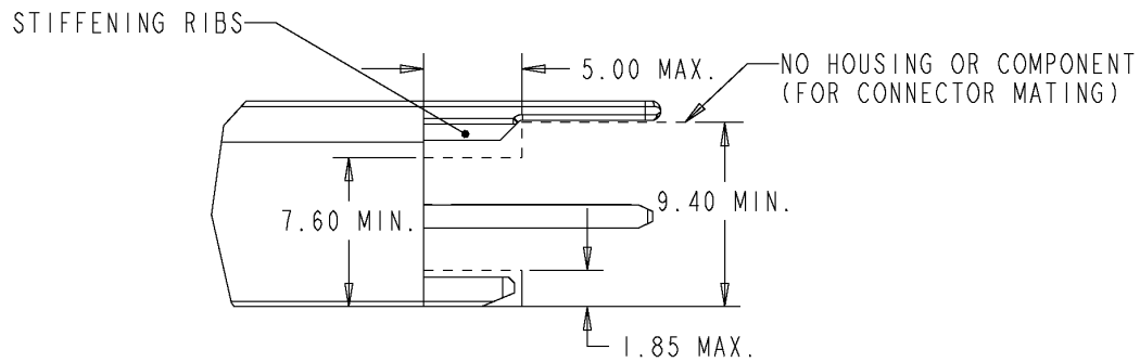
Figure 8-6: Connector keepout area from the side view
