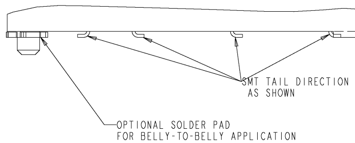
Figure 4-30: Surface mount connector, from the side view
