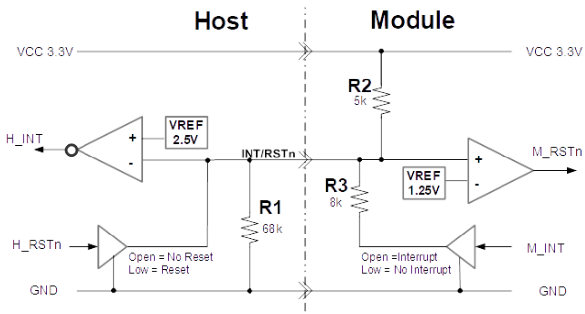
Figure 10-3: INT/RSTn circuit
