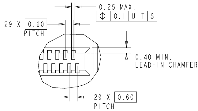
DETAIL CONTACT
