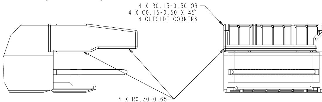
Figure 3-5: OSFP-XD corner radius
