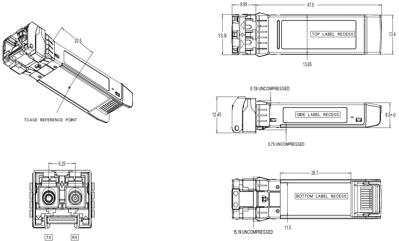
Figure 7: Module Drawing
