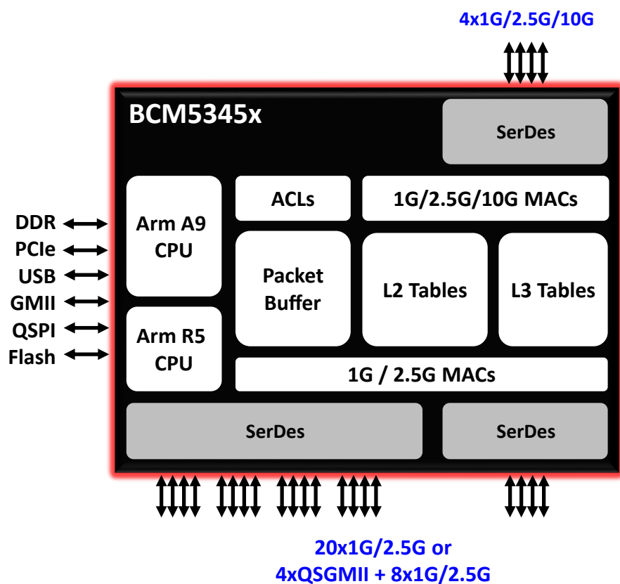
Figure. BCM5345X Block Diagram
