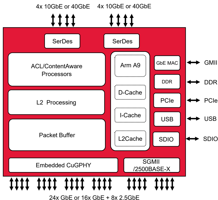
Figure. BCM53440 Block Diagram
