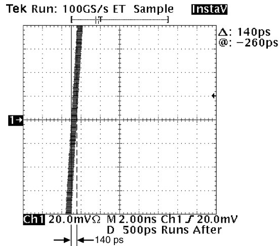
FIGURE 8. Typical Jitter Measured at the Jtxout in IEEE 802.3 Gigabit Test Mode 2 on a Compliant GPHY Device. The Captured is the Rising Edge of the Test Mode 2 Waveform.
