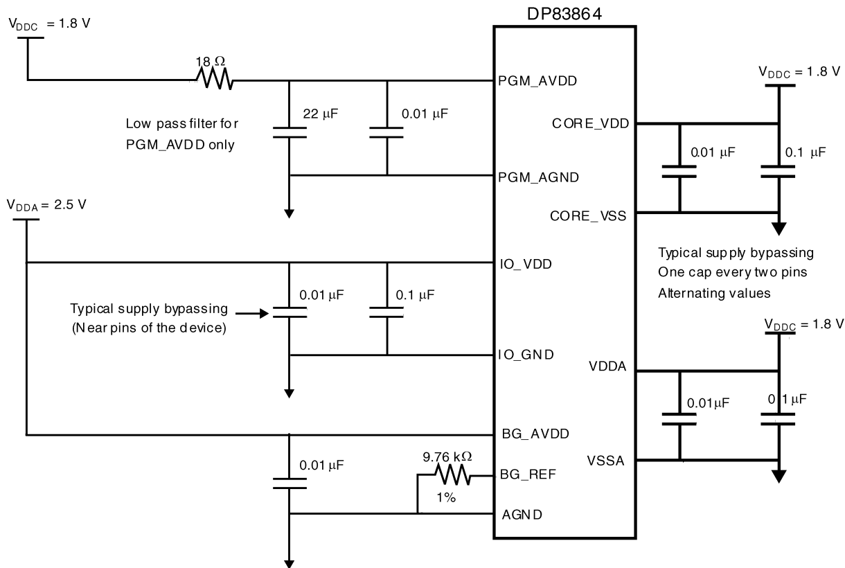
FIGURE 6. GPHY Power Supplies and Bandgap Voltage
