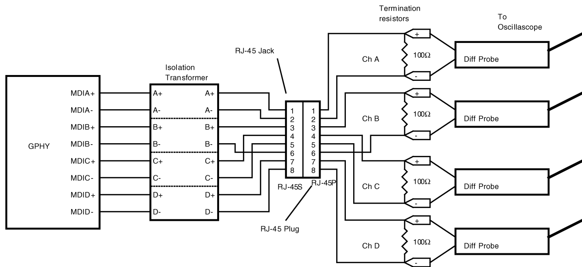
FIGURE 7. IEEE Gigabit Test Mode 2. (Simplified Diagram)
