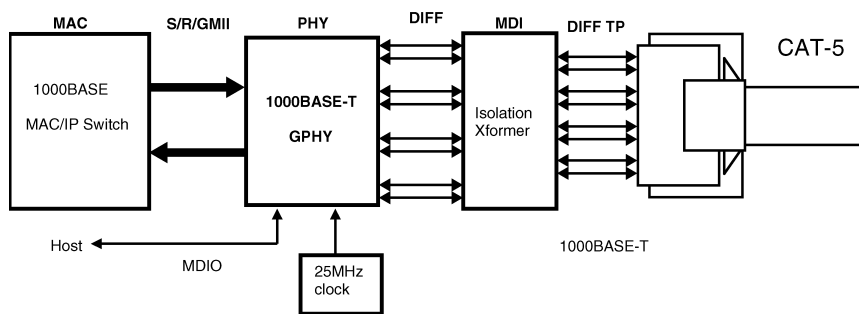
FIGURE 1. GPHY Block Diagram
