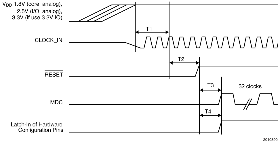
FIGURE 3. Reset timing. T1 = 0+ \mu s; T2 = 150 \mu s; T3 = T4 = 20 ms
