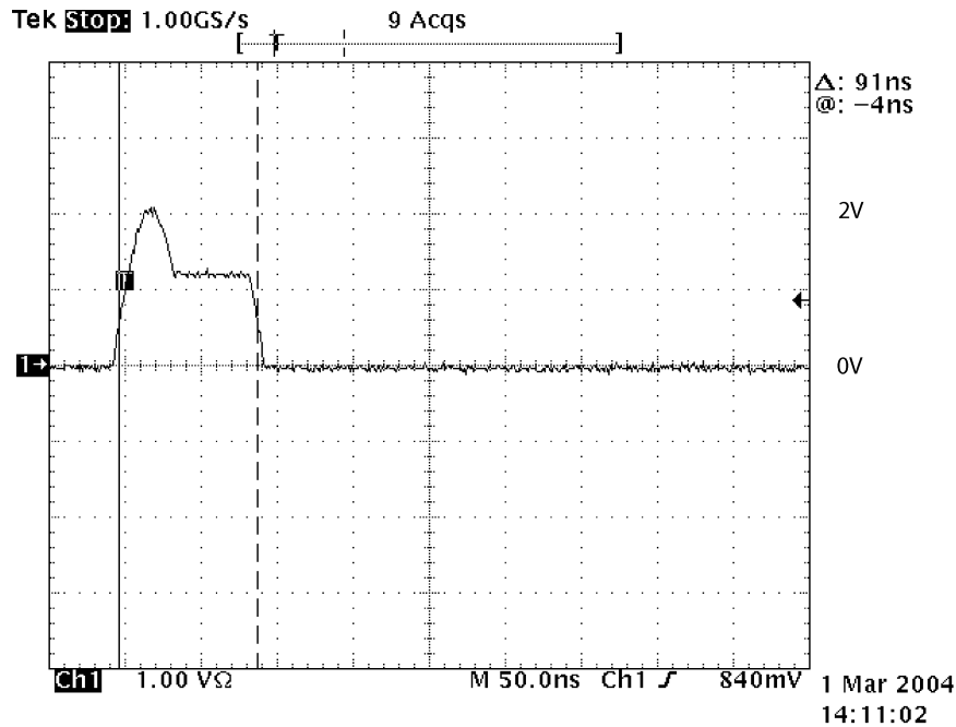
FIGURE 5. Auto-negotiation Link Pulse
