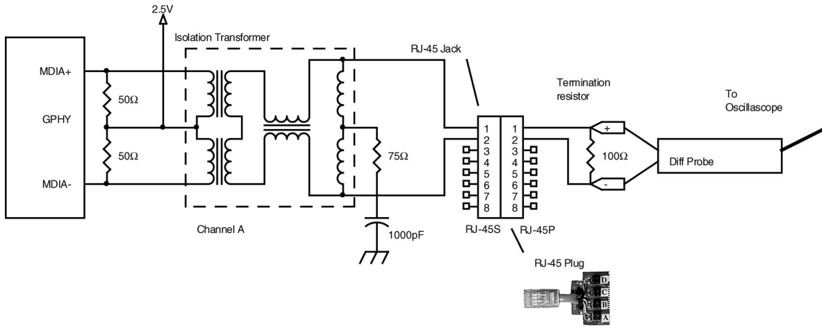
FIGURE 4. Link Pulse Test On Channel A
