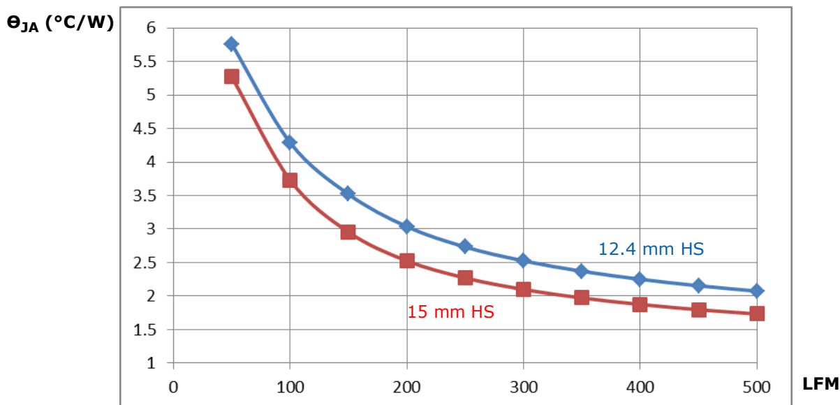
Figure 15-3. X710/XXV710/XL710 \theta_{JA} ( ^{\circ}\text{C/W} ) vs. air flow @ 10 W (JEDEC card)
