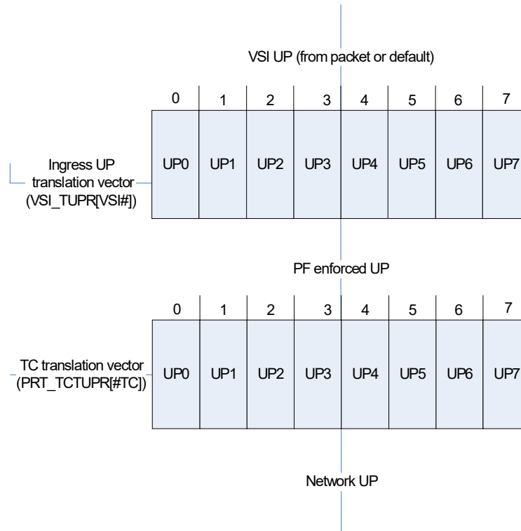
Figure 7-8. Example: Non-VLAN aware, non-DCB aware operating system
