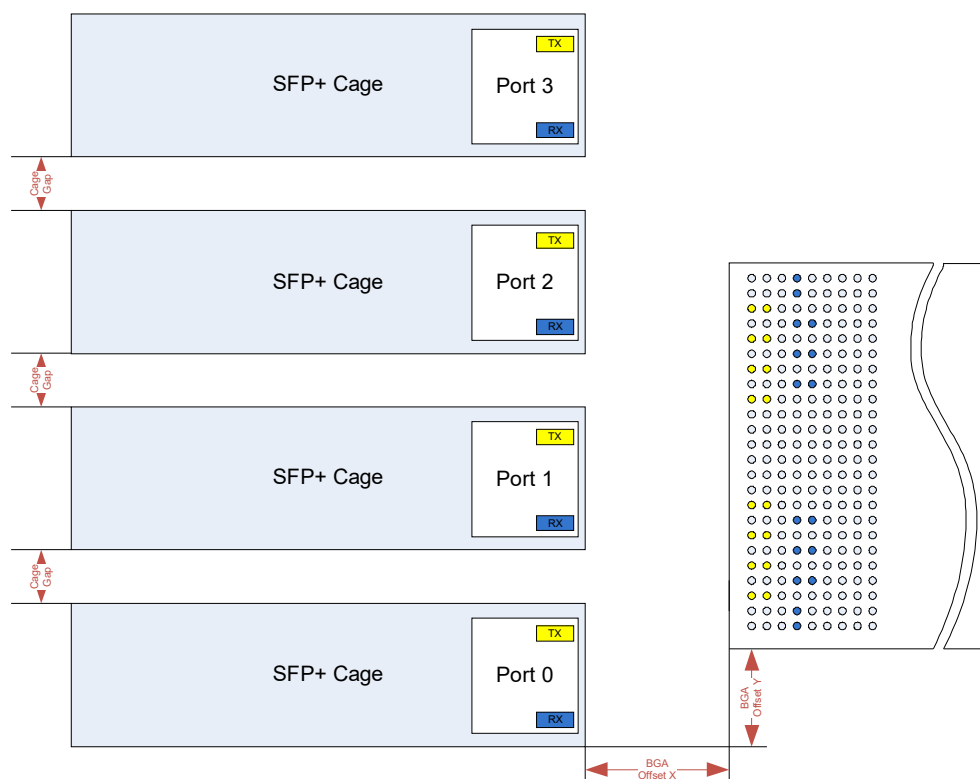
Figure 14-17. Component Placement
