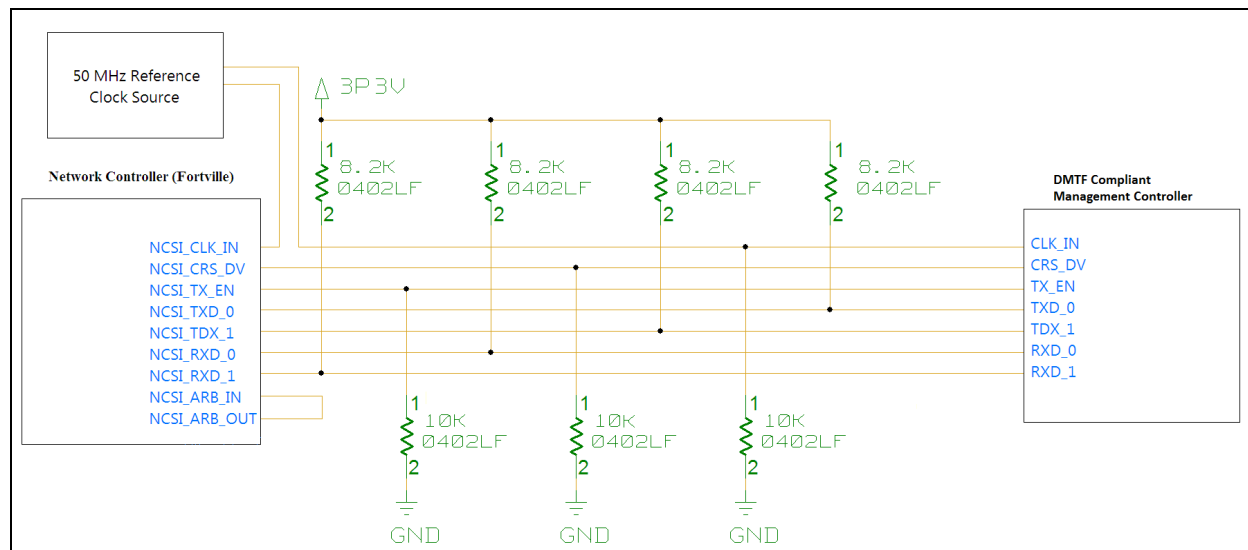
Figure 14-4. NC-SI Connection Schematic: Single-Drop Configuration
