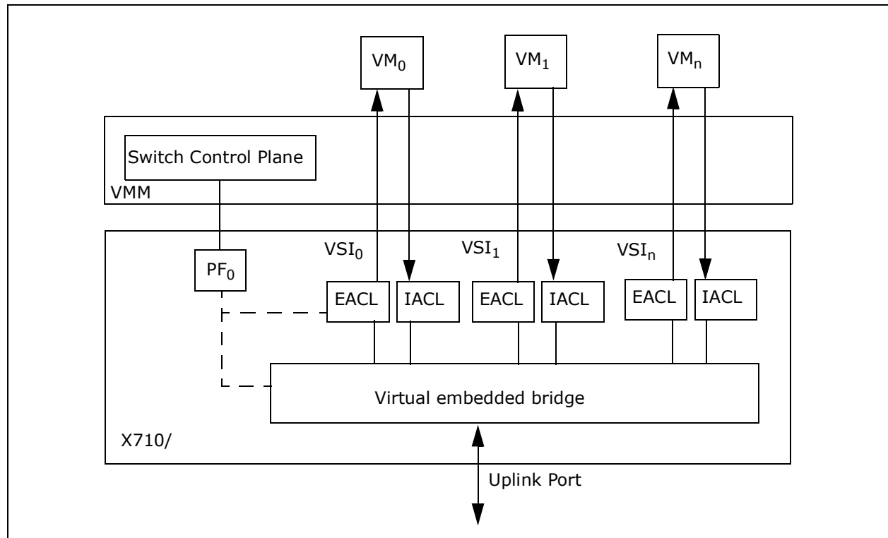
Figure 7-49. Switch control plane
