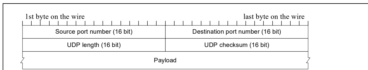
Figure 7-21. UDP packet format
