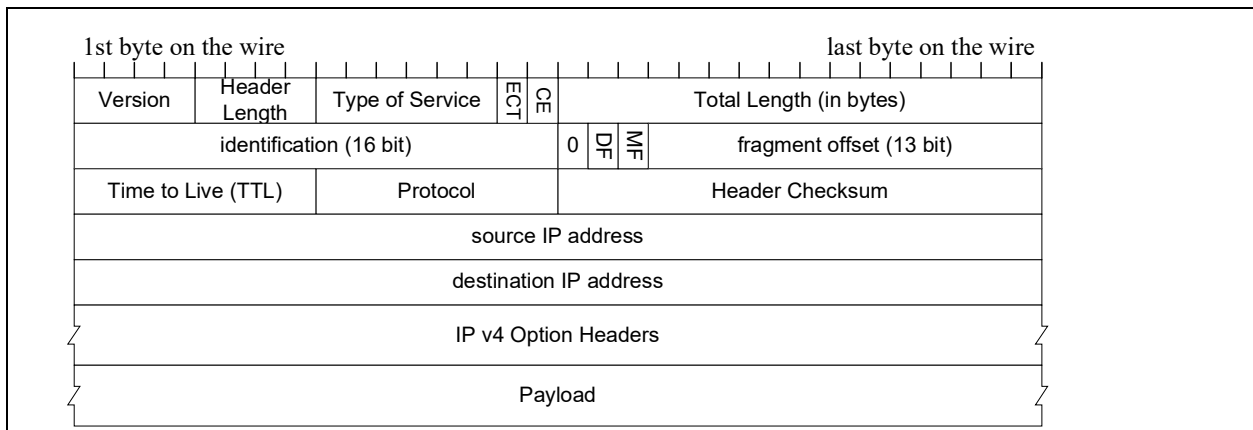
Figure 7-13. IPv4 datagram
