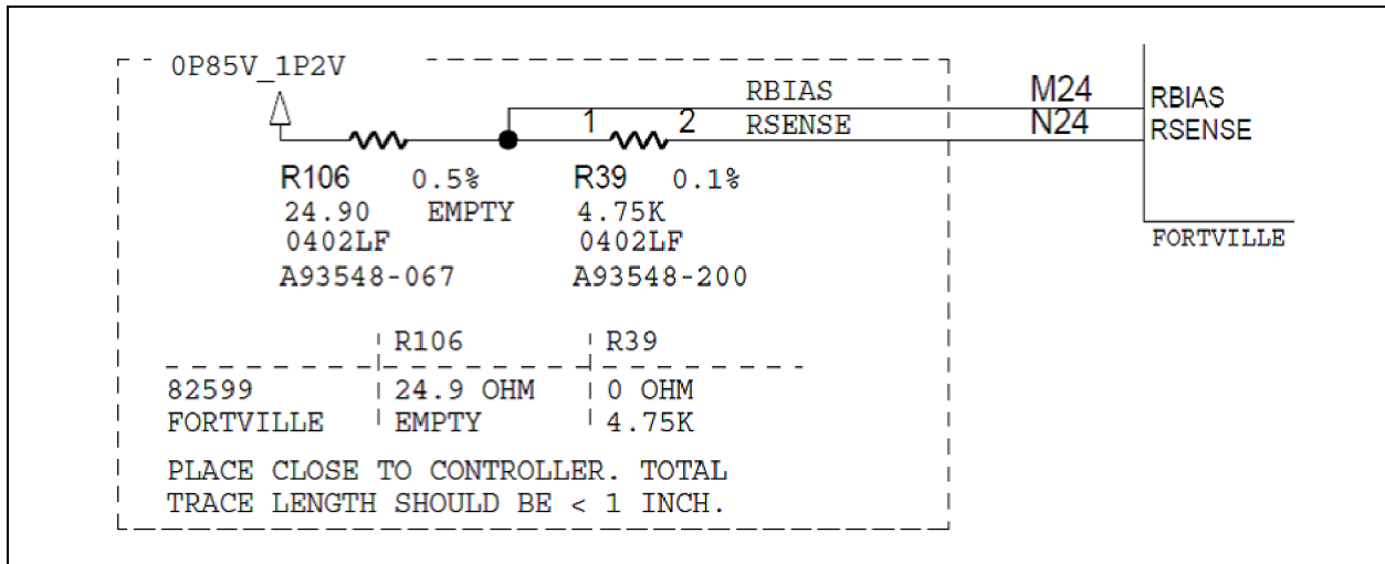
Figure 13-23. X710/XXV710/XL710 Bias Circuit
