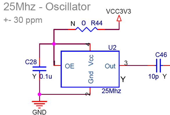
Figure 10. Reference Oscillator Circuit
