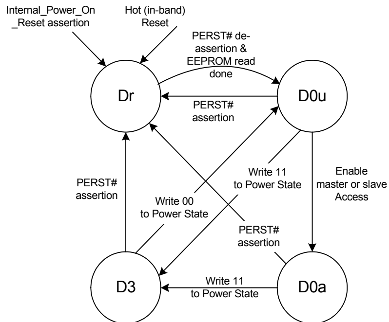
Figure 7. Power Management State Diagram
