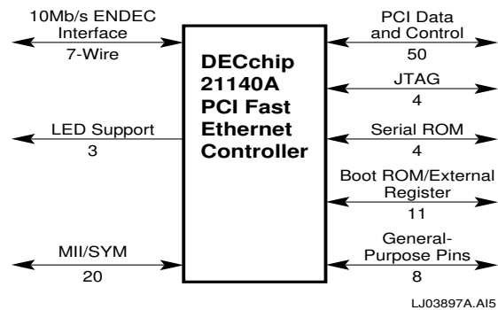
Figure 1 DECchip 21140A Pin Interface
