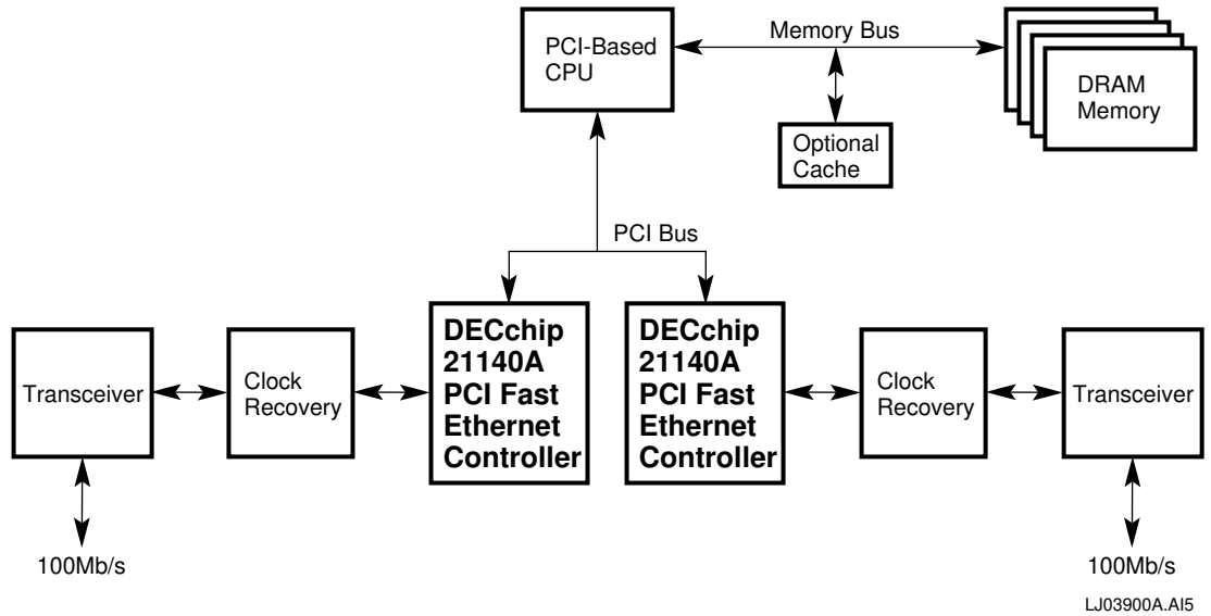
Figure 4 Fast Ethernet, 2-Port Bridge
