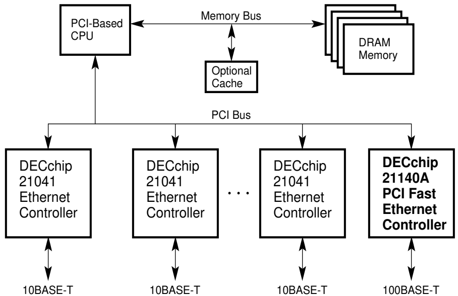
Figure 3 PCI-Based Bridge and Switch
