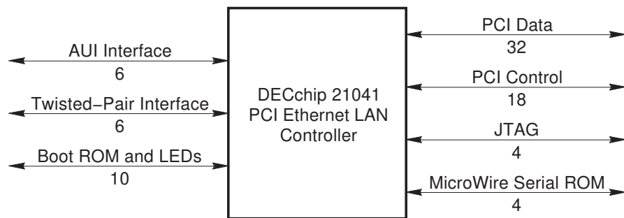
Figure 1 DECchip 21041 Pin Interface
