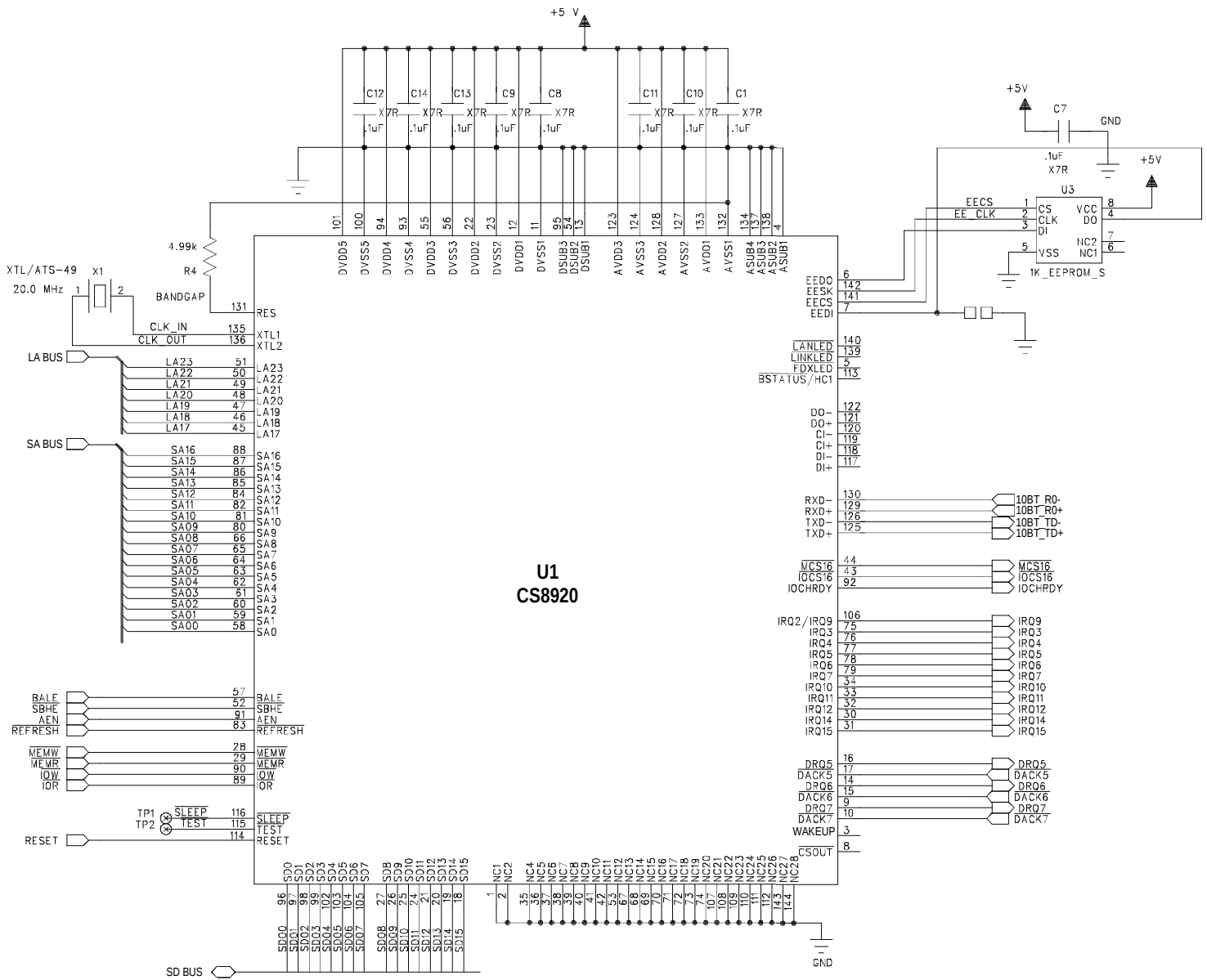
Figure 2.1.2. Overall Schematic
