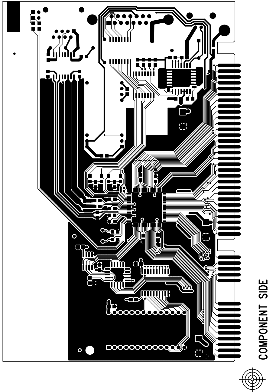
Figure 2.2.2. Ground connection. Top layer of two-layer Combo Card
