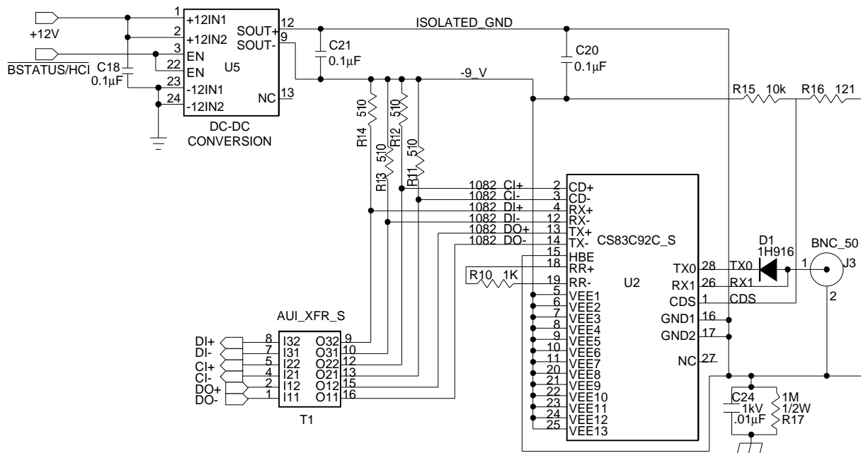
Figure 2.2.7. 10BASE-2 Schematic
