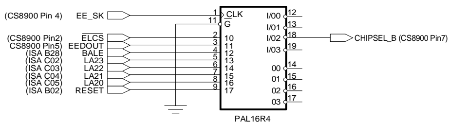
Figure 2.2.8 PAL Decode of LA[20-23]
