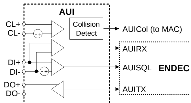
Figure 3.12. AUI
