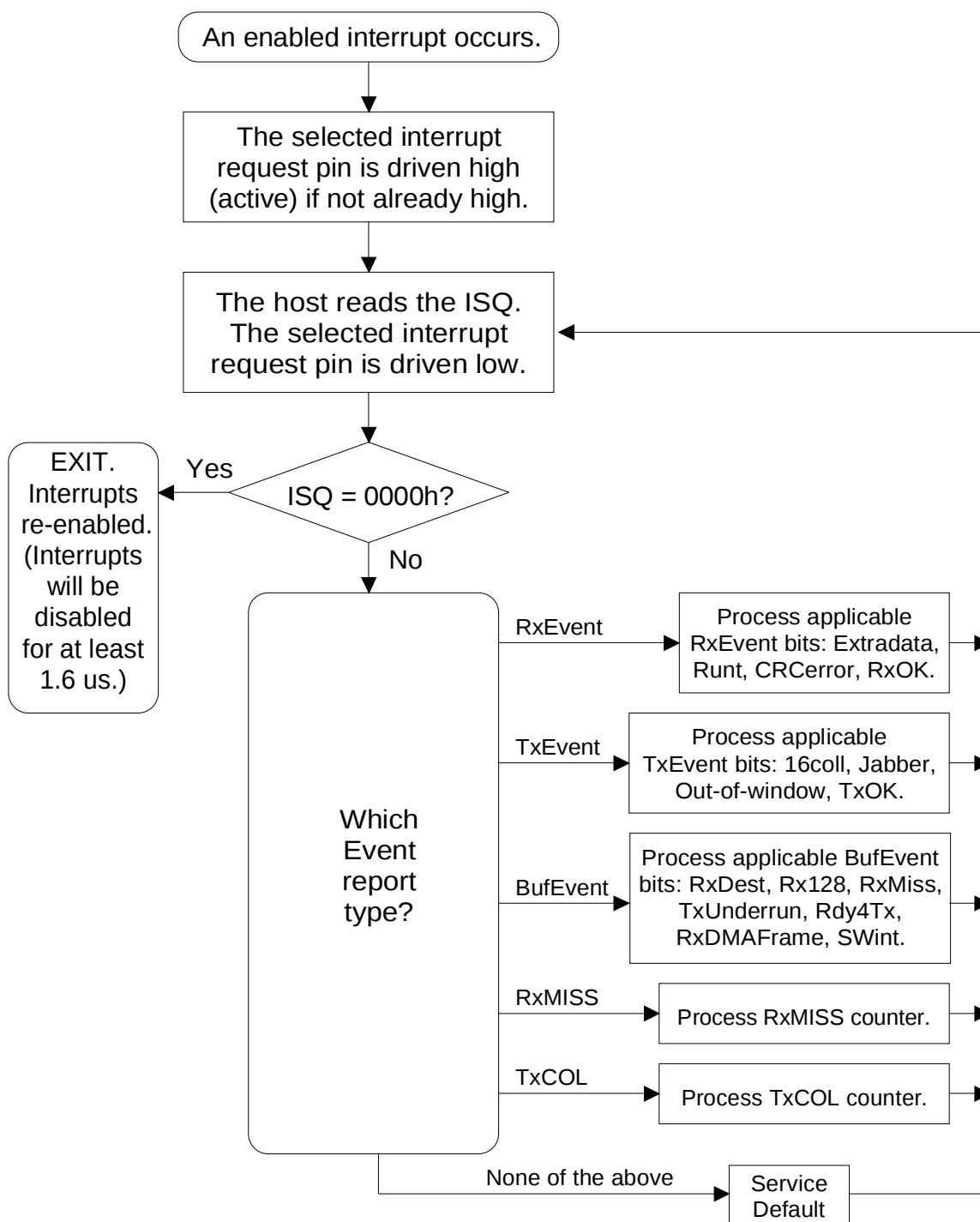
Figure 5.1. Interrupt Status Queue
