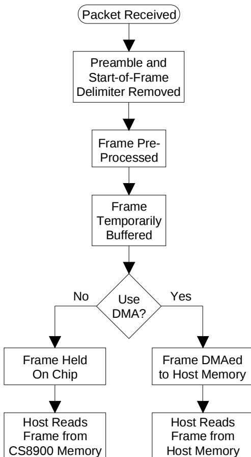
Figure 5.2. Frame Reception
