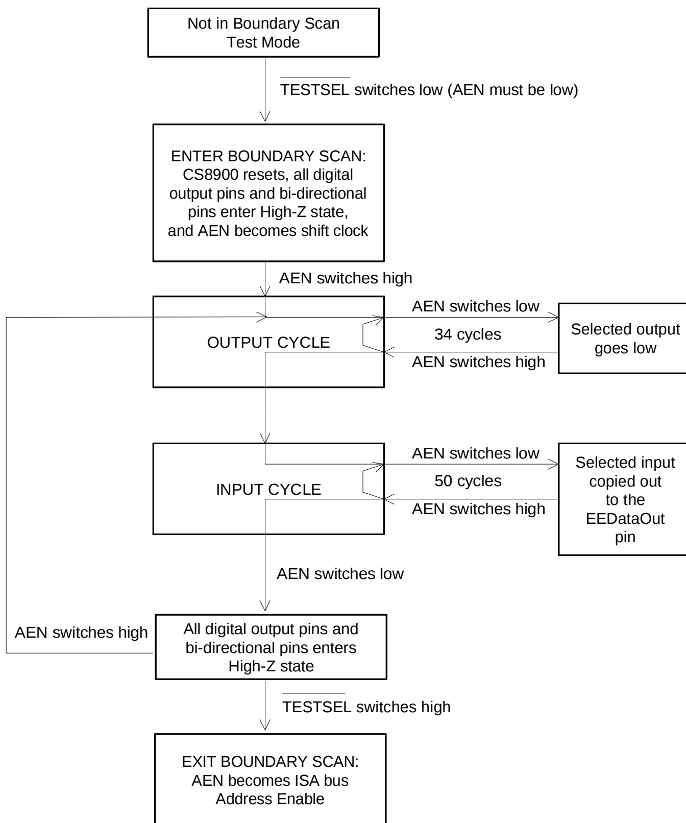
Figure 6.1. Boundary Scan Continuity Cycle
