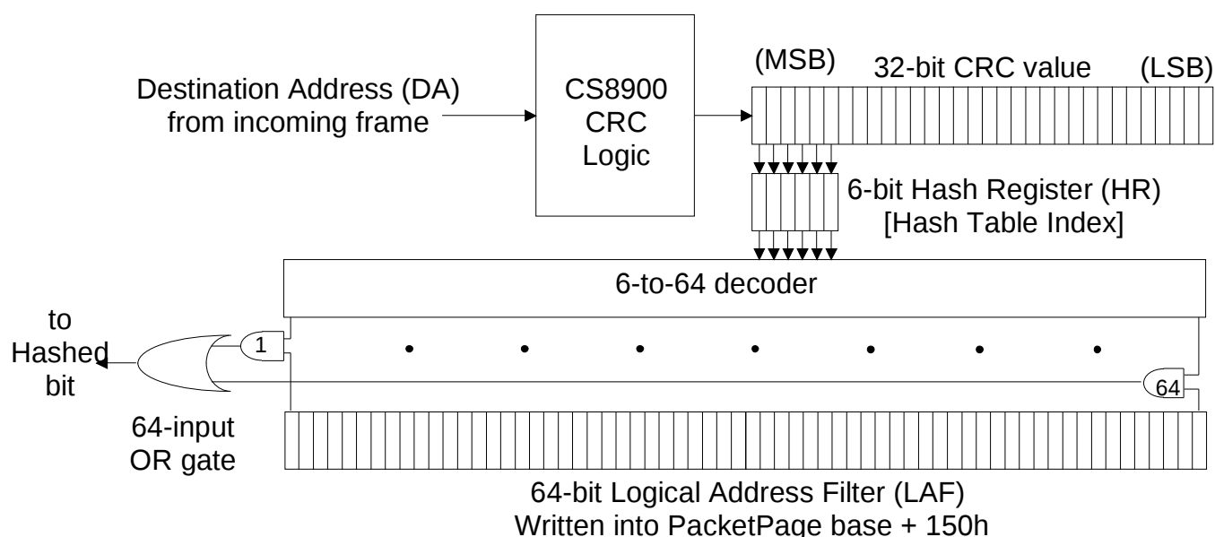
Figure 5.5. Hash Filter Operation
