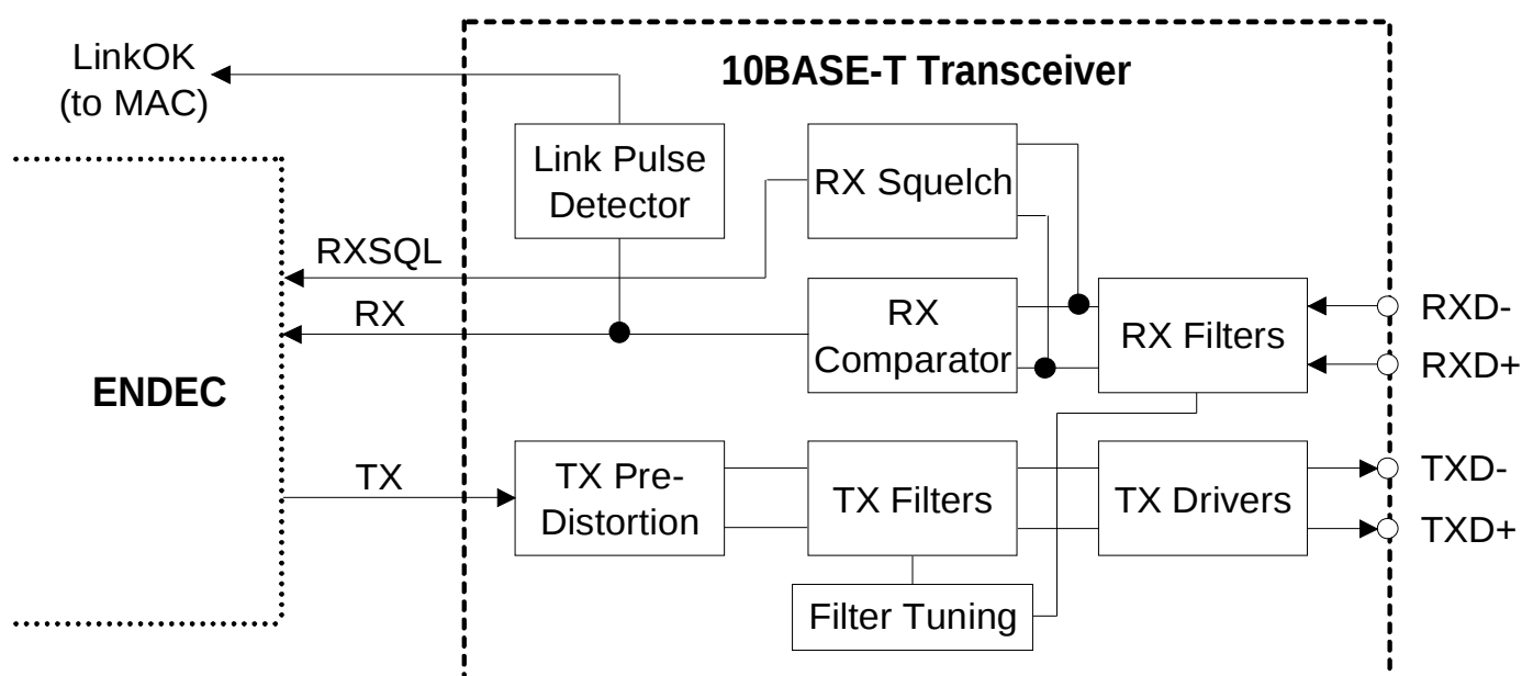
Figure 3.10. 10BASE-T Transceiver
