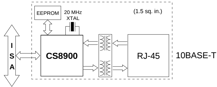
Figure 1.1. Complete Ethernet Motherboard Solution
