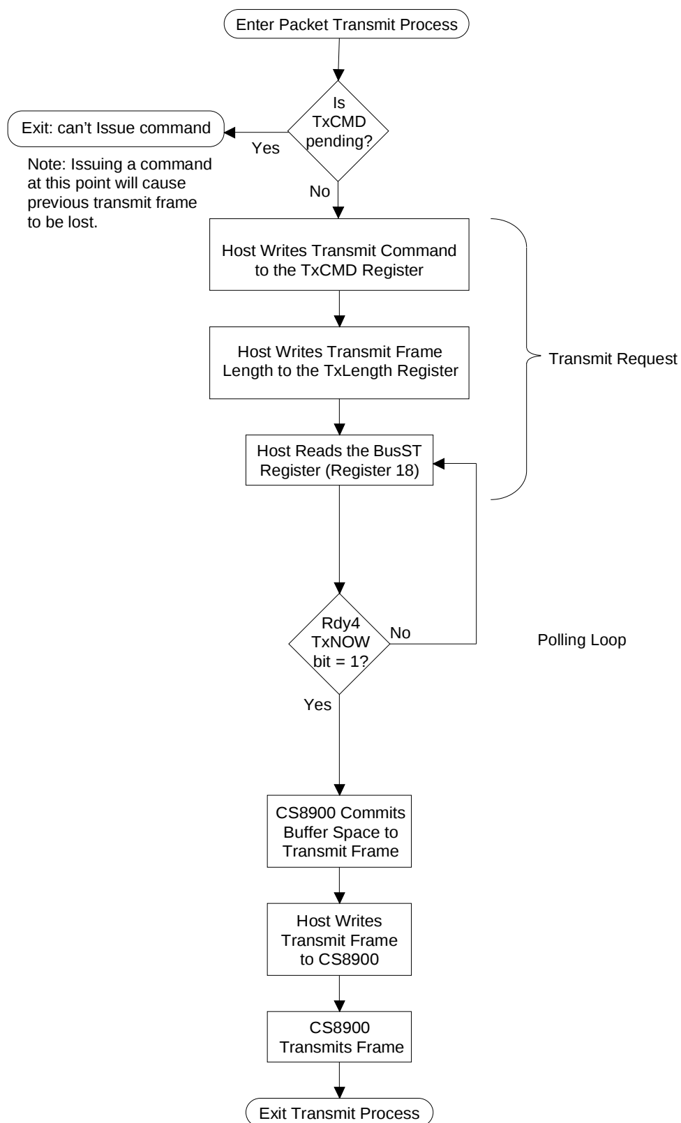
Figure 5.12. Transmit Operation in Polling Mode
