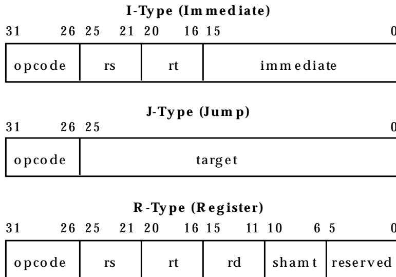
Figure 2. Instruction Formats
