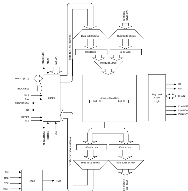
Figure 1: Block Diagram
