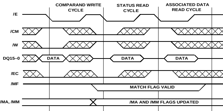
Figure 9: Cycle-to-Cycle Timing Example
