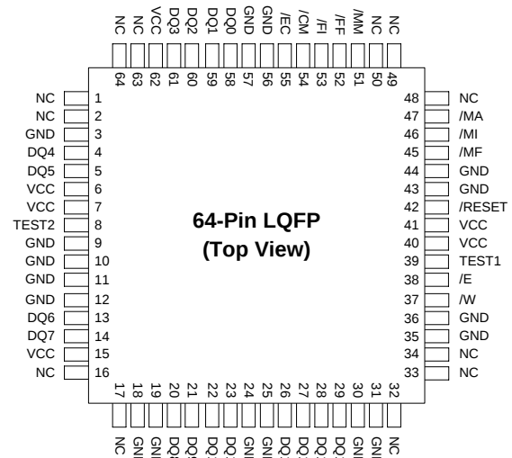
Figure 3: 64-Pin LQFP
