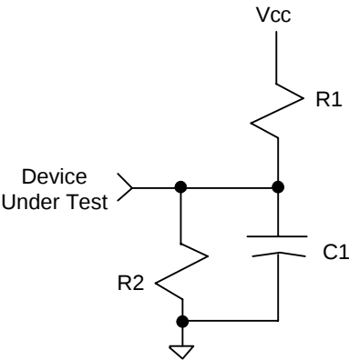
Figure 11: AC Test Load
