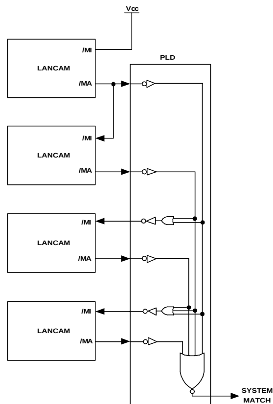
Figure 4: External Prioritizing
