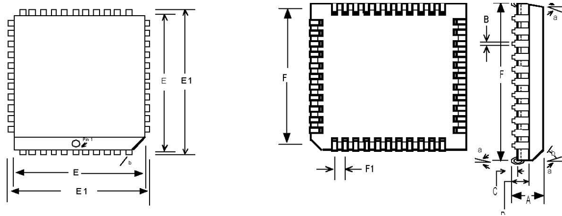
Figure 15: 44-Pin PLCCPackage
