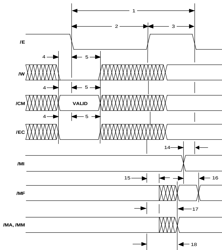
Figure 14: Compare Cycle
