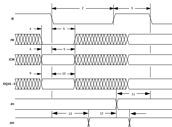
Figure 13: Write Cycle
