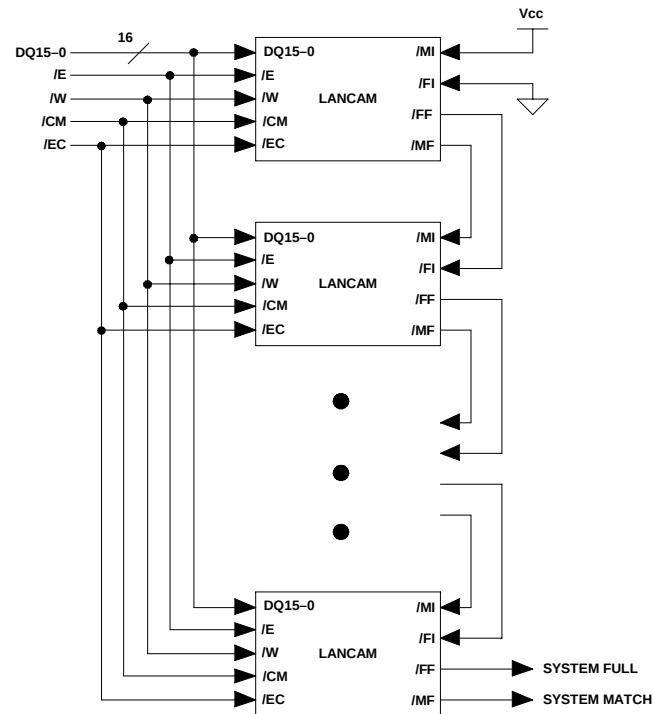
Figure 3: Vertical Cascading
