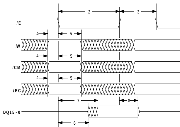
Figure 12: Read Cycle
