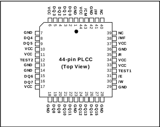
Pinout Diagram
