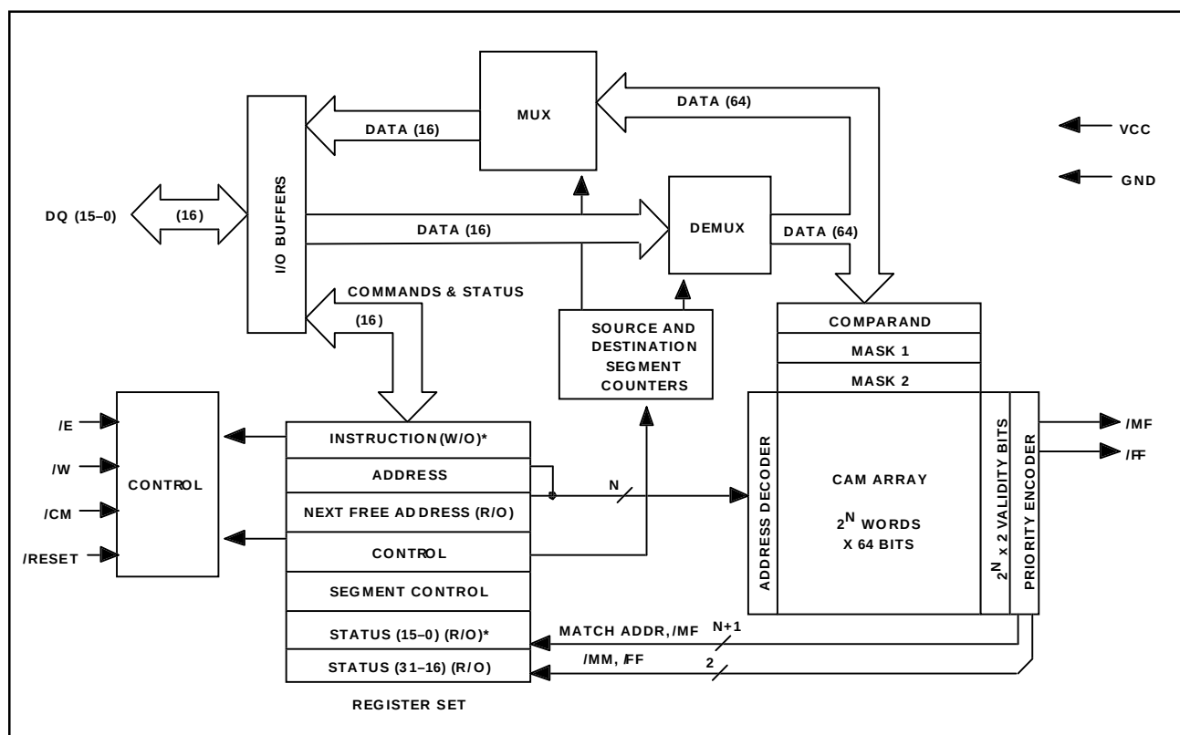
Block Diagram
