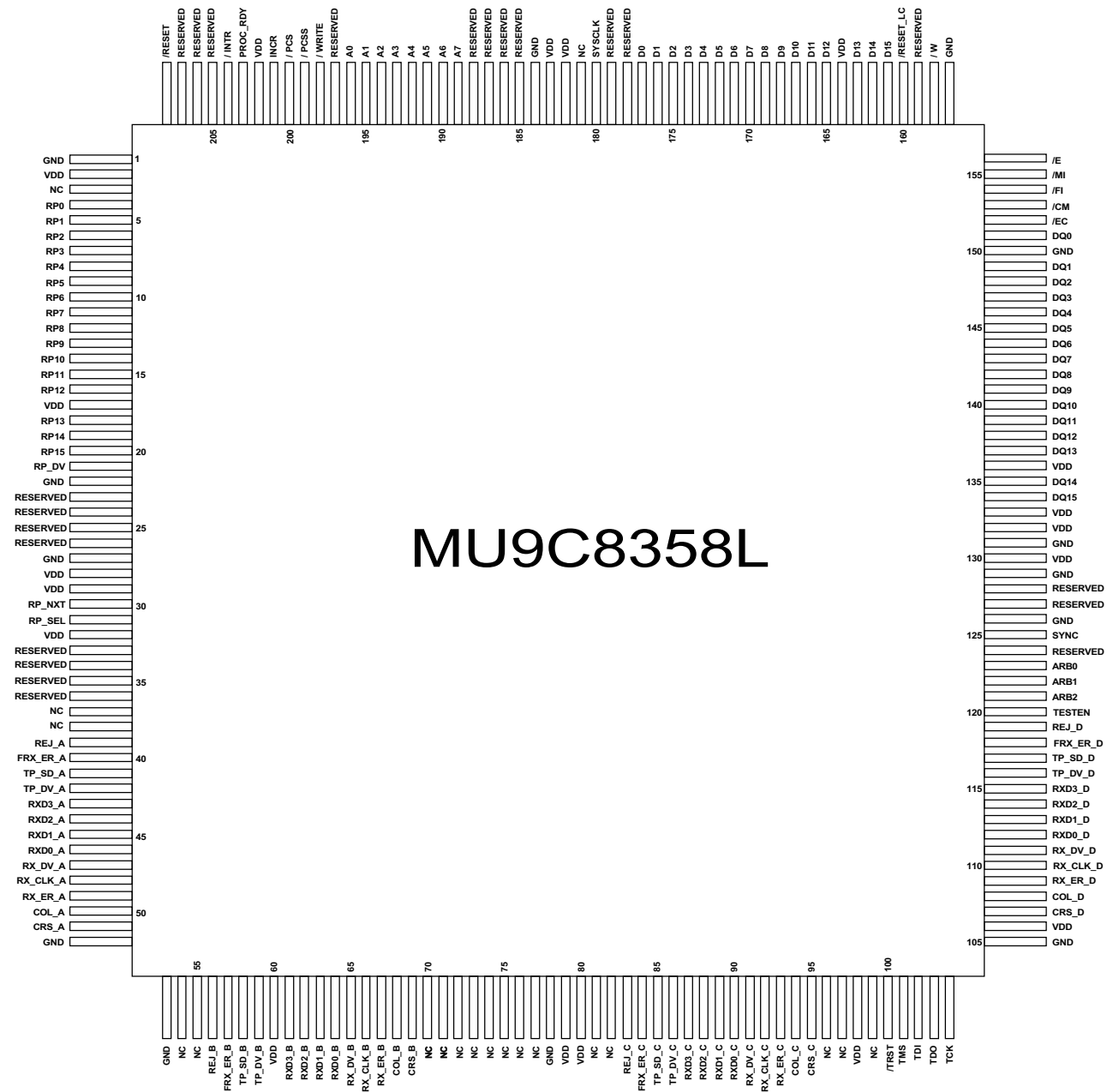
Figure 3: Pinout Diagram
