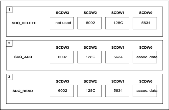
Figure 6: SCDW Register Order
