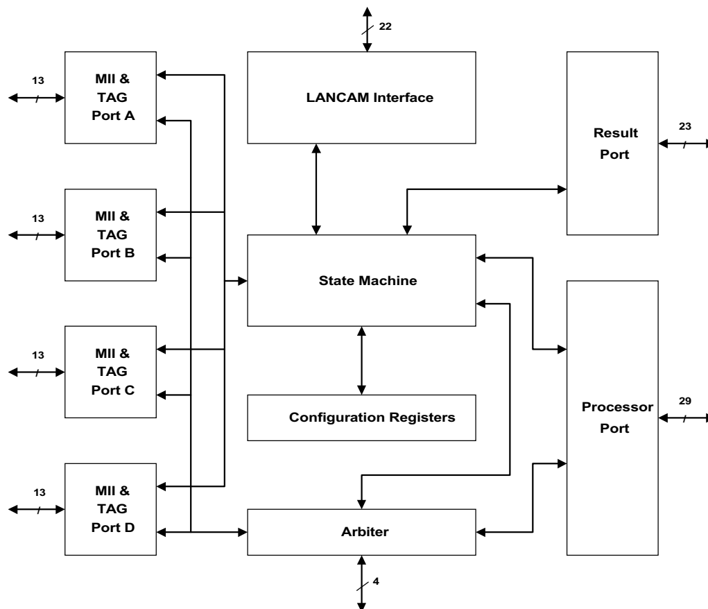
Figure 1: Block Diagram
