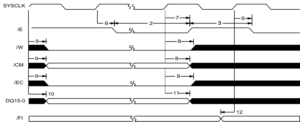
Figure 14: Timing Diagram for LANCAM - Write
