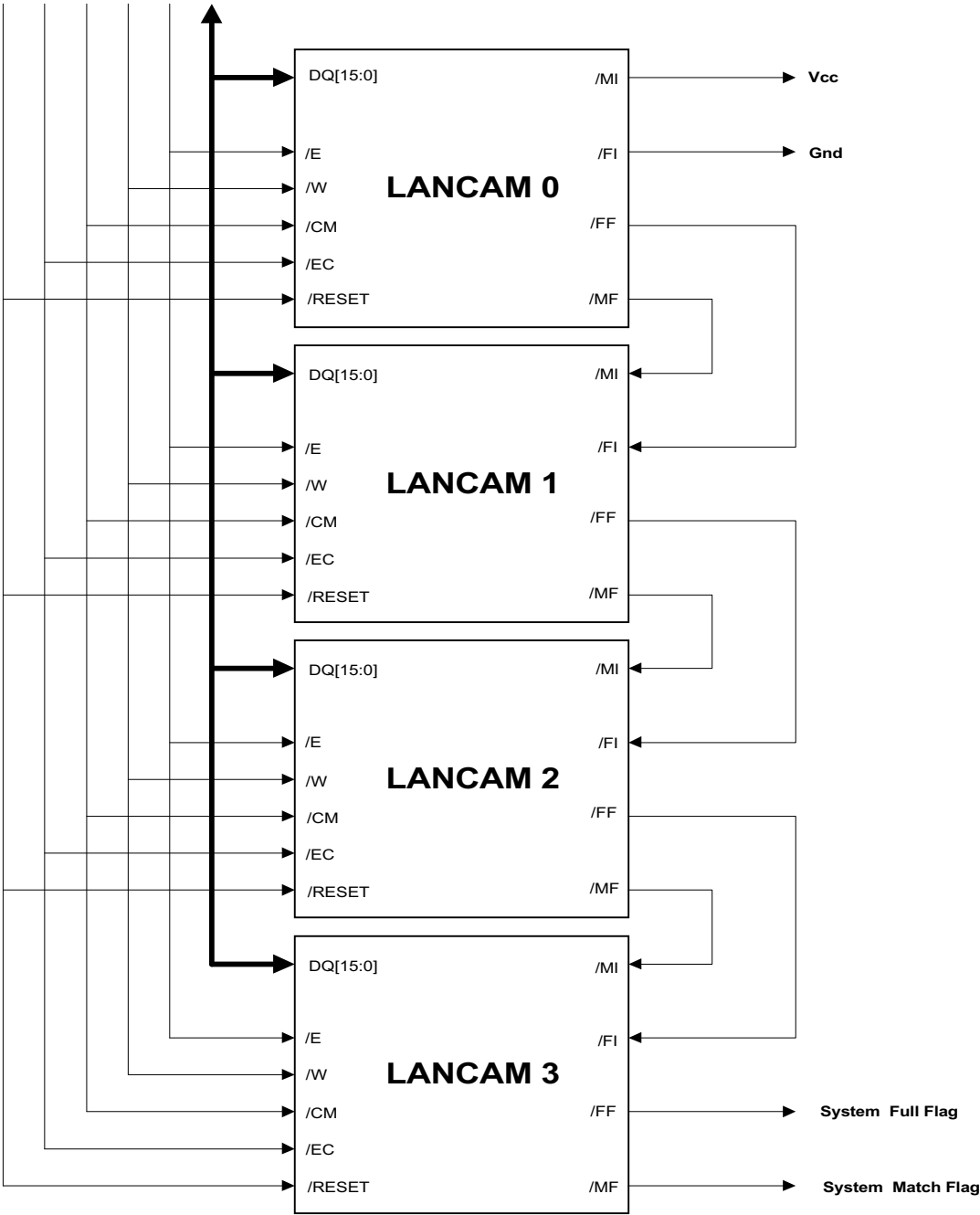
Figure 8: Cascading LANCAMs
