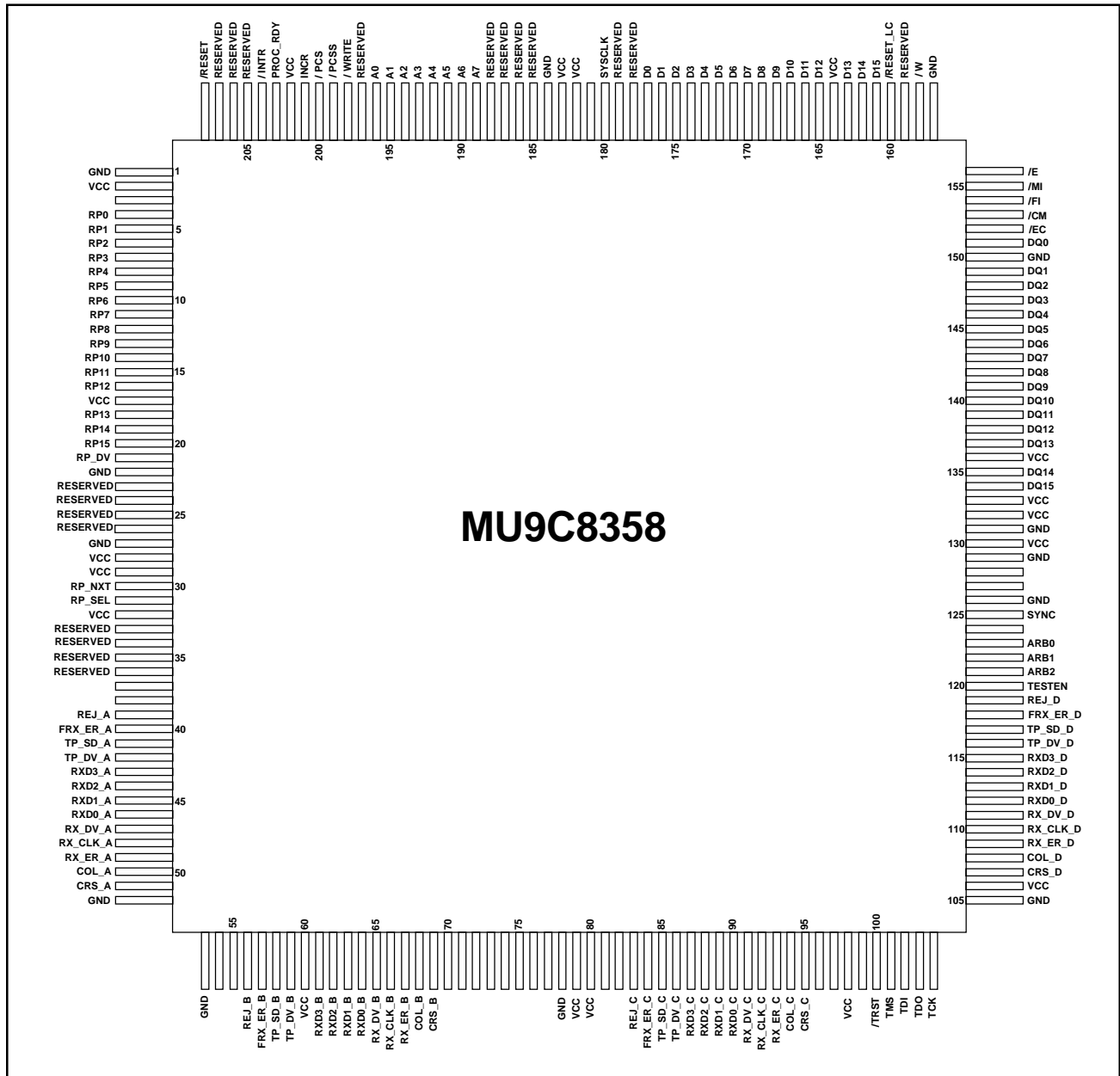
Pinout Diagram
