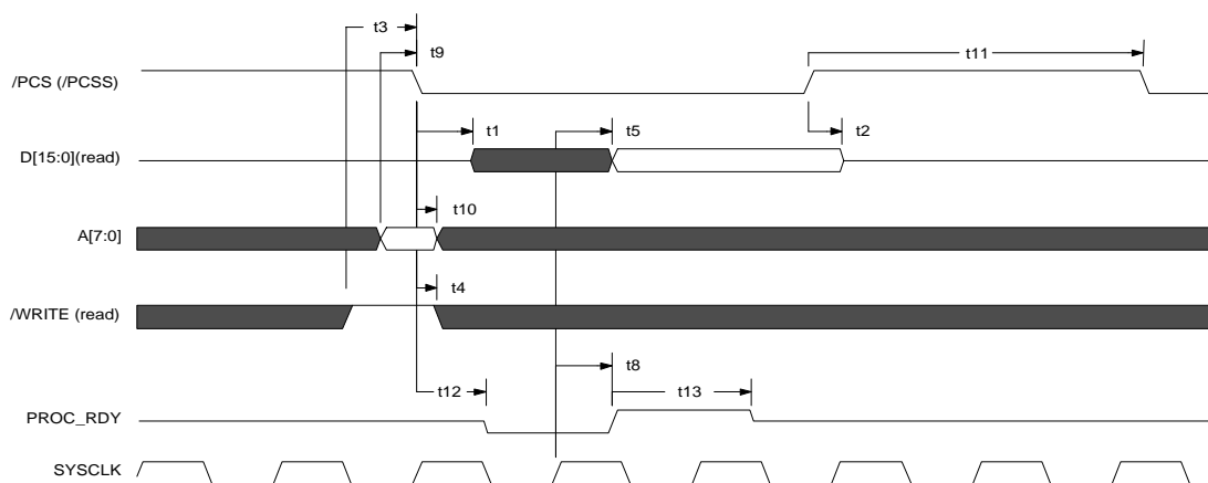
Figure 7: Host Processor Interface - Read Sequence
