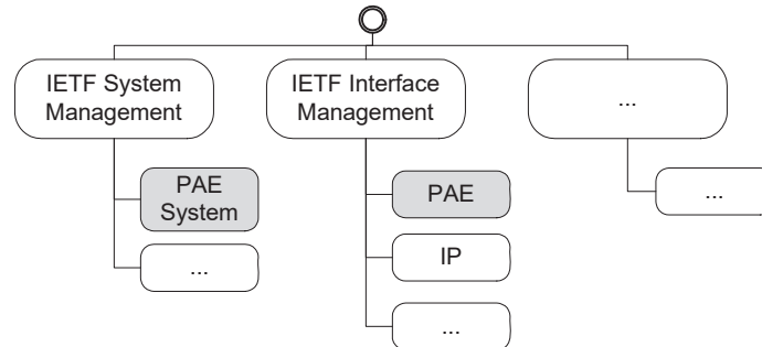
Figure 14-2—YANG object hierarchy with IEEE Std 802.1X
