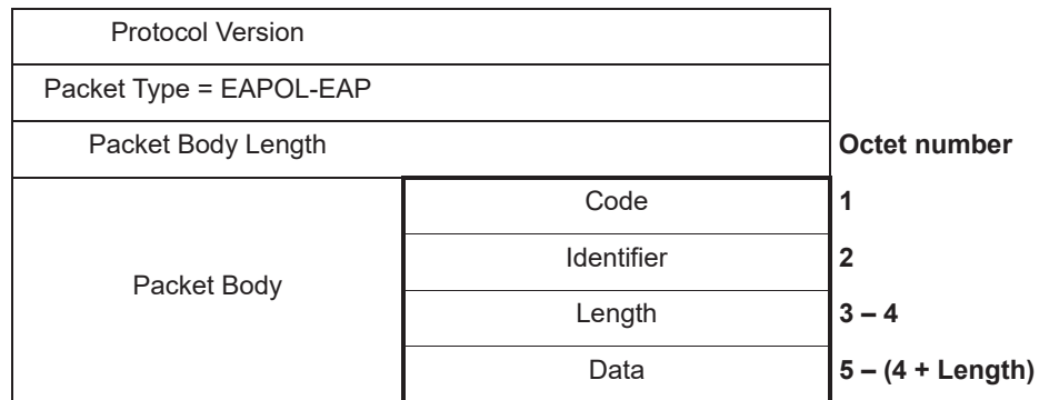
Figure 11-4—EAPOL-EAP Packet Body with EAP packet format
