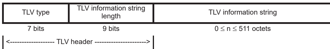
Figure 11-19—EAPOL-Announcement TLV format
