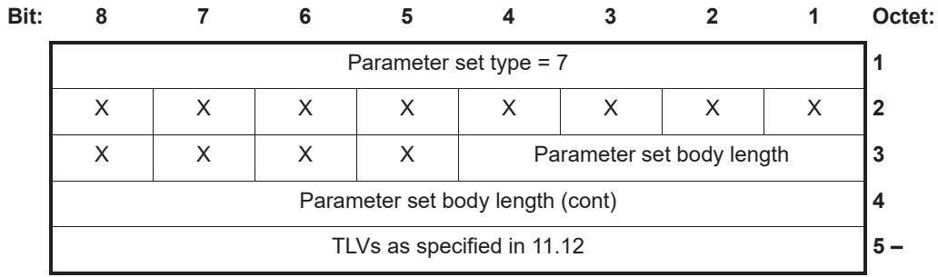
Figure 11-15—Announcement parameter set
