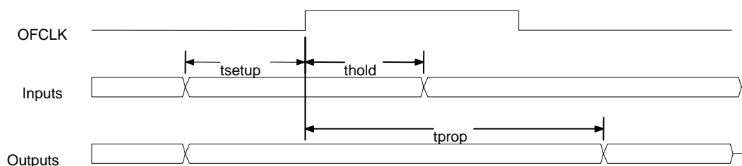
Figure 51 Ingress Output Cell Interface Timing
