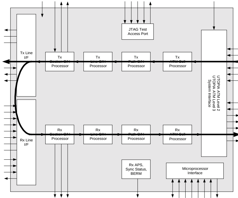
Figure 18: Parallel Diagnostic Loopback Mode
