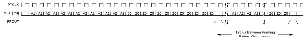
Figure 30: Parallel Transmit Interface Timing
