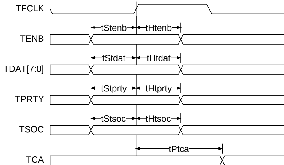
Figure 43: Transmit UTOPIA Level 3 System Interface Timing Diagram
